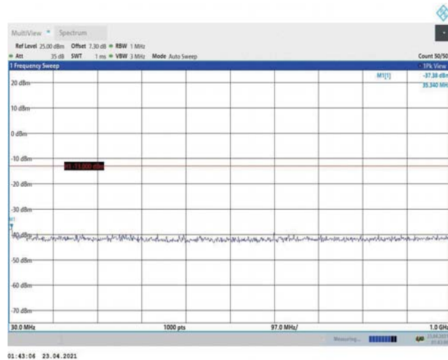
Band2-1.4MHz-16QAM-19193-1RB#0-Range1:30~1000MHz
