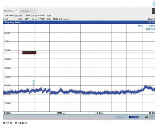
Band2-5MHz-16QAM-18625-1RB#0-Range3:2000~20000MHz
