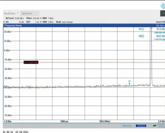
Band2-1.4MHz-16QAM-19193-1RB#0-Range2:1000~2000MHz
