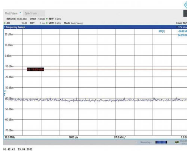
Band2-1.4MHz-QPSK-19193-1RB#0-Range1:30~1000MHz
