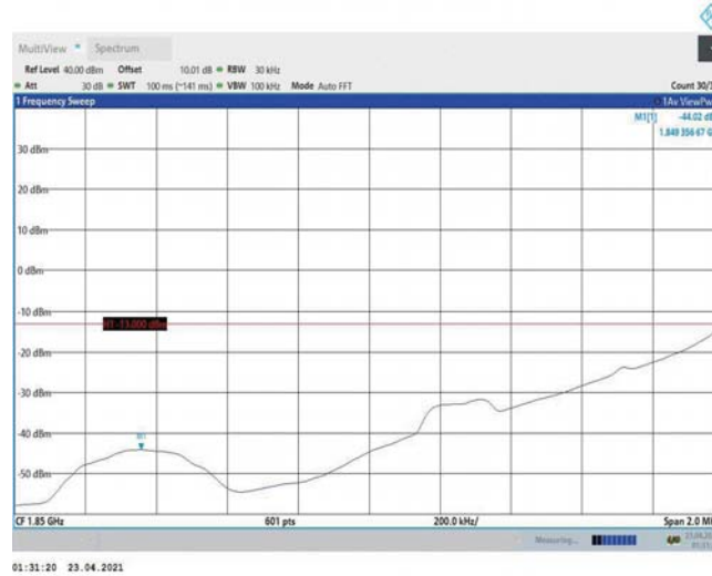
Band2-1.4MHz-16QAM-18607-1RB#5
