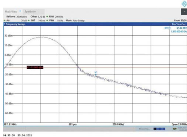
Band2-10MHz-16QAM-19150-1RB#49
