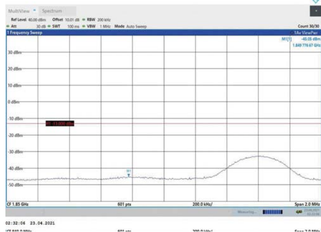
Band2-10MHz-QPSK-18650-1RB#49
