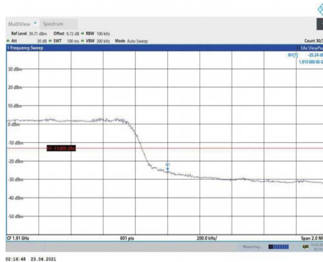
Band2-5MHz-16QAM-19175-25RB#0
