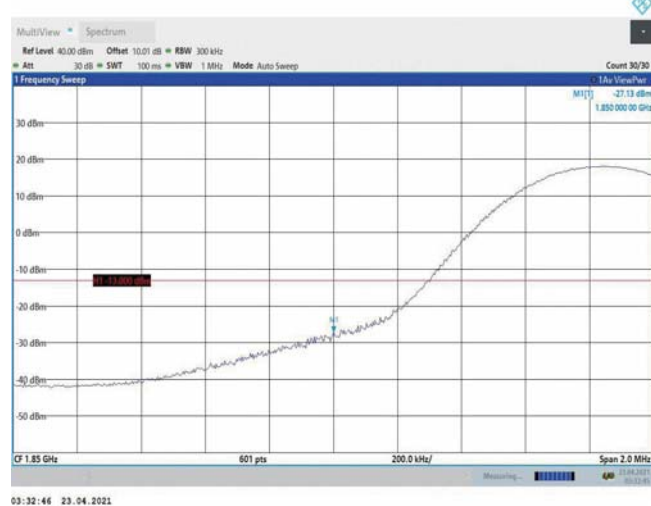
Band2-15MHz-QPSK-18675-1RB#0
