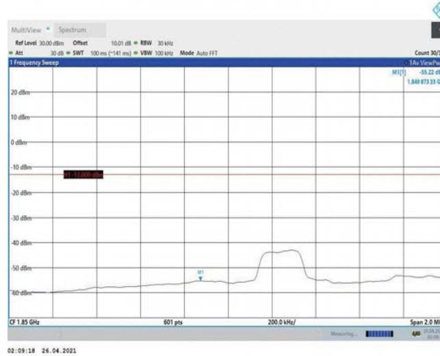
Band2-3MHz-16QAM-18615-1RB#14
