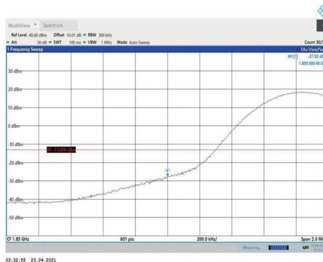
Band2-15MHz-16QAM-18675-1RB#0
