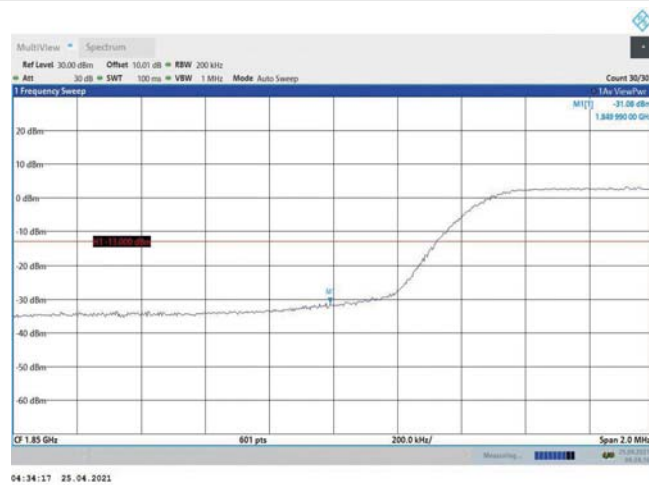
Band2-10MHz-16QAM-18650-50RB#0
