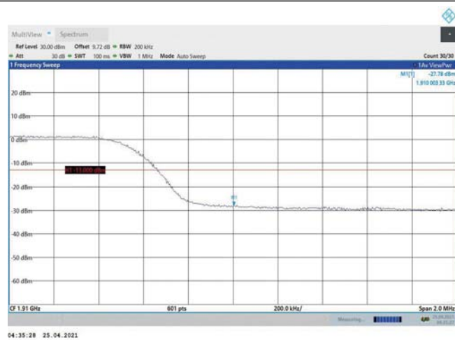
Band2-10MHz-16QAM-19150-50RB#0
