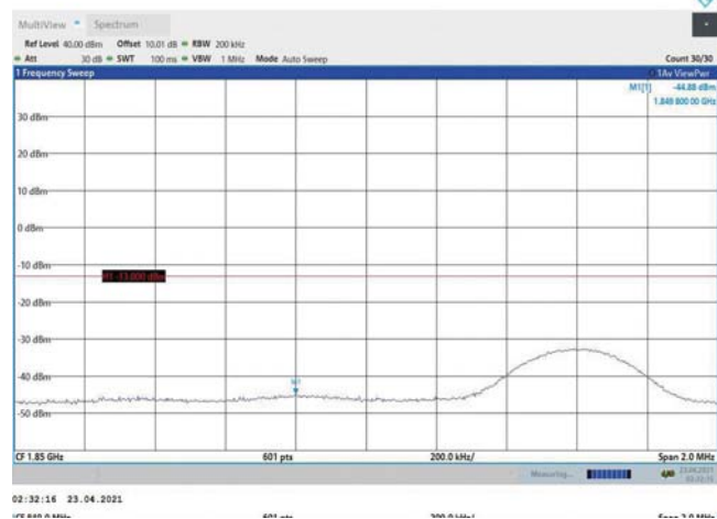
Band2-10MHz-16QAM-18650-1RB#49
