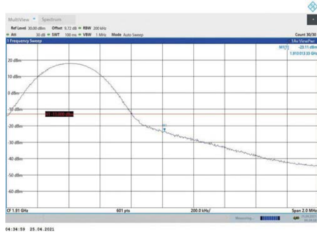
Band2-10MHz-QPSK-19150-1RB#49
