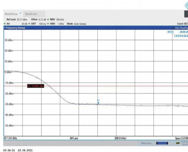
Band2-15MHz-16QAM-19125-75RB#0
