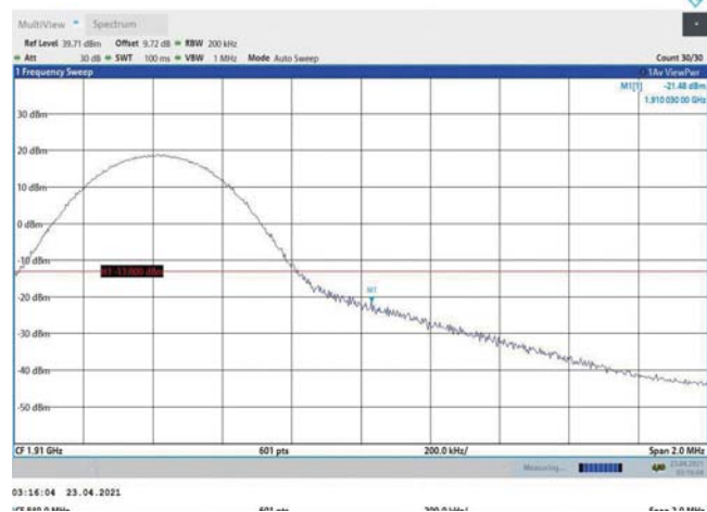
Band2-10MHz-16QAM-19150-1RB#49
