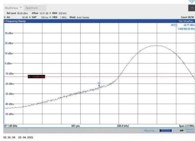
Band2-10MHz-16QAM-18650-1RB#0
