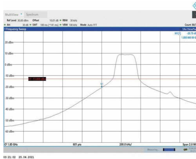
Band2-1.4MHz-16QAM-18607-1RB#0
