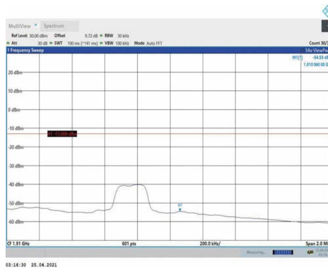
Band2-3MHz-16QAM-19185-1RB#0
