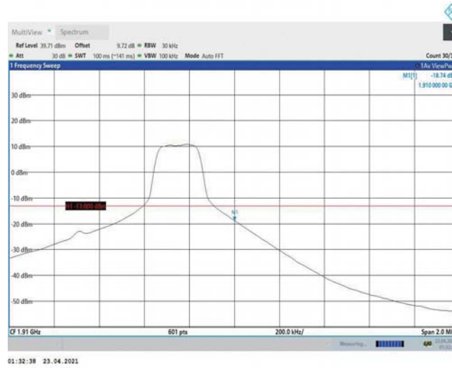
Band2-1.4MHz-16QAM-19193-1RB#5
