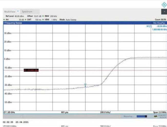
Band2-10MHz-16QAM-18650-50RB#0
