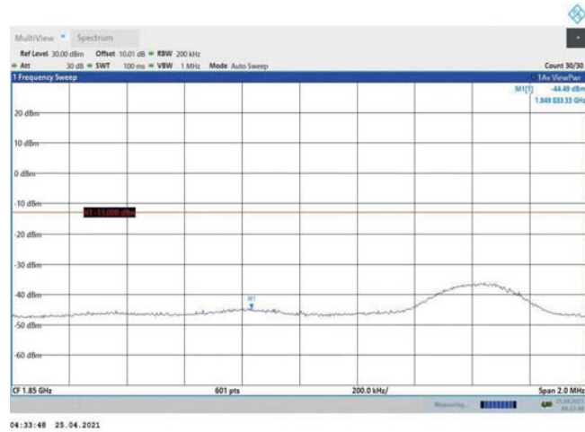
Band2-10MHz-QPSK-18650-1RB#49
