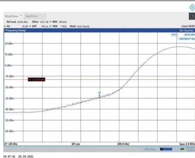
Band2-15MHz-QPSK-18675-1RB#0
