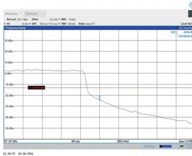
Band2-1.4MHz-16QAM-19193-6RB#0
