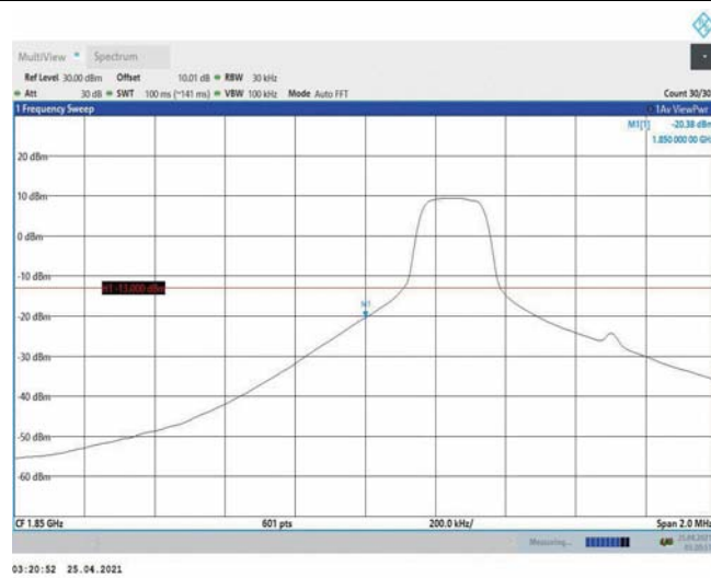
Band2-1.4MHz-QPSK-18607-1RB#0
