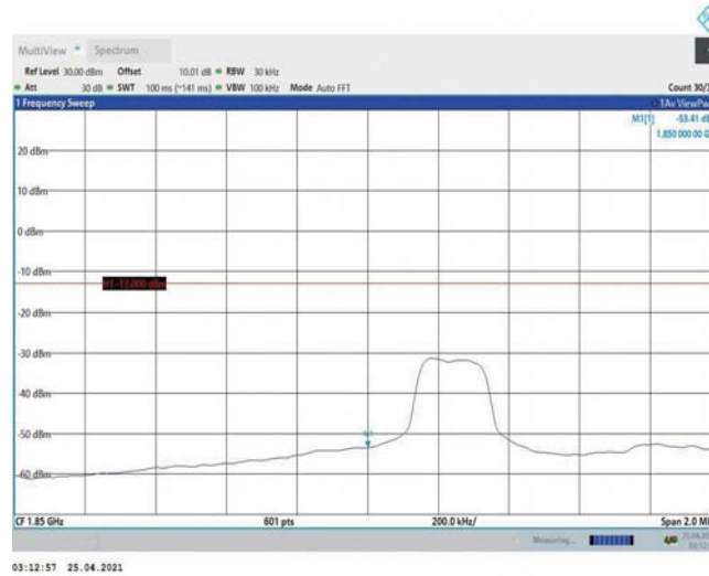
Band2-3MHz-16QAM-18615-1RB#14
