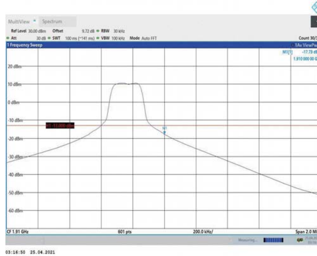
Band2-3MHz-16QAM-19185-1RB#14
