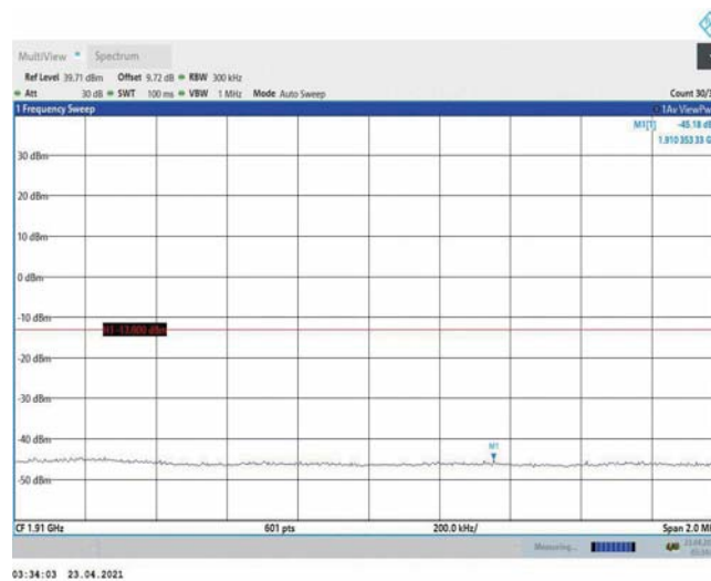
Band2-15MHz-QPSK-19125-1RB#0
