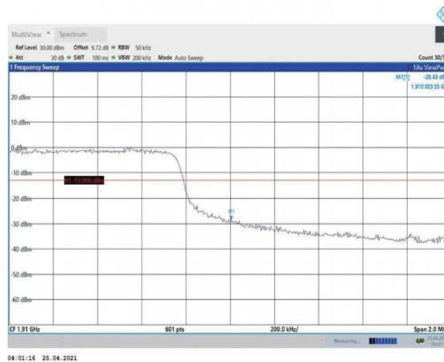
Band2-5MHz-QPSK-19175-25RB#0
