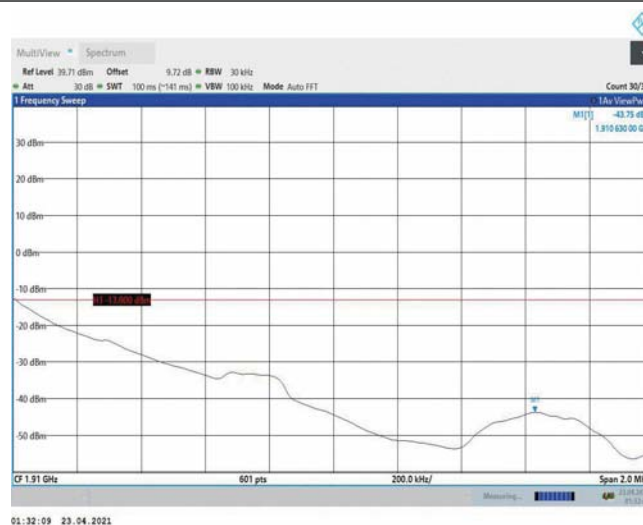
Band2-1.4MHz-QPSK-19193-1RB#0
