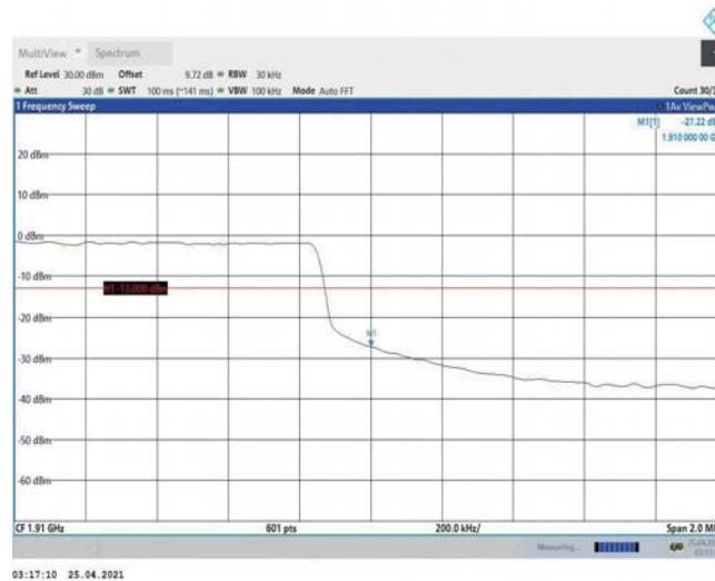
Band2-3MHz-16QAM-19185-15RB#0
