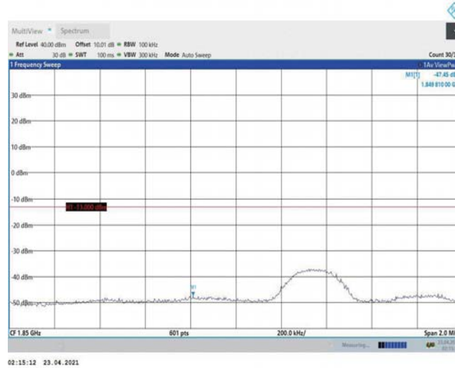
Band2-5MHz-16QAM-18625-1RB#24
