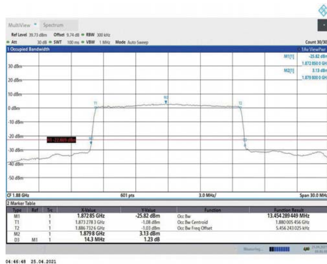
Band2-15MHz-QPSK-18900-75RB#0-13.454
