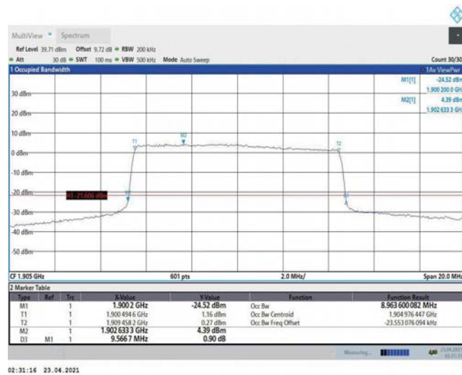
Band2-10MHz-QPSK-19150-50RB#0-8.964
