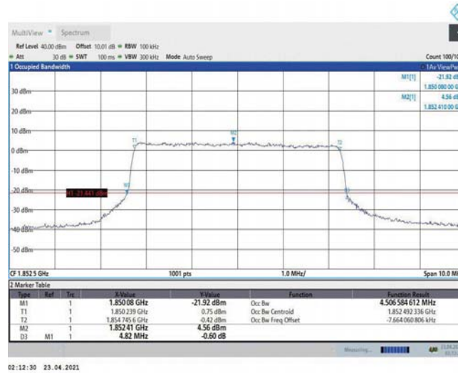
Band2-5MHz-QPSK-18625-25RB#0-4.507
