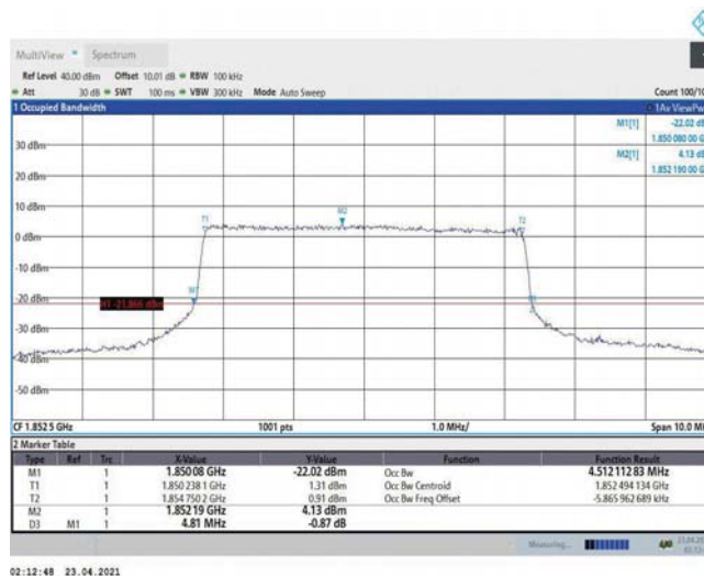
Band2-5MHz-16QAM-18625-25RB#0-4.512
