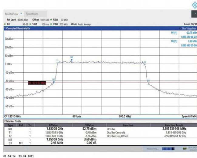
Band2-3MHz-16QAM-18615-15RB#0-2.696
