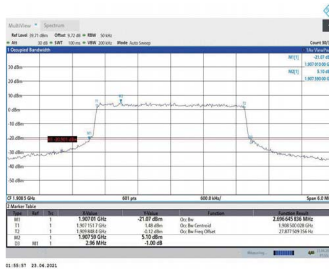
Band2-3MHz-16QAM-19185-15RB#0-2.697
