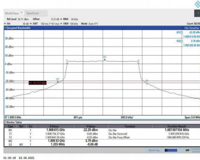
Band2-1.4MHz-16QAM-19193-6RB#0-1.087
