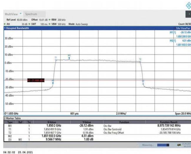
Band2-10MHz-16QAM-18650-50RB#0-8.976
