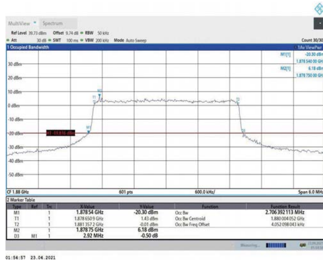
Band2-3MHz-QPSK-18900-15RB#0-2.706
