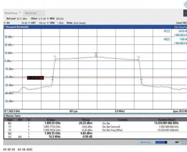
Band2-15MHz-QPSK-19125-75RB#0-13.417
