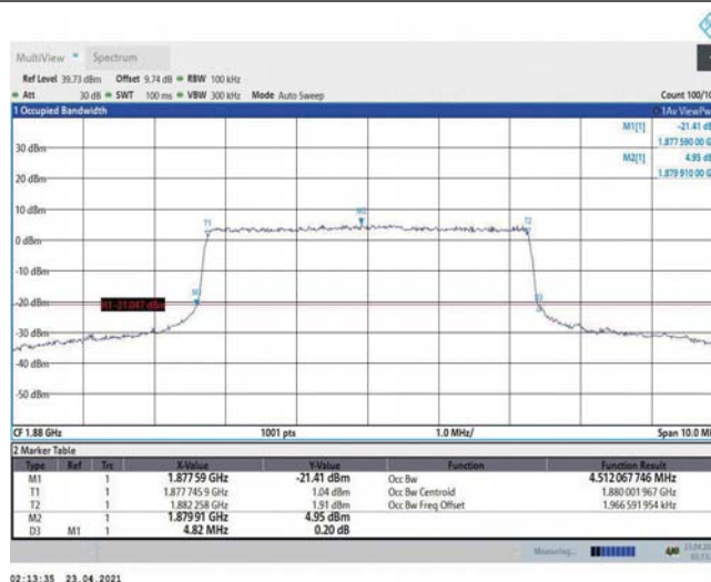
Band2-5MHz-16QAM-18900-25RB#0-4.512
