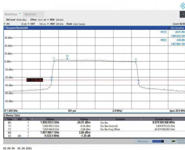
Band2-10MHz-16QAM-18650-50RB#0-8.975
