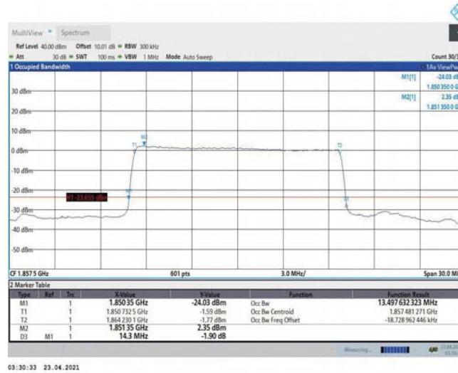
Band2-15MHz-16QAM-18675-75RB#0-13.498
