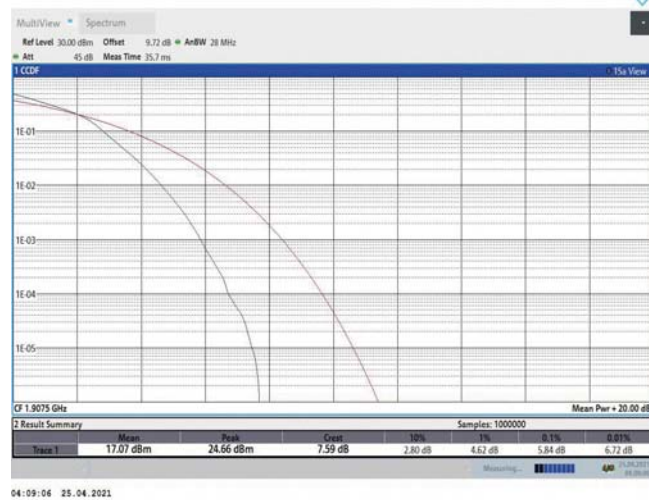
Band2-5MHz-16QAM-19175-25RB#0
