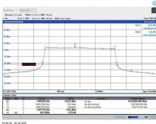
Band2-5MHz-16QAM-19175-25RB#0-4.518
