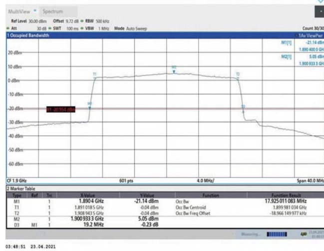
Band2-20MHz-16QAM-19100-100RB#0-17.925
