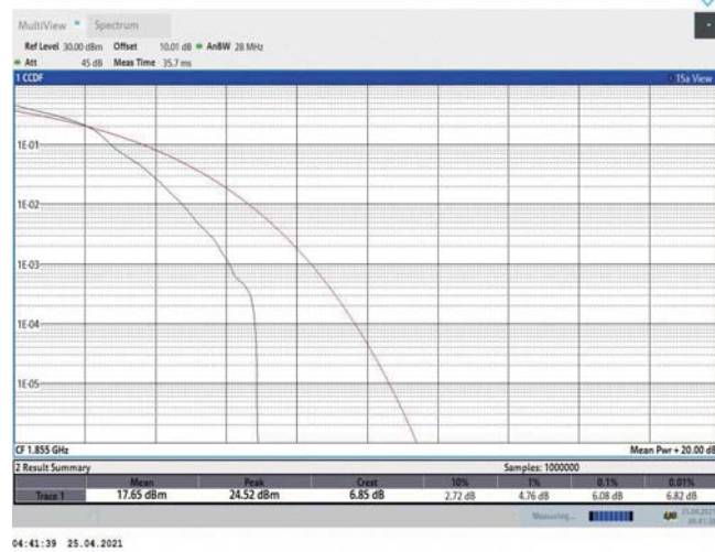
Band2-10MHz-16QAM-18650-1RB#0
