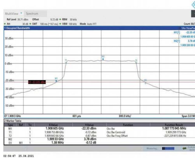
Band2-1.4MHz-16QAM-19193-6RB#0-1.088
