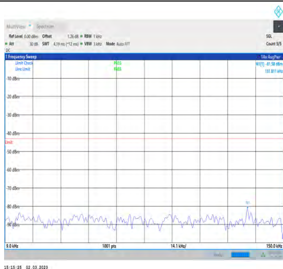
1-N78-3700-3800-PC2-30-100-L-1-DFT-QPSK-Edge e_1RB_Left-1@0-0.009-0.15-Ant1-0.13--81.58--43- PASS
