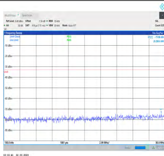
1-N78-3700-3800-PC2-30-100-L-1-DFT-QPSK-Edge _1RB_Left-1@0-0.15-30-Ant1-23.88--73.88--33-PAS S
