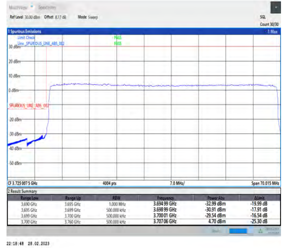
1-N78-3700-3800-30-60-L-3-DFT-PI2BPSK-Outer _Full-162@0-Ant1-1--PASS-see graph
