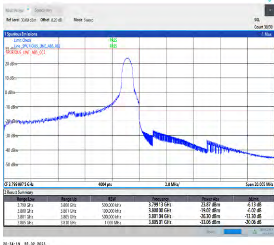
1-N78-3700-3800-PC2-30-10-H-5-CP-QPSK-Edge_1R B_Right-1@23-Ant1-1--PASS-see graph
