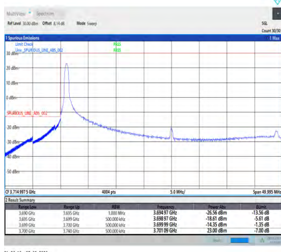
1-N78-3700-3800-30-40-L-4-CP-QPSK-Edge_1RB_Lef t-1@0-Ant1-1--PASS-see graph
