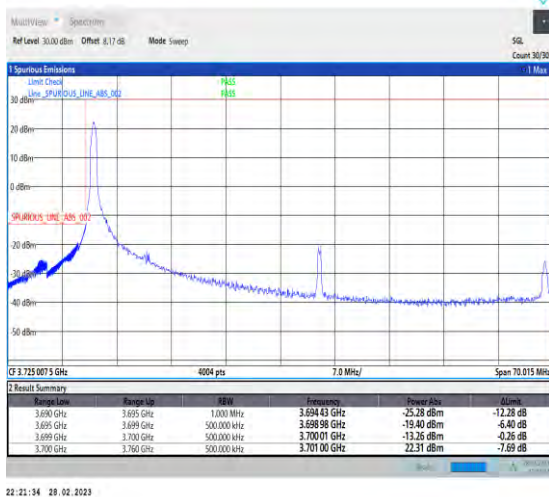
1-N78-3700-3800-30-60-L-4-CP-QPSK-Edge_1RB_Lef t-1@0-Ant1-1--PASS-see graph
