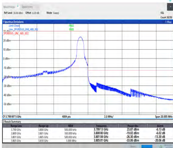
1-N78-3700-3800-30-10-H-2-DFT-PI2BPSK-Edge_1R_B_Right-1@23-Ant1-1--PASS-see graph
