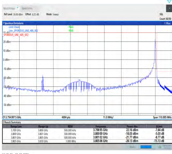
1-N78-3700-3800-PC2-30-100-H-5-CP-QPSK-Edge_1 RB_Right-1@272-Ant1-1--PASS-see graph
