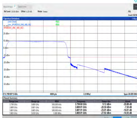
1-N78-3700-3800-30-10-H-6-CP-QPSK-Outer_Full-24@0-Ant1-1--PASS-see graph
