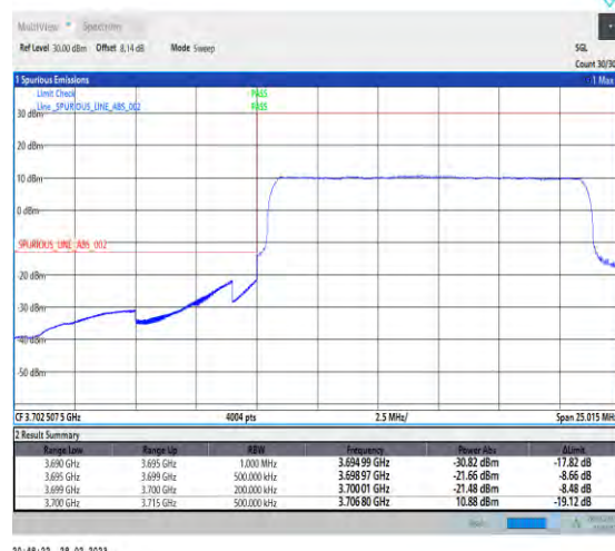
1-N78-3700-3800-30-15-L-3-DFT-PI2BPSK-Outer _Full-36@0-Ant1-1--PASS-see graph
