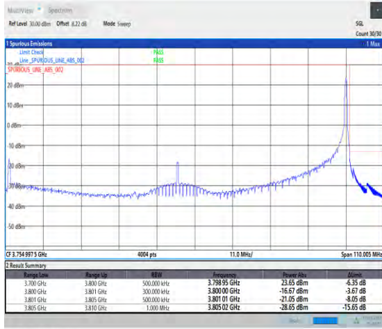
1-N78-3700-3800-30-100-H-2-DFT-PI2BPSK-Edge_1R_B_Right-1@272-Ant1-1--PASS-see graph
