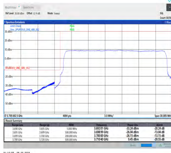
1-N78-3700-3800-30-20-L-3-DFT-PI2BPSK-Outer _Full-50@0-Ant1-1--PASS-see graph
