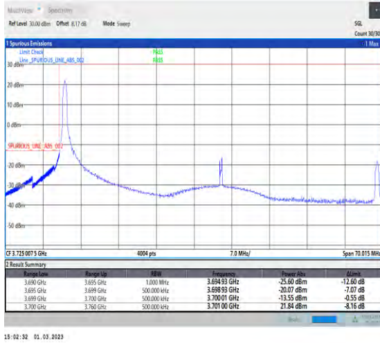
1-N78-3700-3800-30-60-L-1-DFT-PI2BPSK-Edge_1RB _Left-1@0-Ant1-1--PASS-see graph
