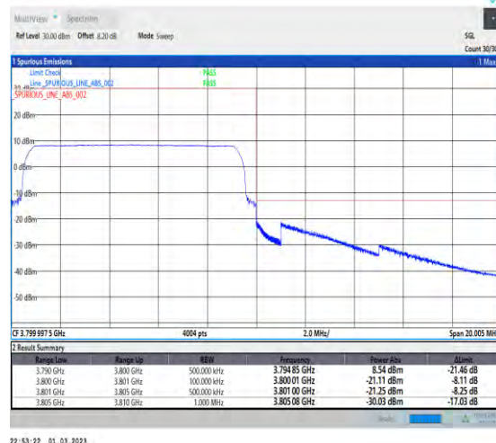
1-N78-3700-3800-PC2-30-10-H-6-CP-QPSK-Outer _Full-24@0-Ant1-1--PASS-see graph
