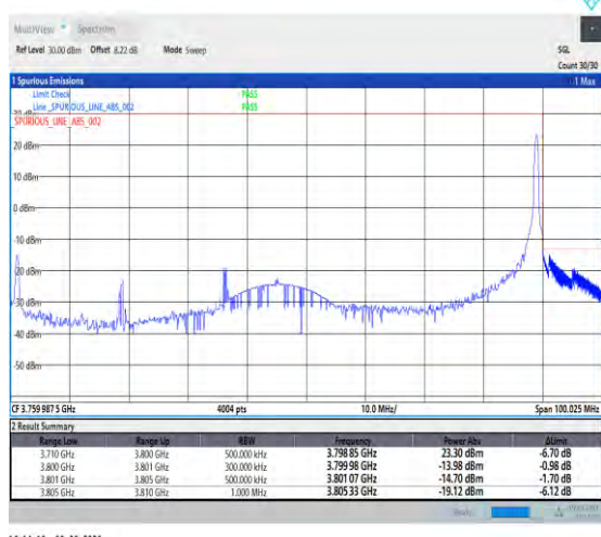
1-N78-3700-3800-PC2-30-90-H-5-CP-QPSK-Edge_1R B_Right-1@244-Ant1-1--PASS-see graph
