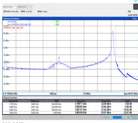
1-N78-3700-3800-PC2-30-50-H-5-CP-QPSK-Edge_1R B_Right-1@132-Ant1-1--PASS-see graph
