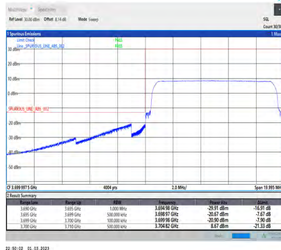
1-N78-3700-3800-PC2-30-10-L-6-CP-QPSK-Outer _Full-24@0-Ant1-1--PASS-see graph
