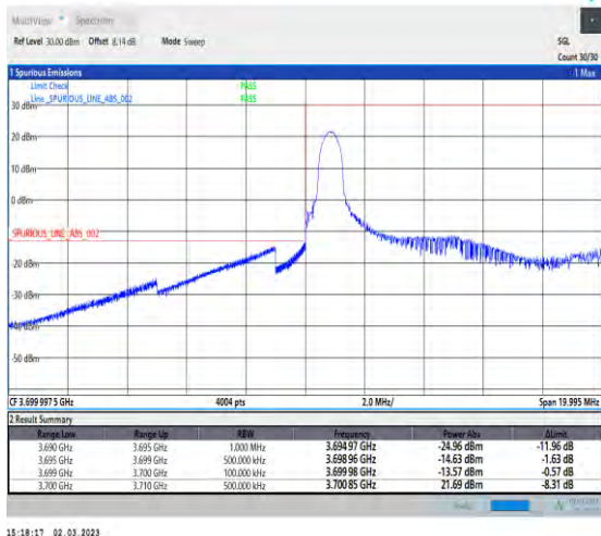
1-N78-3700-3800-PC2-30-10-L-4-CP-QPSK-Edge_1R B_Left-1@0-Ant1-1--PASS-see graph
