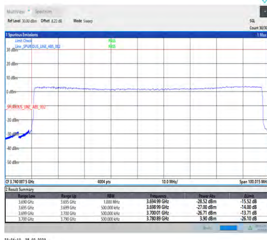
1-N78-3700-3800-30-90-L-3-DFT-PI2BPSK-Outer_Full-240@0-Ant1-1--PASS-see graph
