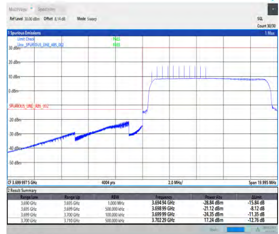
1-N78-3700-3800-30-10-L-6-CP-QPSK-Outer_Full -24@0-Ant1-1--PASS-see graph
