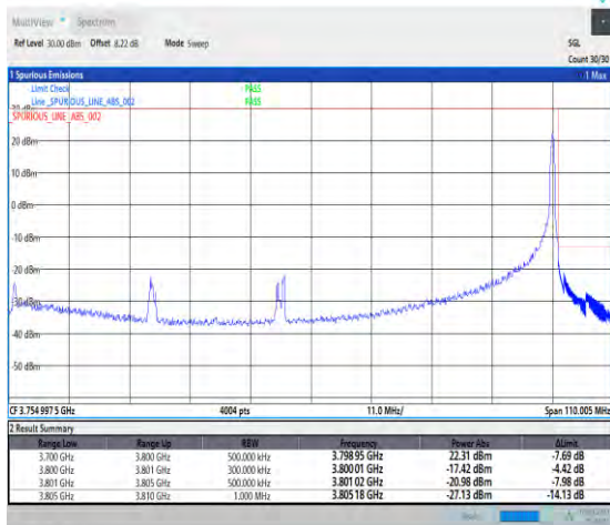
1-N78-3700-3800-30-100-H-5-CP-QPSK-Edge_1RB_Right-1@272-Ant1-1--PASS-see graph
