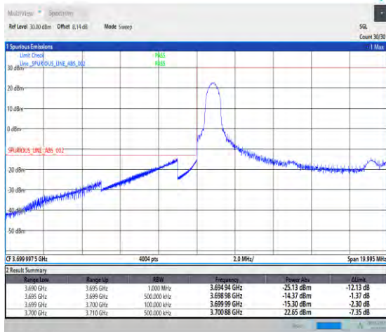
1-N78-3700-3800-30-10-L-4-CP-QPSK-Edge_1RB_Lef t-1@0-Ant1-1--PASS-see graph
