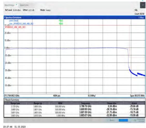
1-N78-3700-3800-PC2-30-80-H-6-CP-QPSK-Outer _Full-217@0-Ant1-1--PASS-see graph
