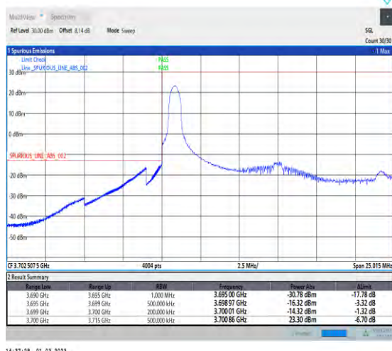
1-N78-3700-3800-30-15-L-1-DFT-PI2BPSK-Edge_1RB _Left-1@0-Ant1-1--PASS-see graph
