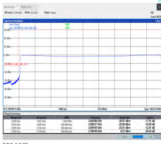
1-N78-3700-3800-PC2-30-90-L-6-CP-QPSK-Outer _Full-245@0-Ant1-1--PASS-see graph
