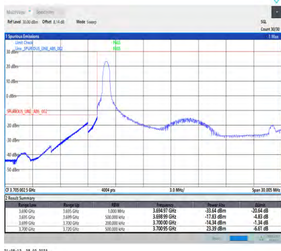
1-N78-3700-3800-30-20-L-1-DFT-PI2BPSK-Edge_1RB _Left-1@0-Ant1-1--PASS-see graph
