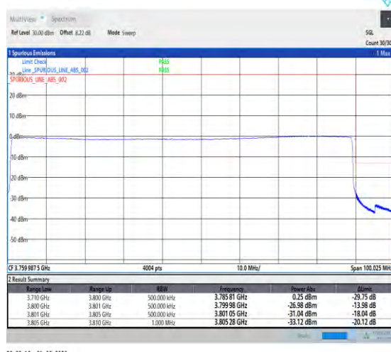
1-N78-3700-3800-PC2-30-90-H-6-CP-QPSK-Outer _Full-245@0-Ant1-1--PASS-see graph
