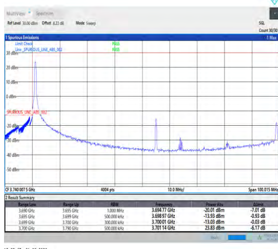
1-N78-3700-3800-30-90-L-4-CP-QPSK-Edge_1RB_Lef t-1@0-Ant1-1--PASS-see graph
