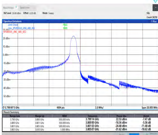
1-N78-3700-3800-30-10-H-5-CP-QPSK-Edge_1RB_Right-1@23-Ant1-1--PASS-see graph
