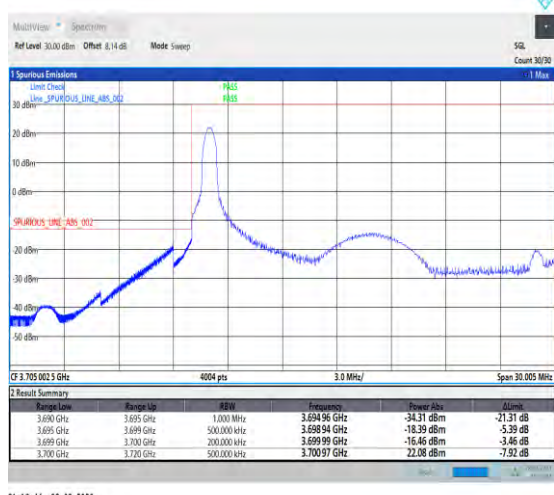
1-N78-3700-3800-30-20-L-4-CP-QPSK-Edge_1RB_Lef t-1@0-Ant1-1--PASS-see graph
