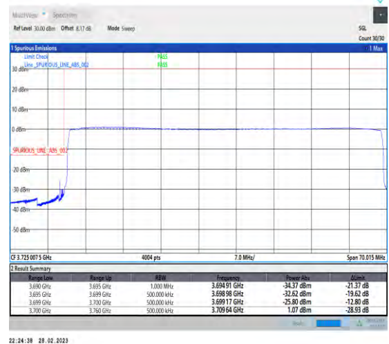
1-N78-3700-3800-30-60-L-6-CP-QPSK-Outer_Full -162@0-Ant1-1--PASS-see graph
