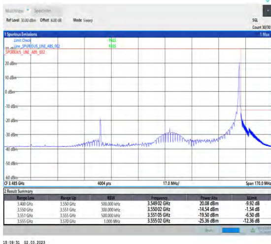
1-N78-3450-3550-PC2-30-90-H-5-CP-QPSK-Edge_1R B_Right-1@244-Ant1-1--PASS-see graph
