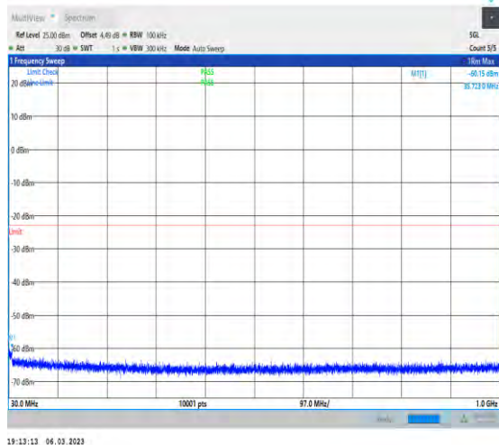
1-N78-3450-3550-PC2-30-100-L-1-DFT-QPSK-Edge e_1RB_Left-1@0-30-1000-Ant1-35.72--60.15--23-P ASS
