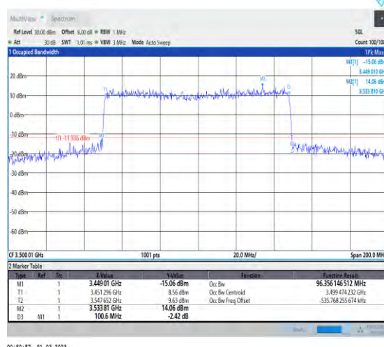
1-N78-3450-3550-30-100-M-3-DFT-16QAM-Outer_F ull-270@0-Ant1-96.356-100.600-≤100-PASS
