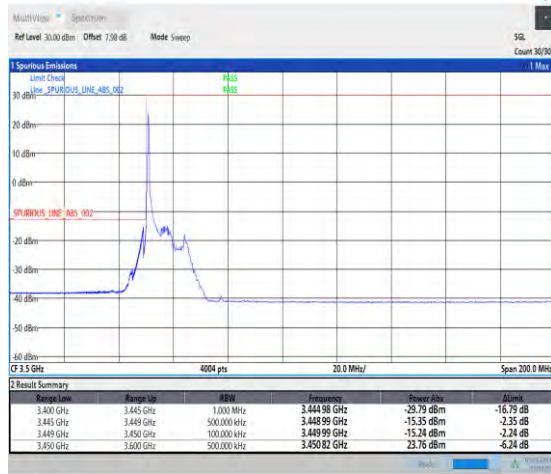
1-N78-3450-3550-30-15-L-1-DFT-PI2BPSK-Edge_1RB _Left-1@0-Ant1-1--PASS-see graph
