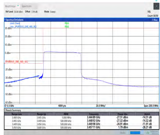
1-N78-3450-3550-30-50-L-6-CP-QPSK-Outer_Full -133@0-Ant1-1--PASS-see graph
