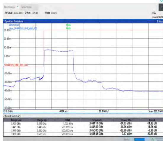
1-N78-3450-3550-30-40-L-3-DFT-PI2BPSK-Outer _Full-100@0-Ant1-1--PASS-see graph
