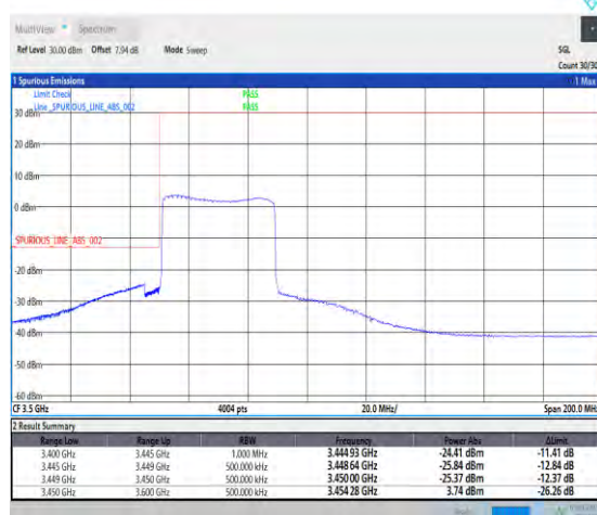
1-N78-3450-3550-30-40-L-6-CP-QPSK-Outer_Full -106@0-Ant1-1--PASS-see graph
