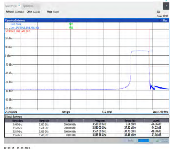
1-N78-3450-3550-PC2-30-20-H-6-CP-QPSK-Outer _Full-51@0-Ant1-1--PASS-see graph
