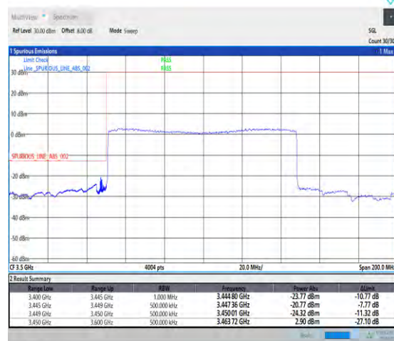
1-N78-3450-3550-30-100-L-3-DFT-PI2BPSK-Outer_Full-270@0-Ant1-1--PASS-see graph
