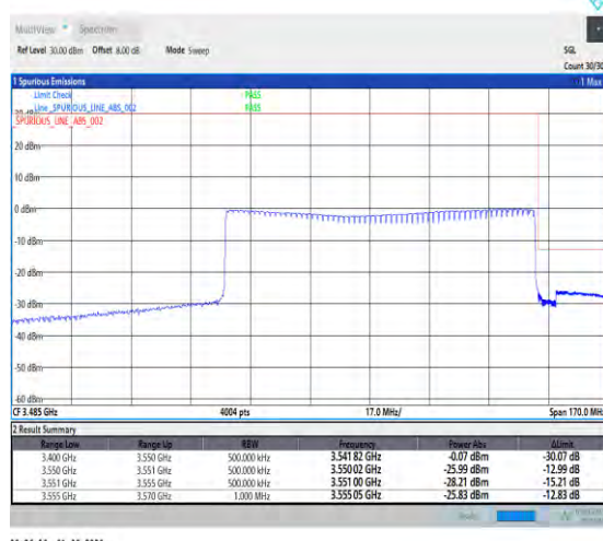
1-N78-3450-3550-30-90-H-6-CP-QPSK-Outer_Full -245@0-Ant1-1--PASS-see graph
