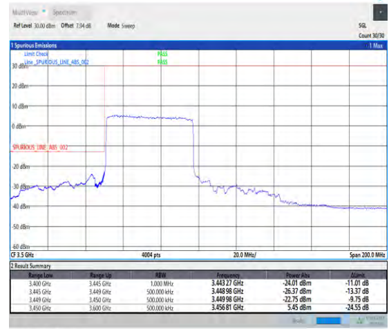
1-N78-3450-3550-30-50-L-3-DFT-PI2BPSK-Outer _Full-128@0-Ant1-1--PASS-see graph
