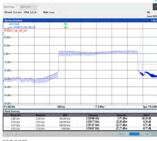
1-N78-3450-3550-30-90-H-3-DFT-PI2BPSK-Outer _Full-240@0-Ant1-1--PASS-see graph
