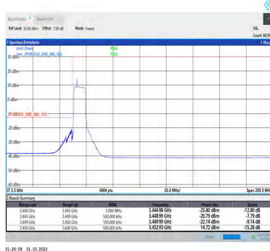
1-N78-3450-3550-30-10-L-6-CP-QPSK-Outer_Full -24@0-Ant1-1--PASS-see graph
