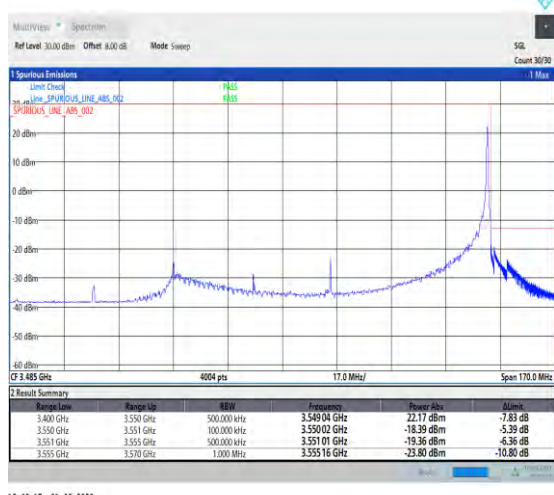
1-N78-3450-3550-30-100-H-5-CP-QPSK-Edge_1RB_Right-1@272-Ant1-1--PASS-see graph
