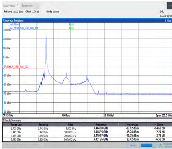
1-N78-3450-3550-30-50-L-1-DFT-PI2BPSK-Edge_1RB _Left-1@0-Ant1-1--PASS-see graph
