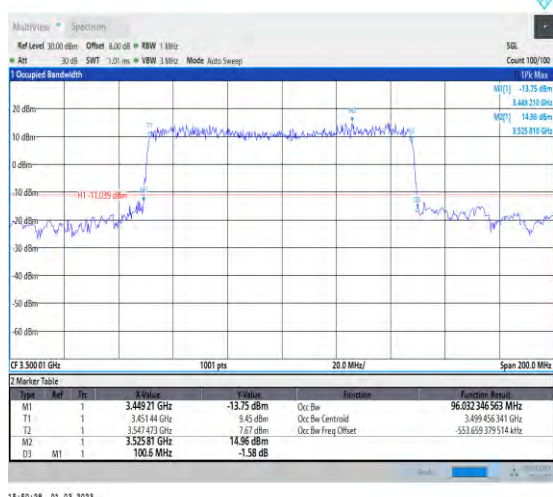
1-N78-3450-3550-30-100-M-2-DFT-PI2BPSK-Outer_ Full-270@0-Ant1-96.032-100.600-≤100-PASS
