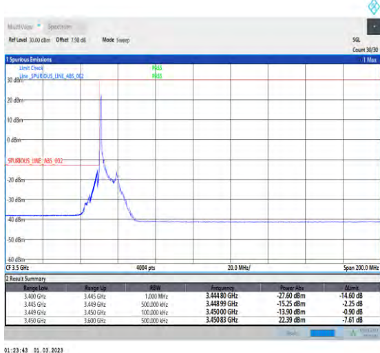
1-N78-3450-3550-30-10-L-4-CP-QPSK-Edge_1RB_Lef t-1@0-Ant1-1--PASS-see graph
