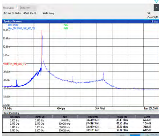
1-N78-3450-3550-30-80-L-4-CP-QPSK-Edge_1RB_Lef t-1@0-Ant1-1--PASS-see graph
