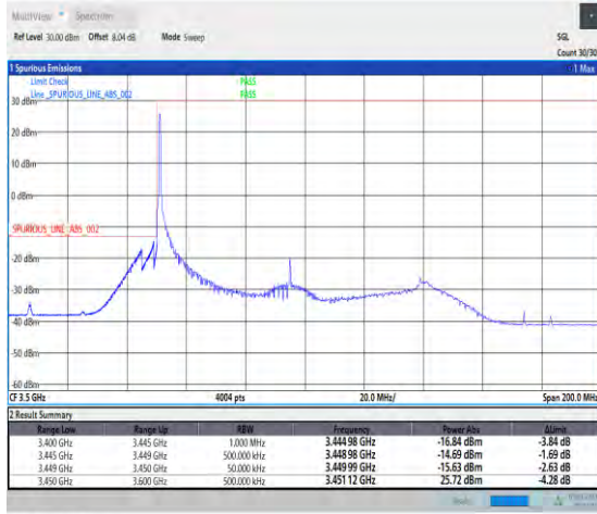
1-N78-3450-3550-30-90-L-1-DFT-PI2BPSK-Edge_1RB _Left-1@0-Ant1-1--PASS-see graph
