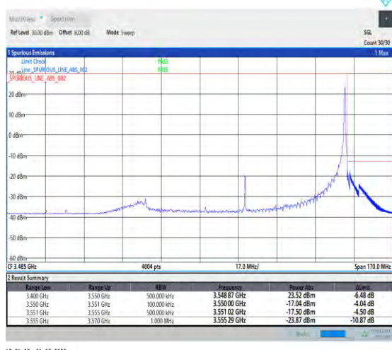
1-N78-3450-3550-30-90-H-5-CP-QPSK-Edge_1RB_Ri ght-1@244-Ant1-1--PASS-see graph
