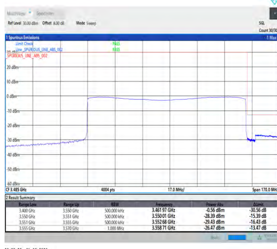
1-N78-3450-3550-30-100-H-6-CP-QPSK-Outer_Full-273@0-Ant1-1--PASS-see graph
