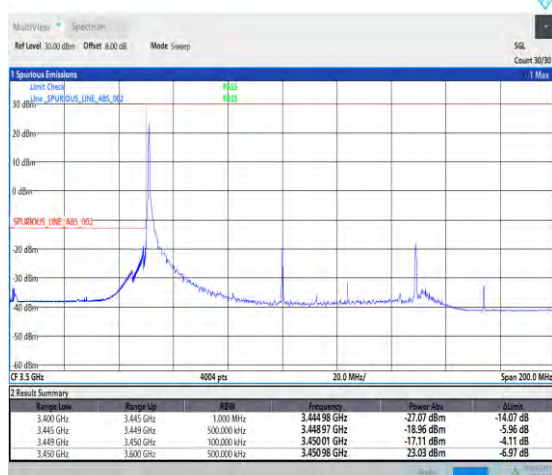
1-N78-3450-3550-30-100-L-4-CP-QPSK-Edge_1RB_Left-1@0-Ant1-1--PASS-see graph
