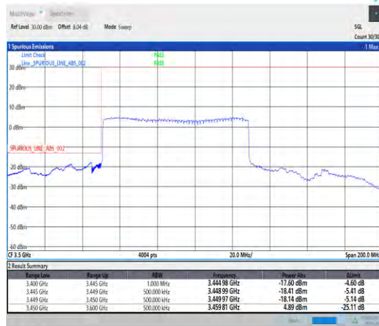
1-N78-3450-3550-30-80-L-3-DFT-PI2BPSK-Outer _Full-216@0-Ant1-1--PASS-see graph
