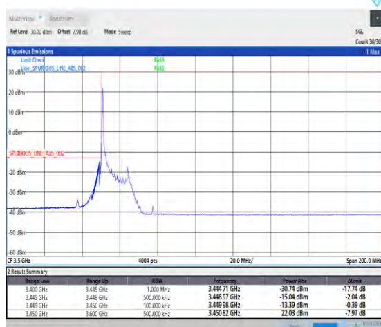
1-N78-3450-3550-30-15-L-4-CP-QPSK-Edge_1RB_Lef t-1@0-Ant1-1--PASS-see graph
