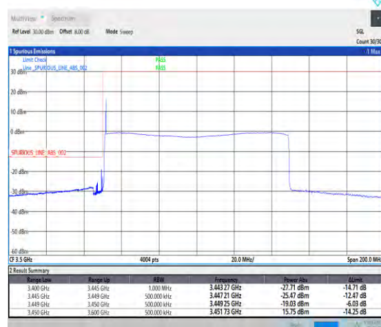
1-N78-3450-3550-30-100-L-6-CP-QPSK-Outer_Full-273@0-Ant1-1--PASS-see graph
