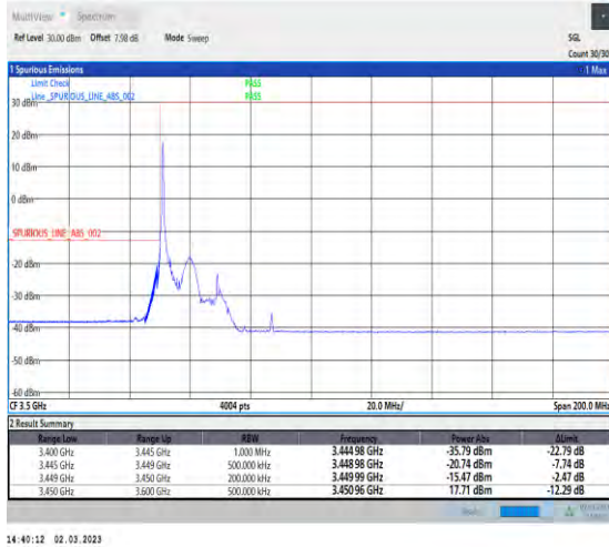
1-N78-3450-3550-PC2-30-20-L-4-CP-QPSK-Edge_1R B_Left-1@0-Ant1-1--PASS-see graph
