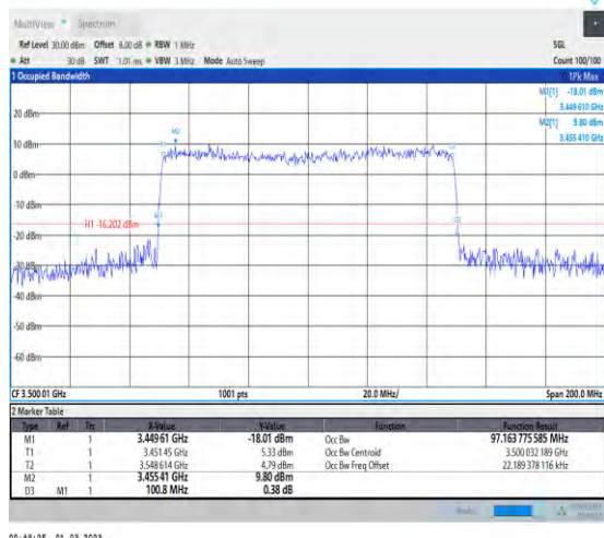
1-N78-3450-3550-30-100-L-9-CP-256QAM-Outer_F ull-273@0-Ant1-97.164-100.800-≤100-PASS
