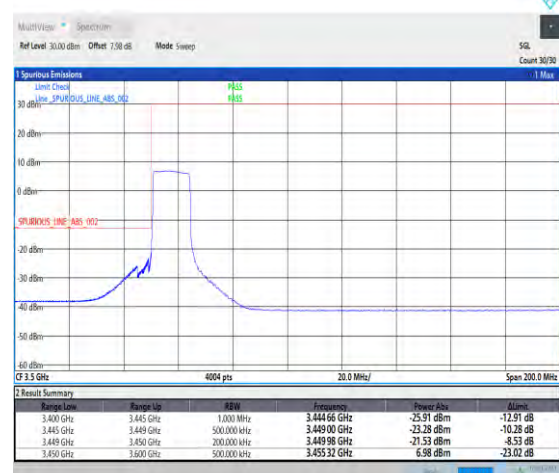
1-N78-3450-3550-30-15-L-6-CP-QPSK-Outer_Full -38@0-Ant1-1--PASS-see graph
