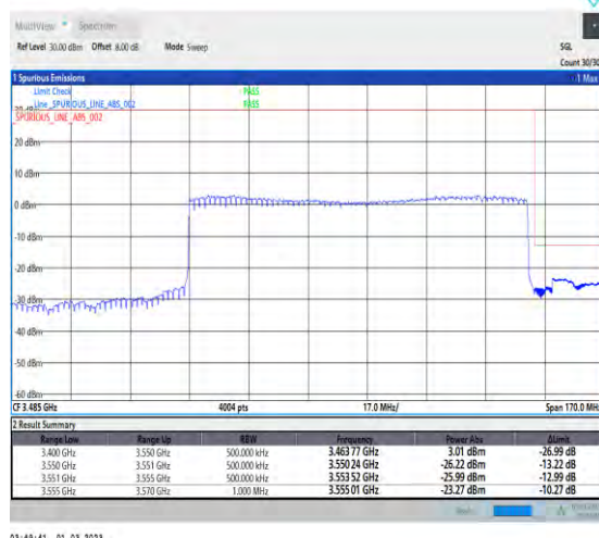
1-N78-3450-3550-30-100-H-3-DFT-PI2BPSK-Oute_r_Full-270@0-Ant1-1--PASS-see graph
