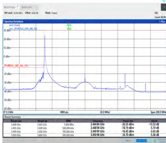
1-N78-3450-3550-30-100-L-1-DFT-PI2BPSK-Edge_1R_B_Left-1@0-Ant1-1--PASS-see graph
