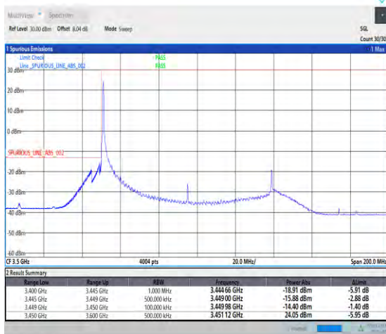
1-N78-3450-3550-30-90-L-4-CP-QPSK-Edge_1RB_Lef t-1@0-Ant1-1--PASS-see graph
