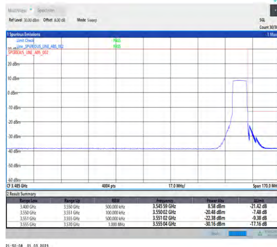
1-N78-3450-3550-PC2-30-10-H-6-CP-QPSK-Outer _Full-24@0-Ant1-1--PASS-see graph
