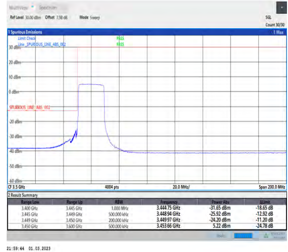
1-N78-3450-3550-PC2-30-20-L-6-CP-QPSK-Outer _Full-51@0-Ant1-1--PASS-see graph
