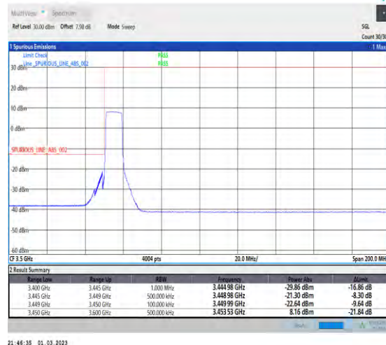
1-N78-3450-3550-PC2-30-10-L-6-CP-QPSK-Outer _Full-24@0-Ant1-1--PASS-see graph
