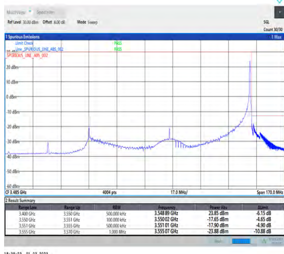
1-N78-3450-3550-30-100-H-2-DFT-PI2BPSK-Edge_1R_B_Right-1@272-Ant1-1--PASS-see graph
