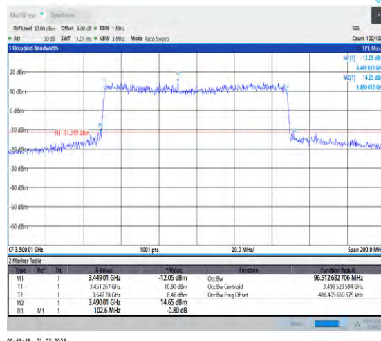
1-N78-3450-3550-30-100-M-1-DFT-QPSK-Outer_Ful l-270@0-Ant1-96.513-102.600-≤100-PASS
