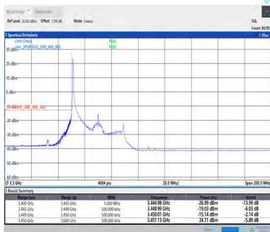
1-N78-3450-3550-30-40-L-1-DFT-PI2BPSK-Edge_1RB _Left-1@0-Ant1-1--PASS-see graph
