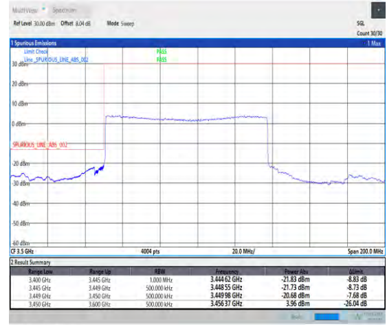
1-N78-3450-3550-30-90-L-3-DFT-PI2BPSK-Outer _Full-240@0-Ant1-1--PASS-see graph
