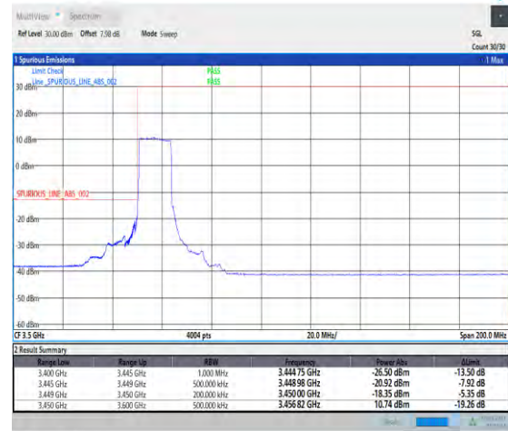
1-N78-3450-3550-30-15-L-3-DFT-PI2BPSK-Outer _Full-36@0-Ant1-1--PASS-see graph
