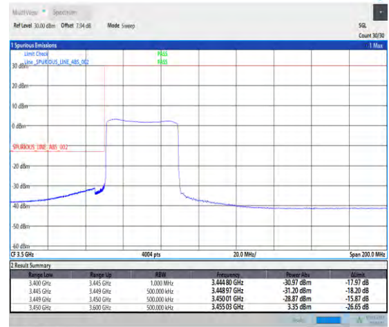
1-N78-3450-3550-PC2-30-40-L-6-CP-QPSK-Outer _Full-106@0-Ant1-1--PASS-see graph
