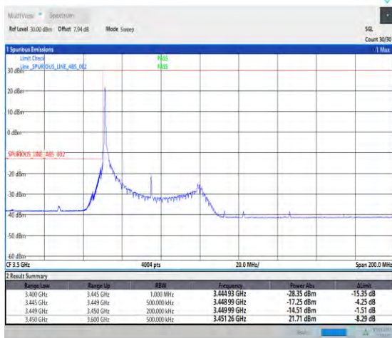
1-N78-3450-3550-30-50-L-4-CP-QPSK-Edge_1RB_Lef t-1@0-Ant1-1--PASS-see graph
