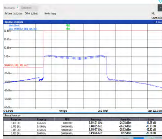
1-N78-3450-3550-30-80-L-6-CP-QPSK-Outer_Full -217@0-Ant1-1--PASS-see graph
