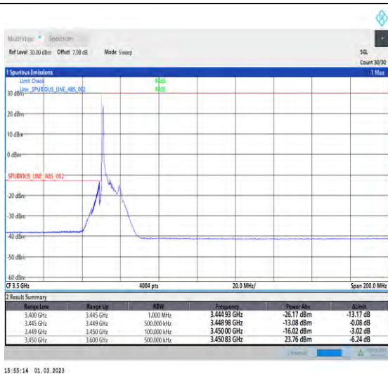
1-N78-3450-3550-30-10-L-1-DFT-PI2BPSK-Edge_1RB _Left-1@0-Ant1-1--PASS-see graph
