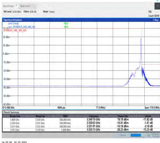
1-N78-3450-3550-PC2-30-10-H-5-CP-QPSK-Edge_1R B_Right-1@23-Ant1-1--PASS-see graph
