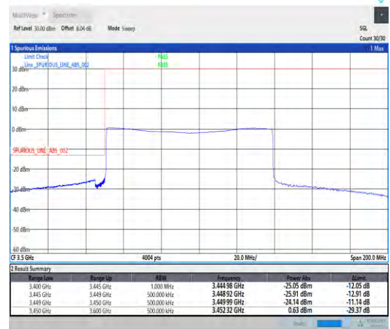
1-N78-3450-3550-30-90-L-6-CP-QPSK-Outer_Full -245@0-Ant1-1--PASS-see graph
