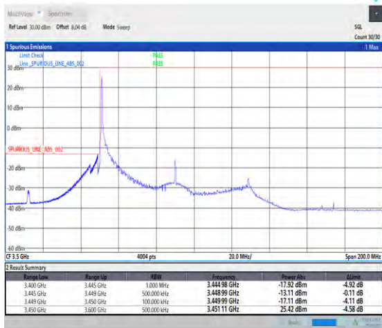
1-N78-3450-3550-30-80-L-1-DFT-PI2BPSK-Edge_1RB _Left-1@0-Ant1-1--PASS-see graph
