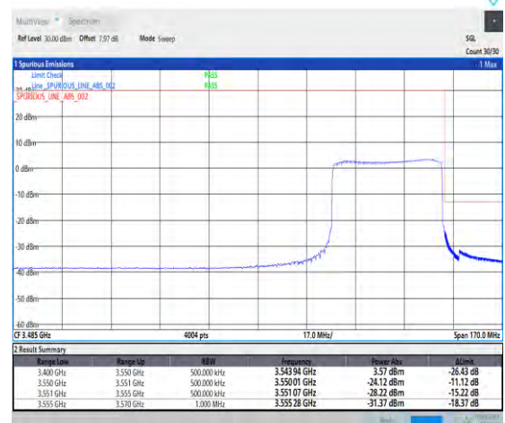
1-N78-3450-3550-PC2-30-40-H-6-CP-QPSK-Outer _Full-106@0-Ant1-1--PASS-see graph
