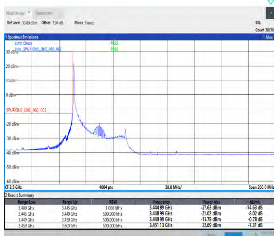
1-N78-3450-3550-30-40-L-4-CP-QPSK-Edge_1RB_Lef t-1@0-Ant1-1--PASS-see graph
