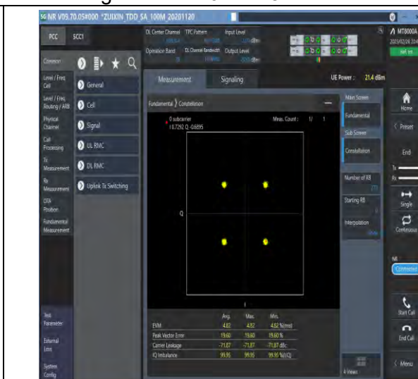
1-N78-3450-3550-30-100-M-6-CP-QPSK-Outer_Full-273@0-Ant1-see graph-PASS
