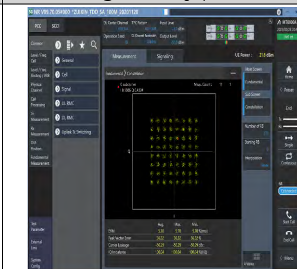
1-N78-3450-3550-30-100-M-8-CP-64QAM-Outer_Full-273@0-Ant1-see graph-PASS
