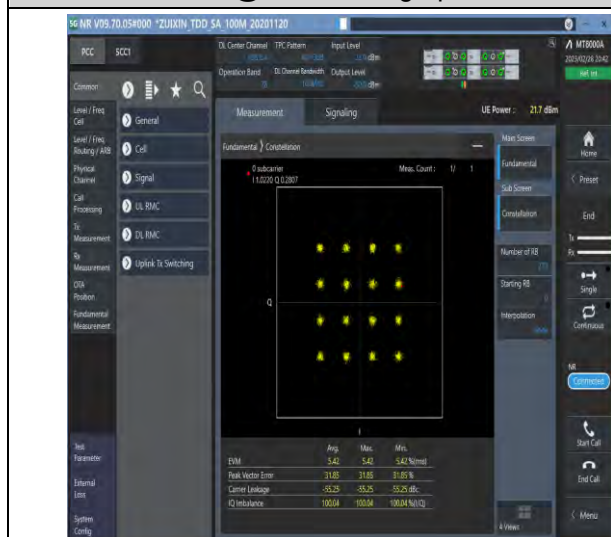
1-N78-3450-3550-30-100-M-7-CP-16QAM-Outer_Full-273@0-Ant1-see graph-PASS
