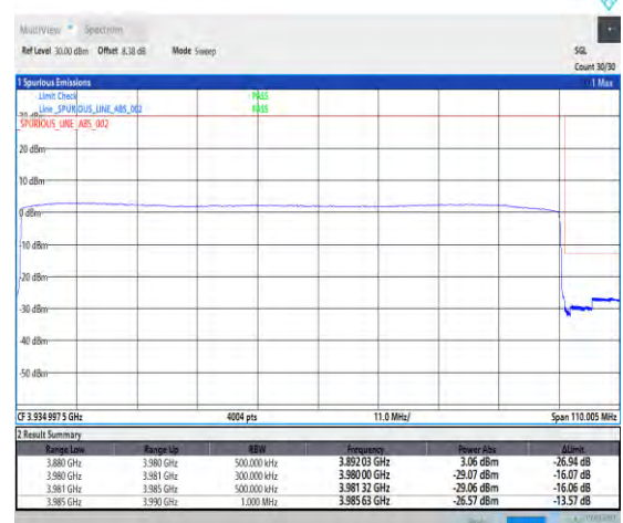
1-N77-3700-3980-30-100-H-6-CP-QPSK-Outer_Full-273@0-Ant1-1--PASS-see graph
