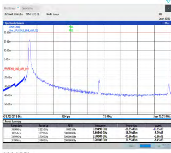
1-N77-3700-3980-30-60-L-4-CP-QPSK-Edge_1RB_Lef t-1@0-Ant1-1--PASS-see graph
