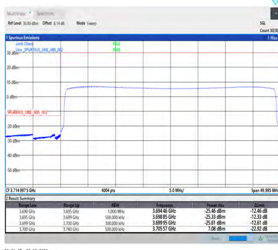
1-N77-3700-3980-30-40-L-6-CP-QPSK-Outer_Full -106@0-Ant1-1--PASS-see graph
