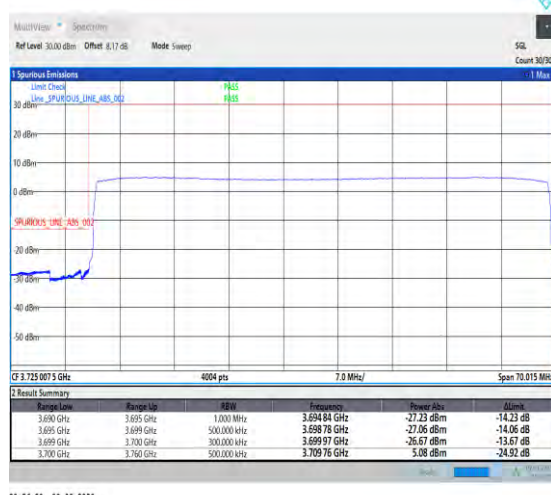
1-N77-3700-3980-30-60-L-6-CP-QPSK-Outer_Full -162@0-Ant1-1--PASS-see graph
