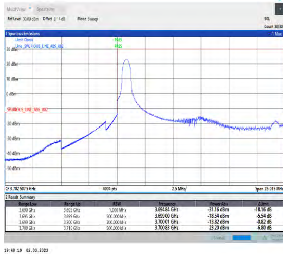
1-N77-3700-3980-30-15-L-1-DFT-PI2BPSK-Edge_1RB_Left-1@0-Ant1-1--PASS-see graph
