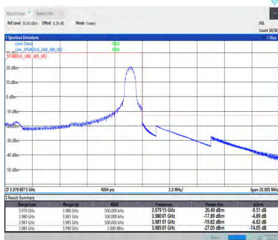
1-N77-3700-3980-30-10-H-5-CP-QPSK-Edge_1RB_Right-1@23-Ant1-1--PASS-see graph
