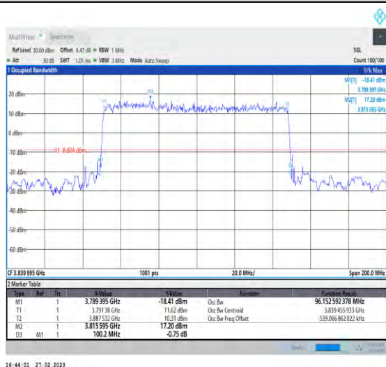
1-N77-3700-3980-30-100-M-2-DFT-PI2BPSK-Outer_Full-270@0-Ant1-96.153-100.200-≤100-PASS
