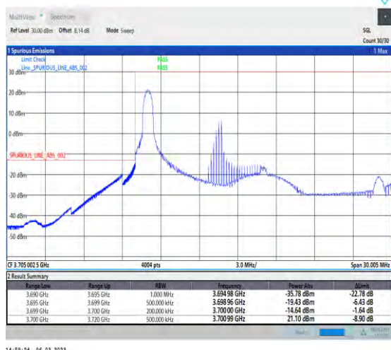
1-N77-3700-3980-30-20-L-1-DFT-PI2BPSK-Edge_1RB_Left-1@0-Ant1-1--PASS-see graph
