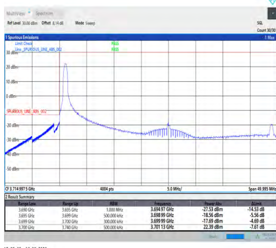
1-N77-3700-3980-30-40-L-4-CP-QPSK-Edge_1RB_Lef t-1@0-Ant1-1--PASS-see graph
