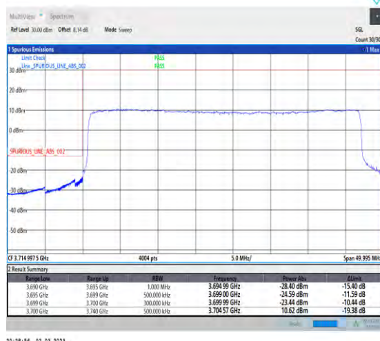
1-N77-3700-3980-30-40-L-3-DFT-PI2BPSK-Outer _Full-100@0-Ant1-1--PASS-see graph
