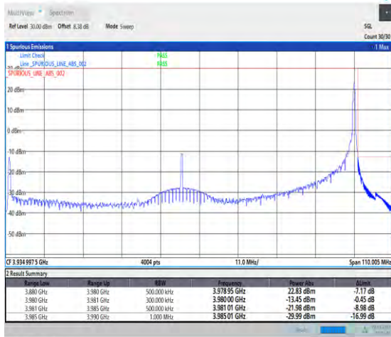
1-N77-3700-3980-30-100-H-2-DFT-PI2BPSK-Edge_1R_B_Right-1@272-Ant1-1--PASS-see graph
