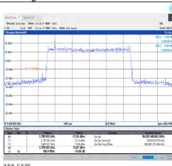
1-N77-3700-3980-30-100-M-1-DFT-QPSK-Outer_Fu II-270@0-Ant1-96.092-100.400-≤100-PASS
