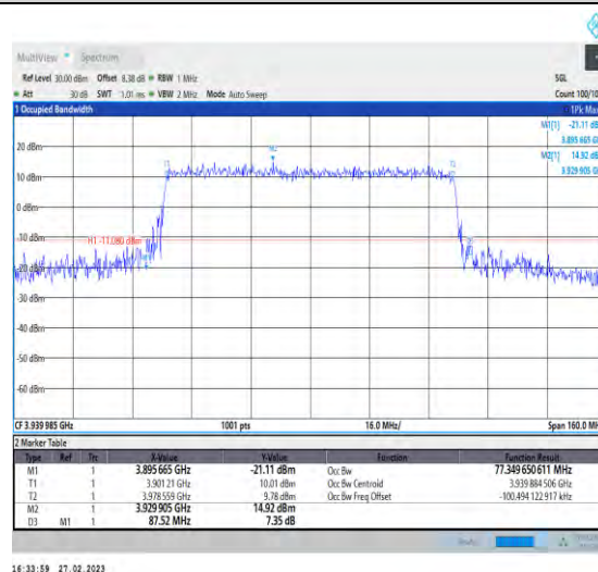
1-N77-3700-3980-30-80-H-8-CP-64QAM-Outer_Full-217@0-Ant1-77.35-87.520-≤80-PASS
