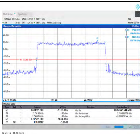
1-N77-3700-3980-30-100-L-9-CP-256QAM-Outer_Fu II-273@0-Ant1-97.051-101.000-≤100-PASS
