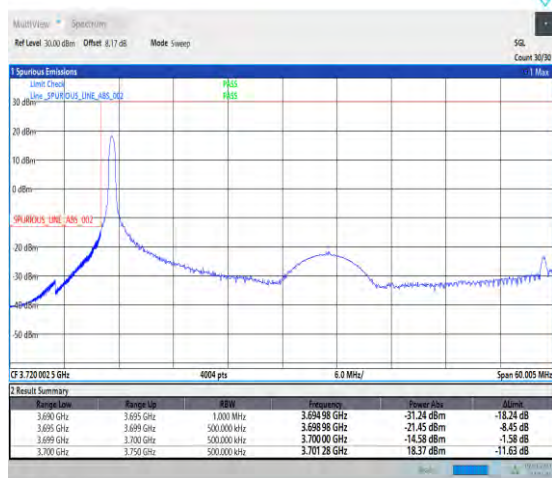
1-N77-3700-3980-PC2-30-50-L-4-CP-QPSK-Edge_1R B_Left-1@0-Ant1-1--PASS-see graph
