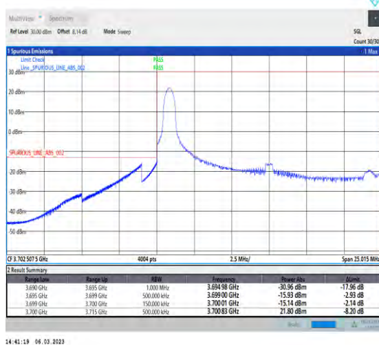
1-N77-3700-3980-30-15-L-4-CP-QPSK-Edge_1RB_Lef t-1@0-Ant1-1--PASS-see graph
