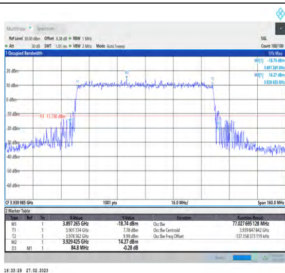
1-N77-3700-3980-30-80-H-5-DFT-256QAM-Outer_Fu II-216@0-Ant1-77.028-84.800-≤80-PASS
