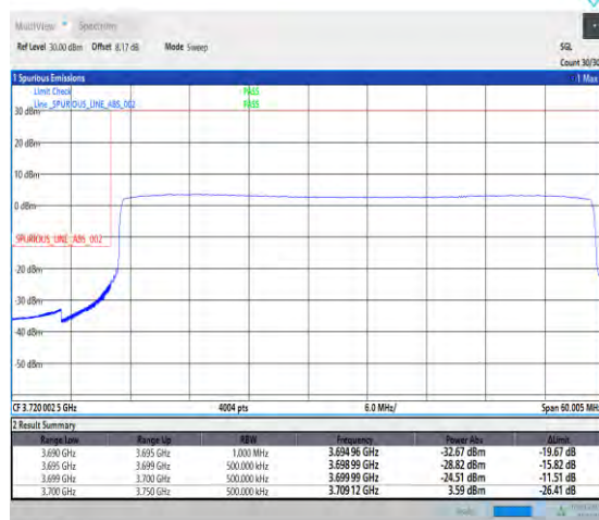
1-N77-3700-3980-PC2-30-50-L-6-CP-QPSK-Outer _Full-133@0-Ant1-1--PASS-see graph
