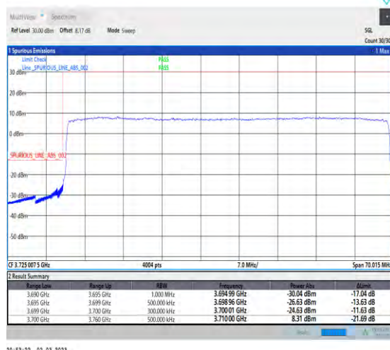
1-N77-3700-3980-30-60-L-3-DFT-PI2BPSK-Outer _Full-162@0-Ant1-1--PASS-see graph
