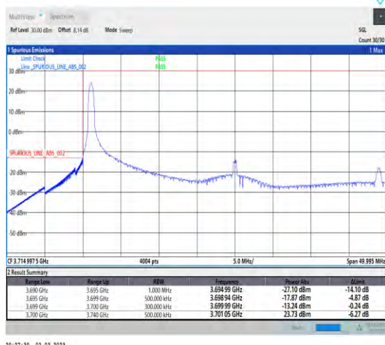
1-N77-3700-3980-30-40-L-1-DFT-PI2BPSK-Edge_1RB _Left-1@0-Ant1-1--PASS-see graph
