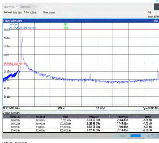
1-N77-3700-3980-30-80-L-1-DFT-PI2BPSK-Edge_1RB _Left-1@0-Ant1-1--PASS-see graph
