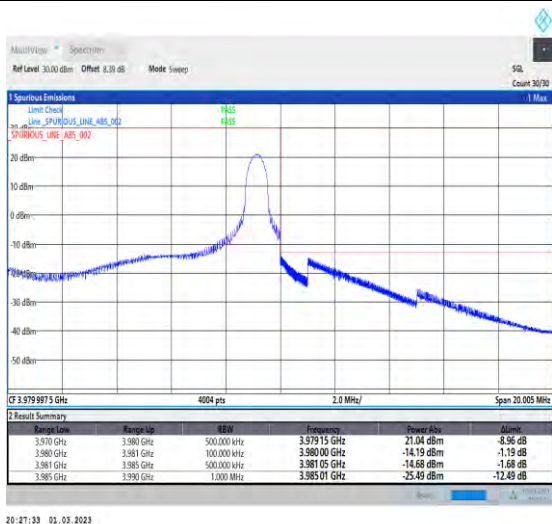
1-N77-3700-3980-PC2-30-10-H-5-CP-QPSK-Edge_1R B_Right-1@23-Ant1-1--PASS-see graph
