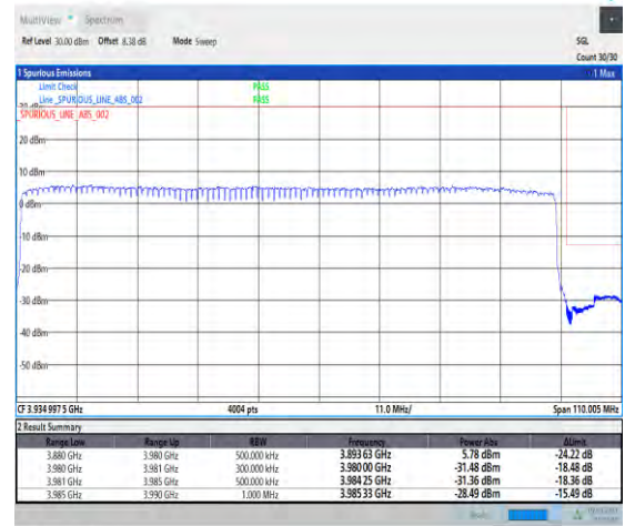
1-N77-3700-3980-30-100-H-3-DFT-PI2BPSK-Outer_Full-270@0-Ant1-1--PASS-see graph
