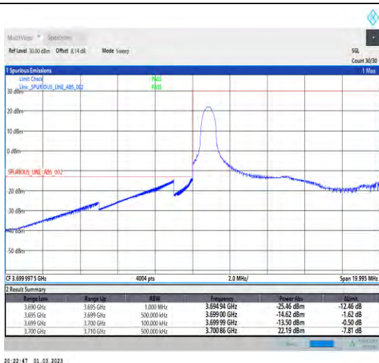
1-N77-3700-3980-PC2-30-10-L-4-CP-QPSK-Edge_1R B_Left-1@0-Ant1-1--PASS-see graph
