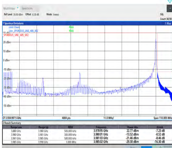
1-N77-3700-3980-30-100-H-5-CP-QPSK-Edge_1RB_Right-1@272-Ant1-1--PASS-see graph
