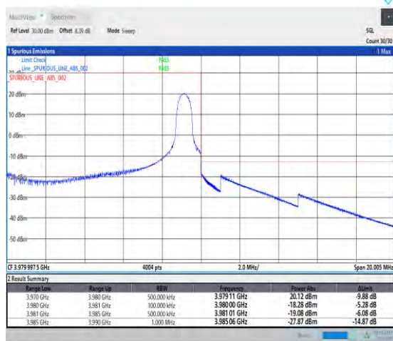
1-N77-3700-3980-30-10-H-2-DFT-PI2BPSK-Edge_1R_B_Right-1@23-Ant1-1--PASS-see graph
