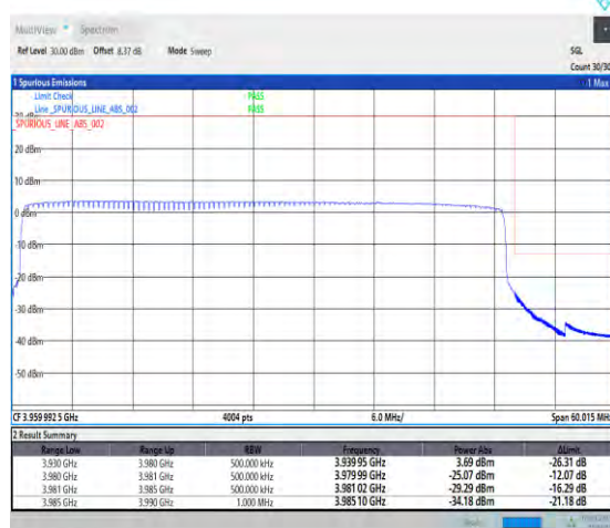
1-N77-3700-3980-PC2-30-50-H-6-CP-QPSK-Outer _Full-133@0-Ant1-1--PASS-see graph
