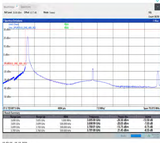
1-N77-3700-3980-30-60-L-1-DFT-PI2BPSK-Edge_1RB _Left-1@0-Ant1-1--PASS-see graph
