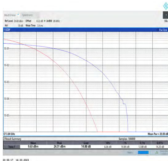
1-N77-3700-3980-30-100-M-1-DFT-256QAM-Outer_F Full-270@0-Ant1-PASS-≤13
