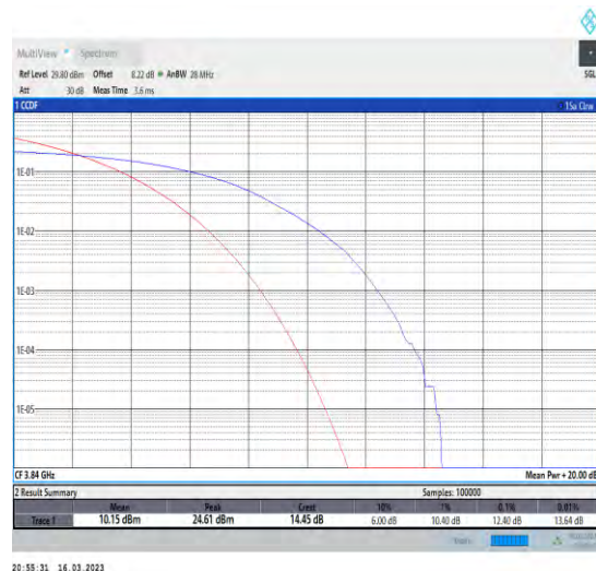
1-N77-3700-3980-30-100-M-2-CP-256QAM-Outer_F ull-273@0-Ant1-PASS-≤13
