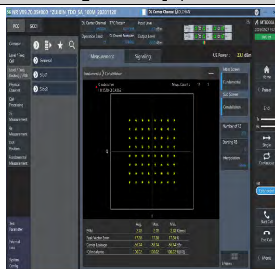
1-N77-3700-3980-30-100-M-8-CP-64QAM-Outer_Full-273@0-Ant1-see graph-PASS
