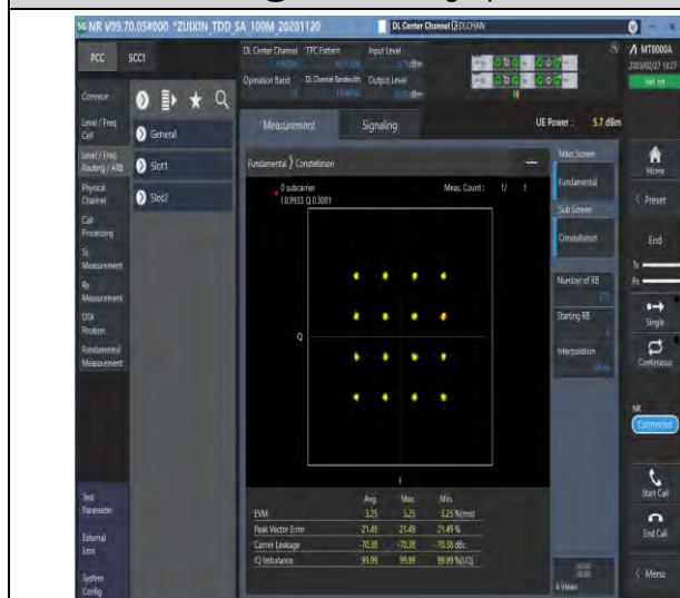
1-N77-3700-3980-30-100-M-7-CP-16QAM-Outer_Full-273@0-Ant1-see graph-PASS
