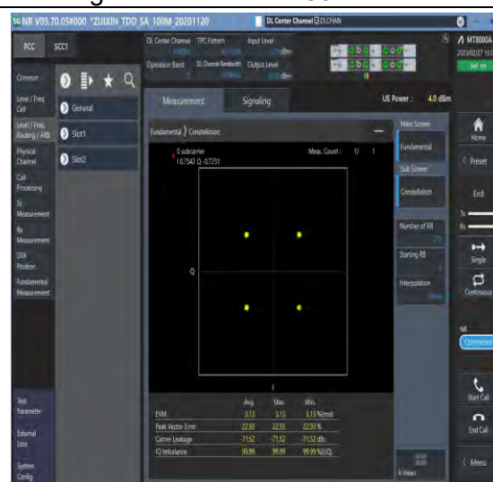
1-N77-3700-3980-30-100-M-6-CP-QPSK-Outer_Full-273@0-Ant1-see graph-PASS
