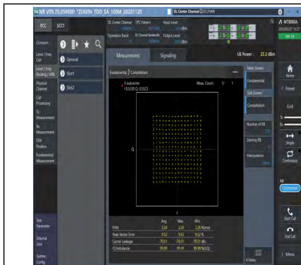
1-N77-3700-3980-30-100-M-5-DFT-256QAM-Outer_Full-270@0-Ant1-see graph-PASS
