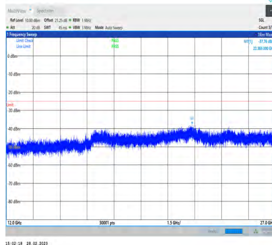
1-N7-PC3-15-20-H-1-DFT-PI2BPSK-Inner_1RB_Left- 1@1-12000-27000-Ant1-22363.00--37.76--25-PASS
