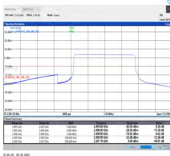
1-N7-PC3-15-5-L-6-CP-QPSK-Outer_Full-25@0-Ant1-1--PASS-see graph
