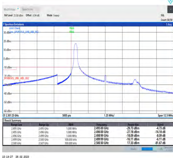
1-N7-PC3-15-5-L-4-CP-QPSK-Edge_1RB_Left-1@0-Ant1-1--PASS-see graph
