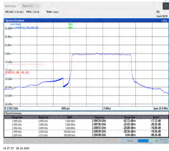
1-N7-PC3-15-10-L-3-DFT-PI2BPSK-Outer_Full-50 @0-Ant1-1--PASS-see graph
