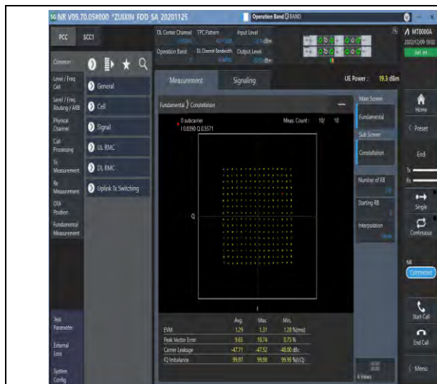
1-N7-15-40-M-5-DFT-256QAM-Outer_Full-216@0-Ant1-see graph-PASS
