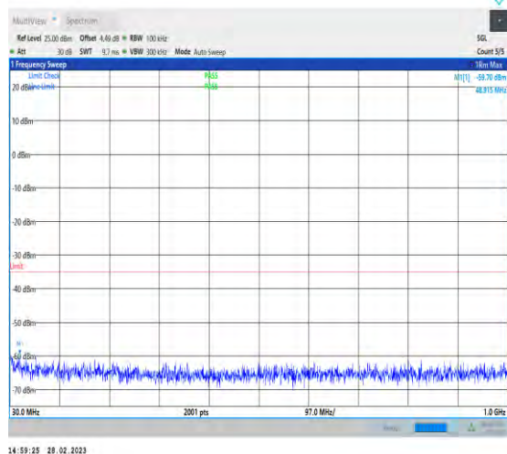
1-N7-PC3-15-20-L-1-DFT-PI2BPSK-Inner_1RB_Left -1@1-30-1000-Ant1-48.92--59.70--35-PASS
