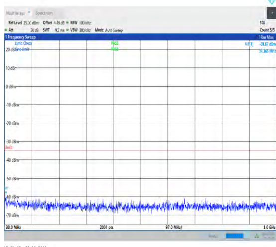
1-N7-PC3-15-20-H-1-DFT-PI2BPSK-Inner_1RB_Lef t-1@1-30-1000-Ant1-34.37--58.87--35-PASS
