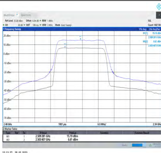
1-N7-PC3-15-20-L-1-DFT-256QAM-Outter_Full-100@ 0-Ant1-8.58-100%-0.00-8.58-PASS-≤13
