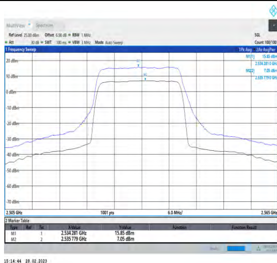
1-N7-PC3-15-20-M-1-DFT-256QAM-Outter_Full-100 @0-Ant1-8.80-100%-0.00-8.80-PASS-≤13
