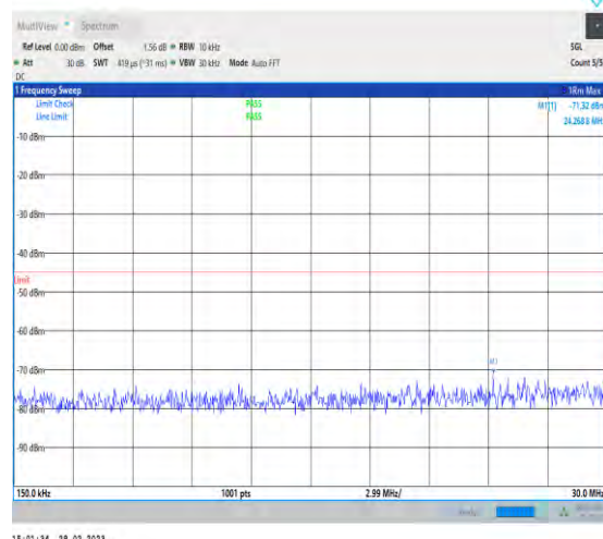
1-N7-PC3-15-20-H-1-DFT-PI2BPSK-Inner_1RB_Left- 1@1-0.15-30-Ant1-24.27--71.32--45-PASS
