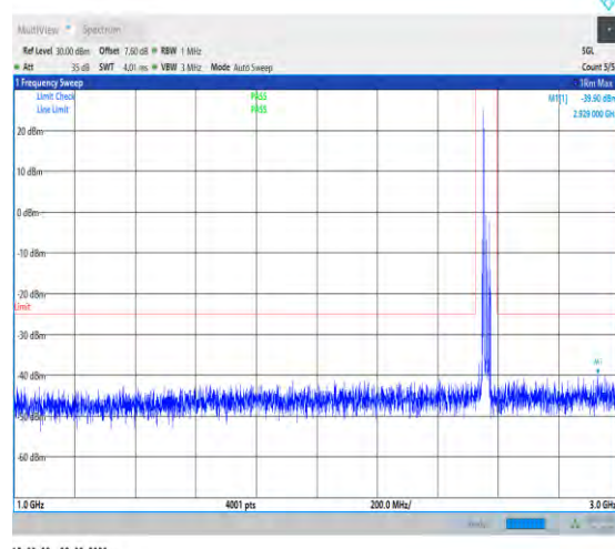
1-N7-PC3-15-20-H-1-DFT-PI2BPSK-Inner_1RB_Left- 1@1-1000-3000-Ant1-2929.00--39.90--25-PASS
