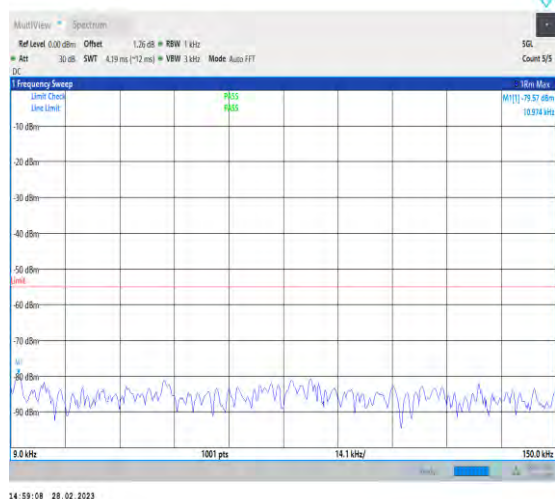
1-N7-PC3-15-20-L-1-DFT-PI2BPSK-Inner_1RB_Left -1@1-0.009-0.15-Ant1-0.01--79.57--55-PASS
