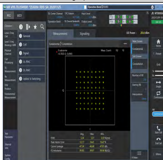
1-N7-15-40-M-8-CP-64QAM-Outer_Full-216@0-Ant1-see graph-PASS
