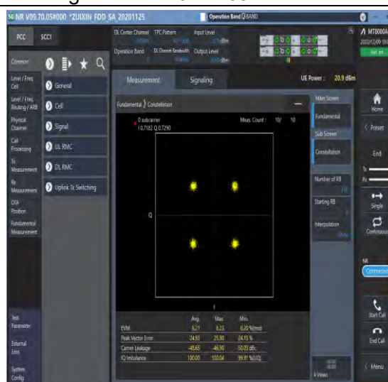
1-N7-15-40-M-6-CP-QPSK-Outer_Full-216@0-Ant1-see graph-PASS
