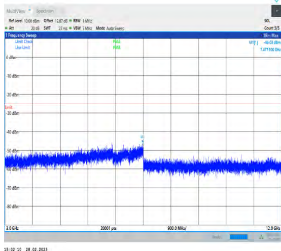
1-N7-PC3-15-20-H-1-DFT-PI2BPSK-Inner_1RB_Lef t-1@1-3000-12000-Ant1-7477.50--46.03--25-PASS
