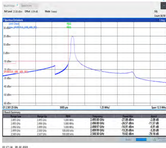
1-N7-PC3-15-5-L-1-DFT-PI2BPSK-Edge_1RB_Left-1@0-Ant1-1--PASS-see graph
