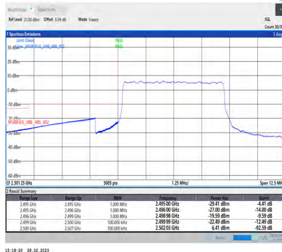
1-N7-PC3-15-5-L-3-DFT-PI2BPSK-Outer_Full-25@0-Ant1-1--PASS-see graph
