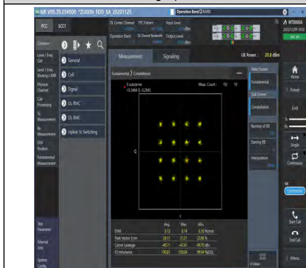
1-N7-15-40-M-7-CP-16QAM-Outer_Full-216@0-Ant1-see graph-PASS
