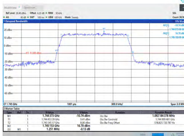
Band66-1.4MHz-QPSK-132322-6RB#0
