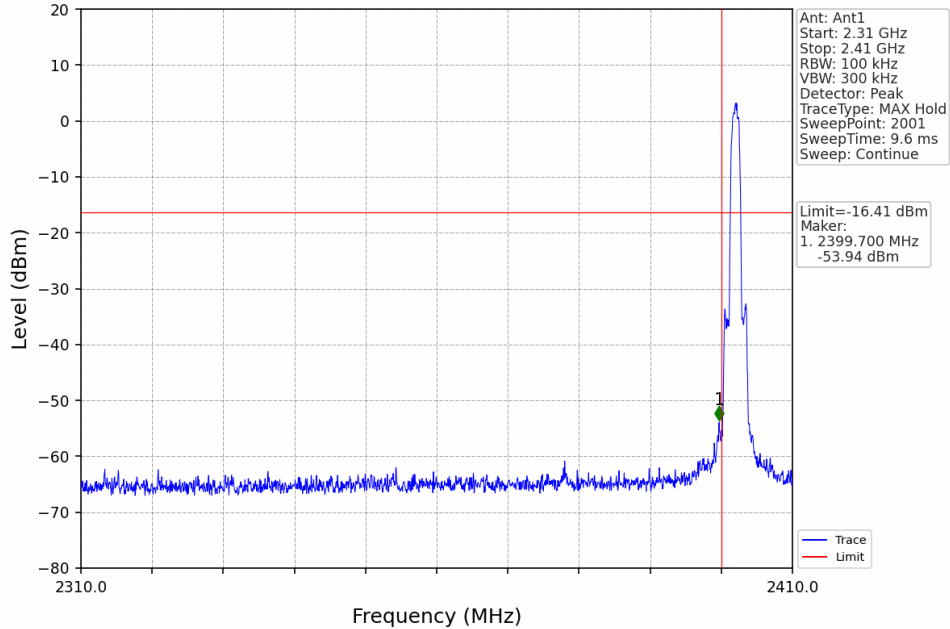
8DPSK_3DH5_LCH_2402MHz_Ant1_NTNV
