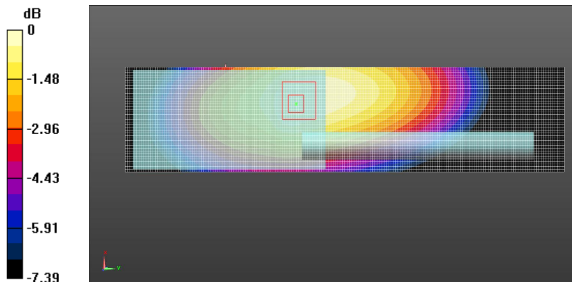
Figure 2: PMR_FM12.5KHz_ Body Worn_0mm
