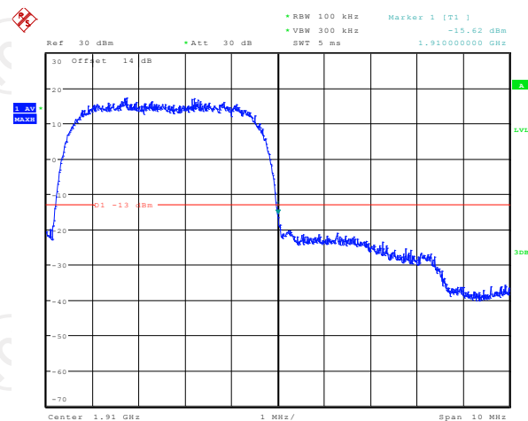
Higher Band Edge Plot on Channel 9538
