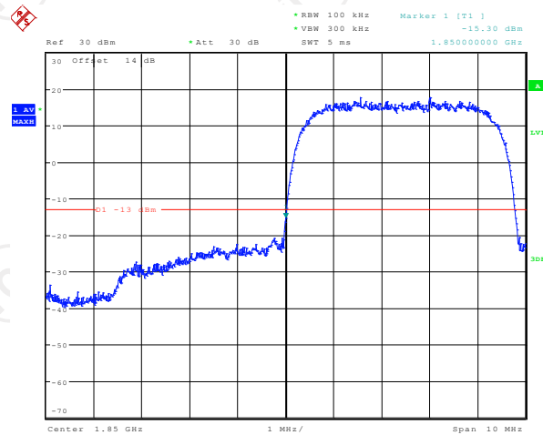
Lower Band Edge Plot on Channel 9262
