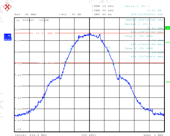
26dB&99% Occupied Bandwidth Plot on Channel 190
