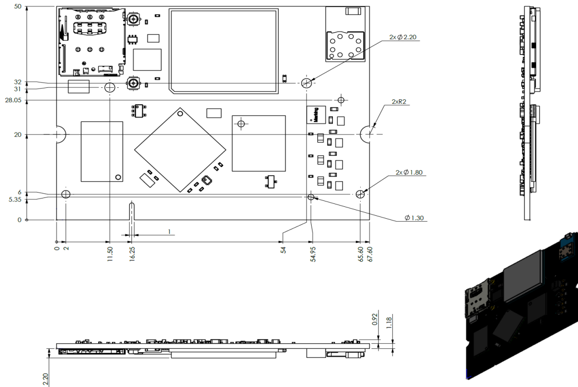
FIGURE 3: MECHANICAL DRAWING
