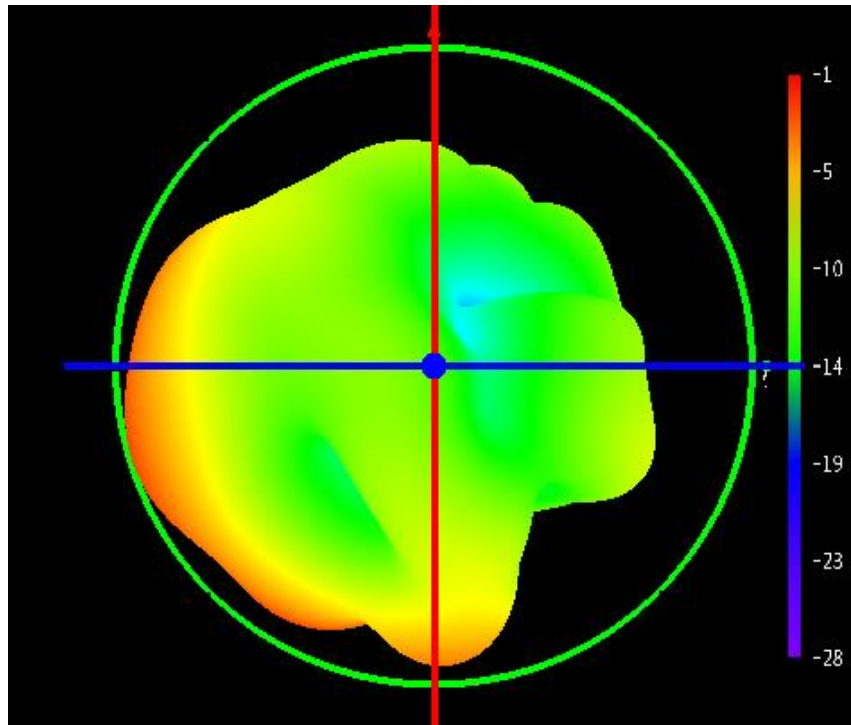
Charts – Antenna Radiation Gain Pattern
