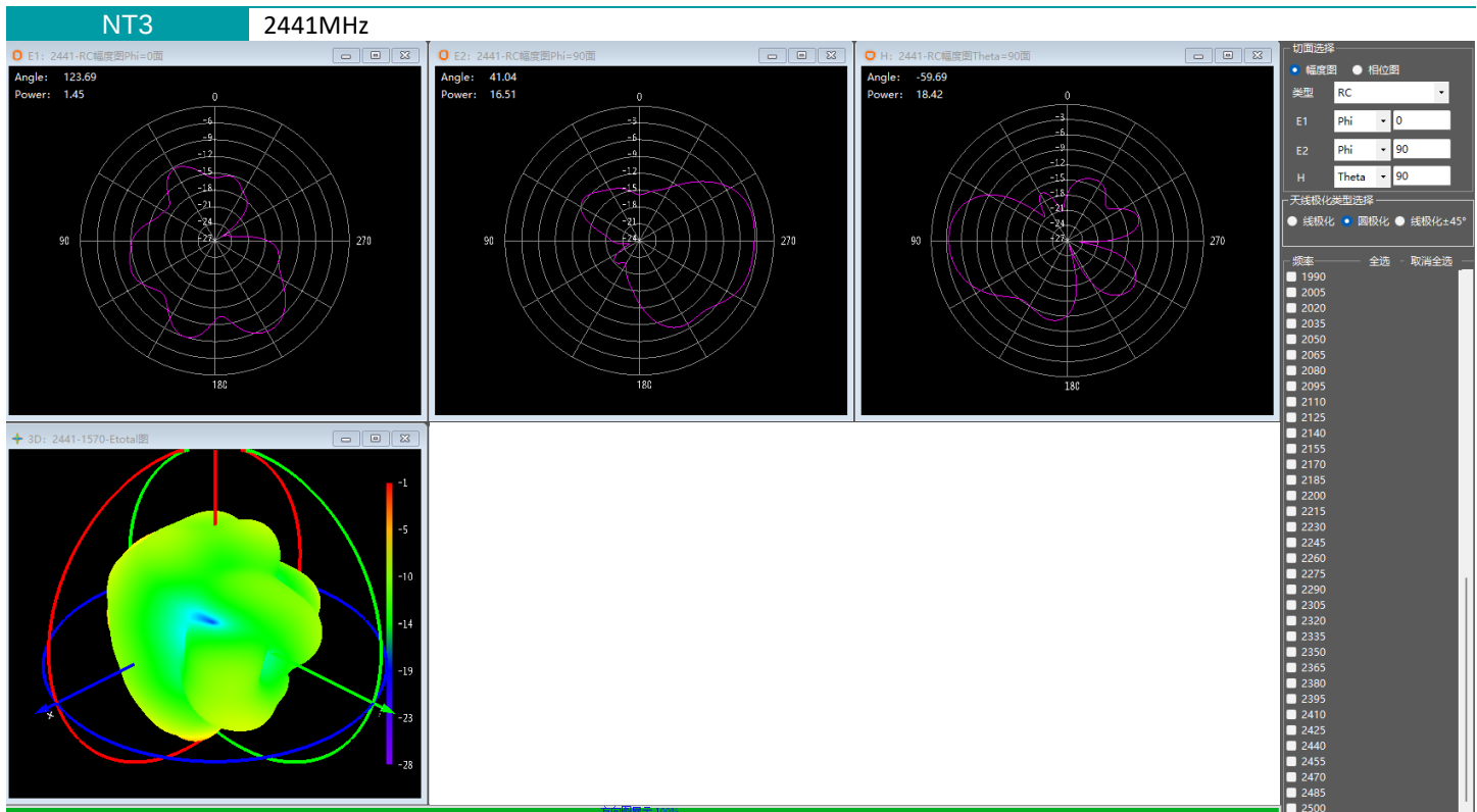
Charts – Antenna Radiation Gain Pattern
