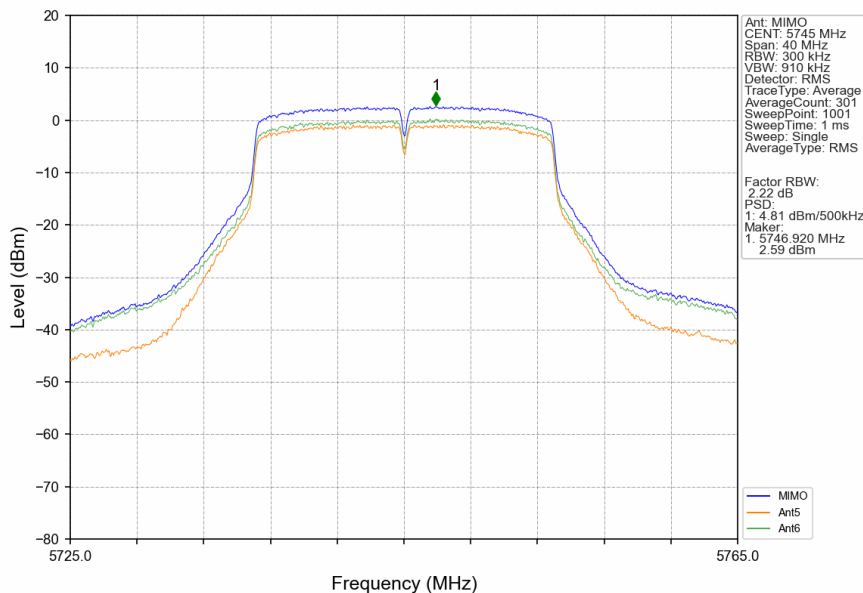
802.11n(HT20)_LCH_5745MHz_MIMO_NTNV
