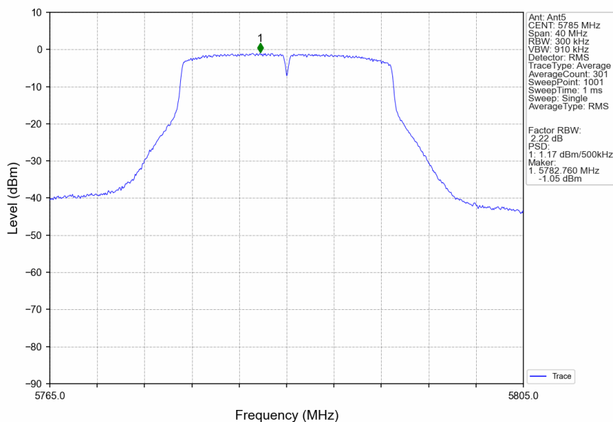
802.11n(HT20)_MCH_5785MHz_Ant5_NTNV
