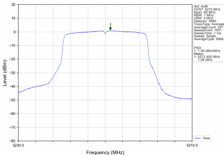
802.11ax(HEW40)_LCH_5270MHz_SU_/_Ant6_NTNV
