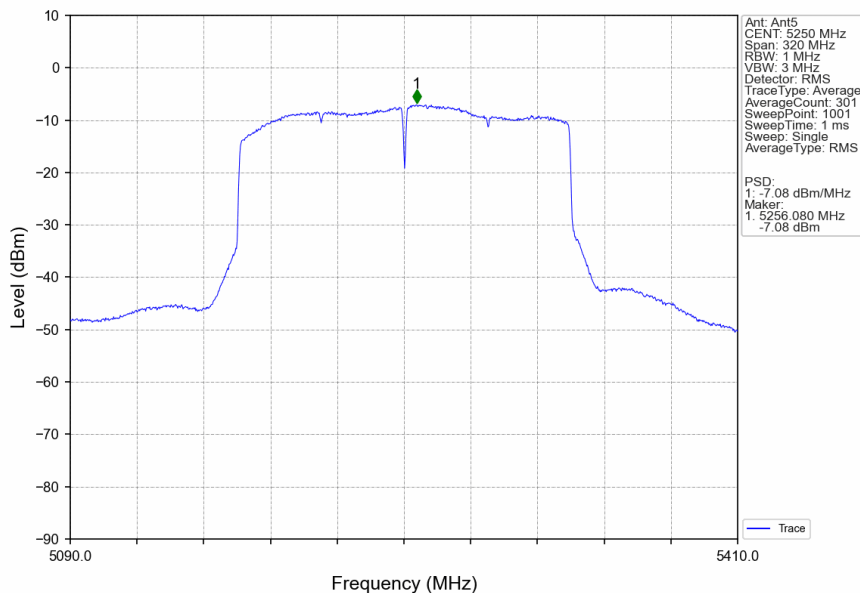
802.11ax(HEW160)_MCH_5250MHz_SU_/_Ant5_NTNV
