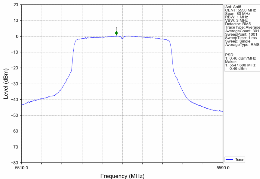
802.11ax(HEW40)_MCH_5550MHz_SU_/_Ant6_NTNV
