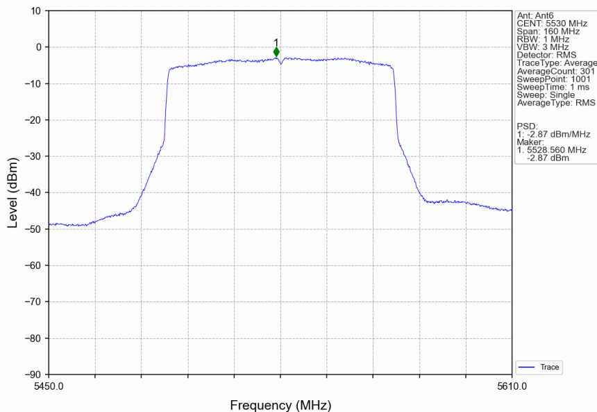
802.11ax(HEW80)_LCH_5530MHz_SU_/_Ant6_NTNV
