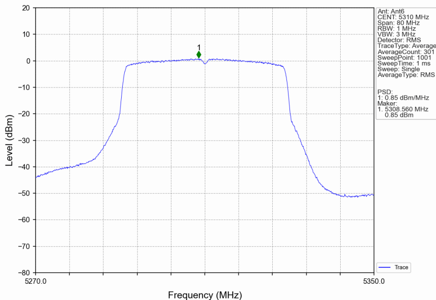
802.11ax(HEW40)_HCH_5310MHz_SU_/_Ant6_NTNV
