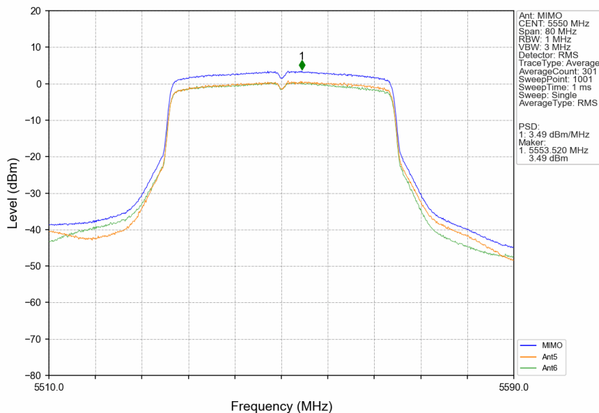
802.11ax(HEW40)_MCH_5550MHz_SU_/_MIMO_NTNV
