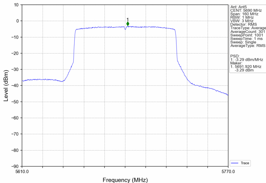
802.11ax(HEW80)_HCH_5690MHz_SU_/_Ant5_NTNV
