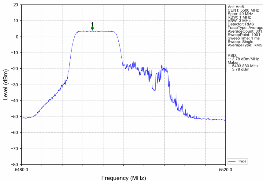
802.11ax(HEW20)_LCH_5500MHz_RU106_Left_Ant6_NTNV
