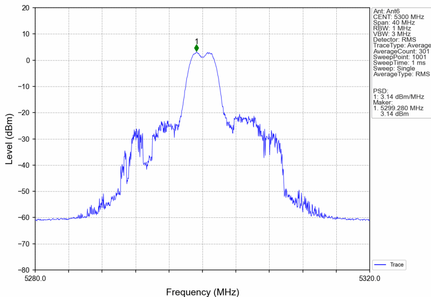
802.11ax(HEW20)_MCH_5300MHz_RU26_Mid_Ant6_NTNV
