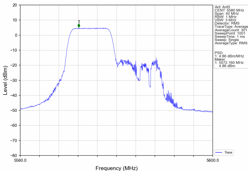
802.11ax(HEW20)_MCH_5580MHz_RU106_Left_Ant5_NTNV
