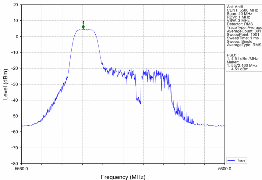
802.11ax(HEW20)_MCH_5580MHz_RU52_Left_Ant6_NTNV
