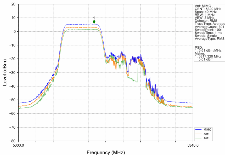
802.11ax(HEW20)_HCH_5320MHz_RU106_Left_MIMO_NTNV
