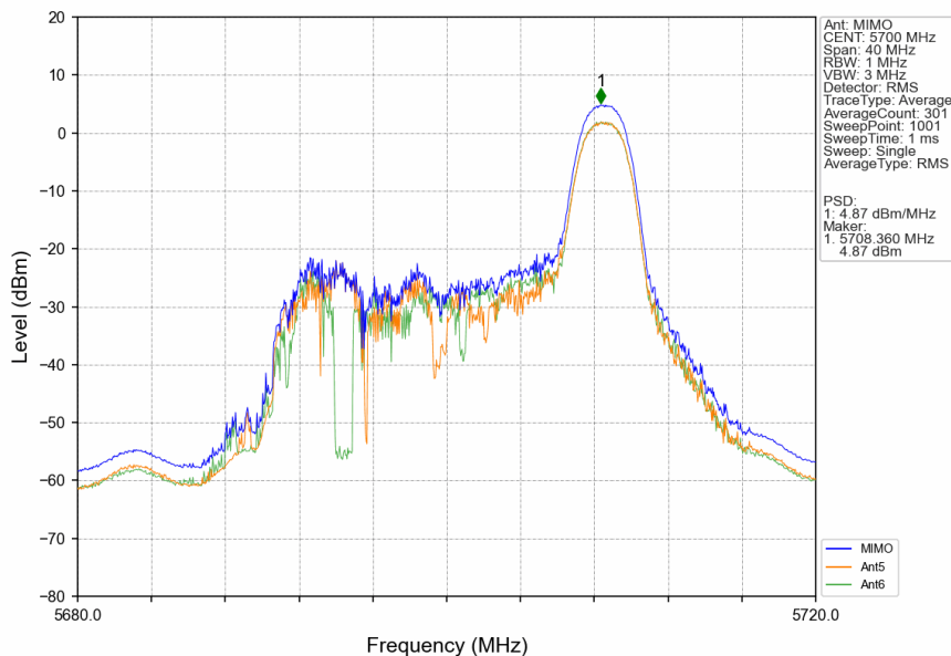
802.11ax(HEW20)_HCH_5700MHz_RU26_Right_MIMO_NTNV
