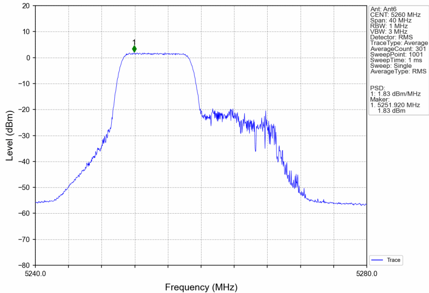
802.11ax(HEW20)_LCH_5260MHz_RU106_Left_Ant6_NTNV
