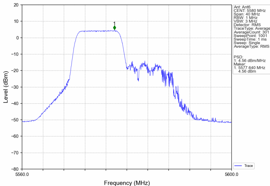
802.11ax(HEW20)_MCH_5580MHz_RU106_Left_Ant6_NTNV
