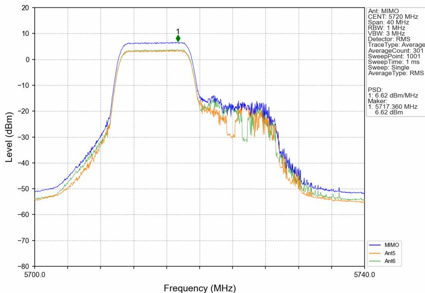
802.11ax(HEW20)_HCH_5720MHz_RU106_Left_MIMO_NTNV
