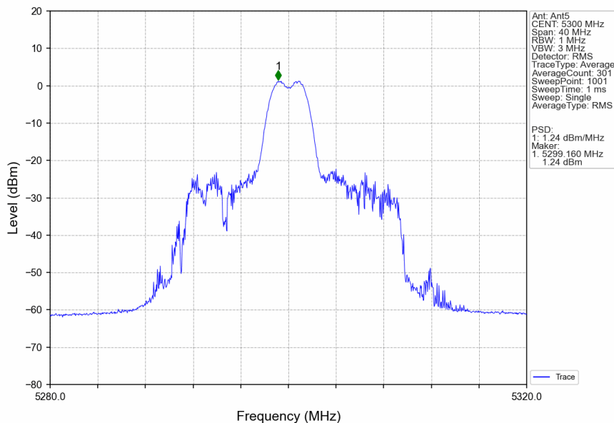
802.11ax(HEW20)_MCH_5300MHz_RU26_Mid_Ant5_NTNV
