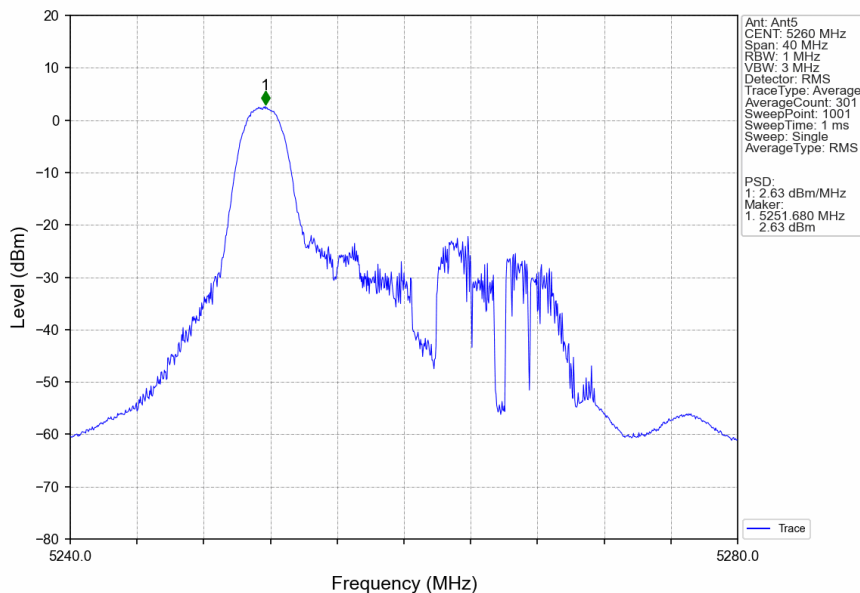
802.11ax(HEW20)_LCH_5260MHz_RU26_Left_Ant5_NTNV
