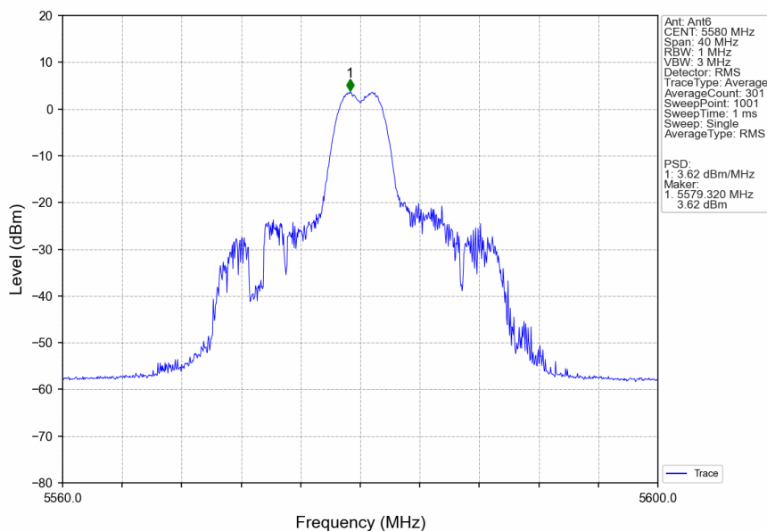
802.11ax(HEW20)_MCH_5580MHz_RU26_Mid_Ant6_NTNV
