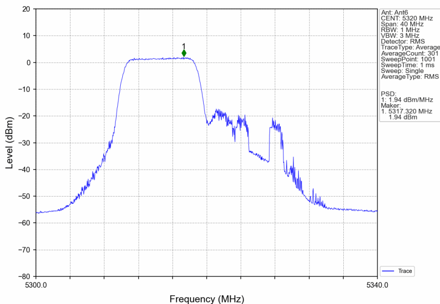
802.11ax(HEW20)_HCH_5320MHz_RU106_Left_Ant6_NTNV
