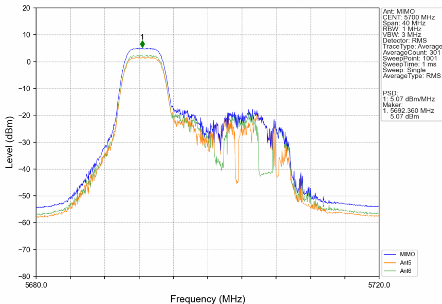
802.11ax(HEW20)_HCH_5700MHz_RU52_Left_MIMO_NTNV
