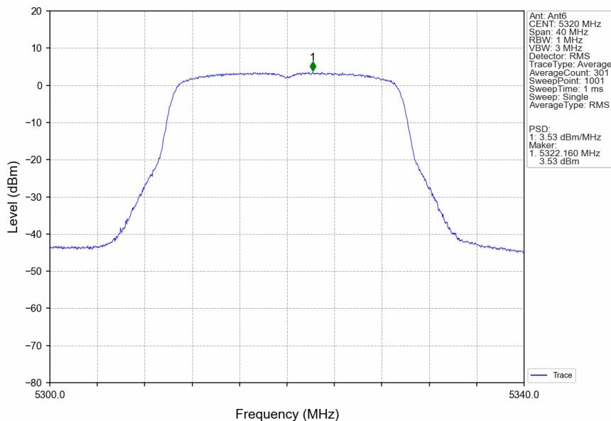
802.11ax(HEW20)_HCH_5320MHz_SU_/_Ant6_NTNV
