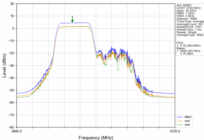
802.11ax(HEW20)_HCH_5700MHz_RU106_Left_MIMO_NTNV
