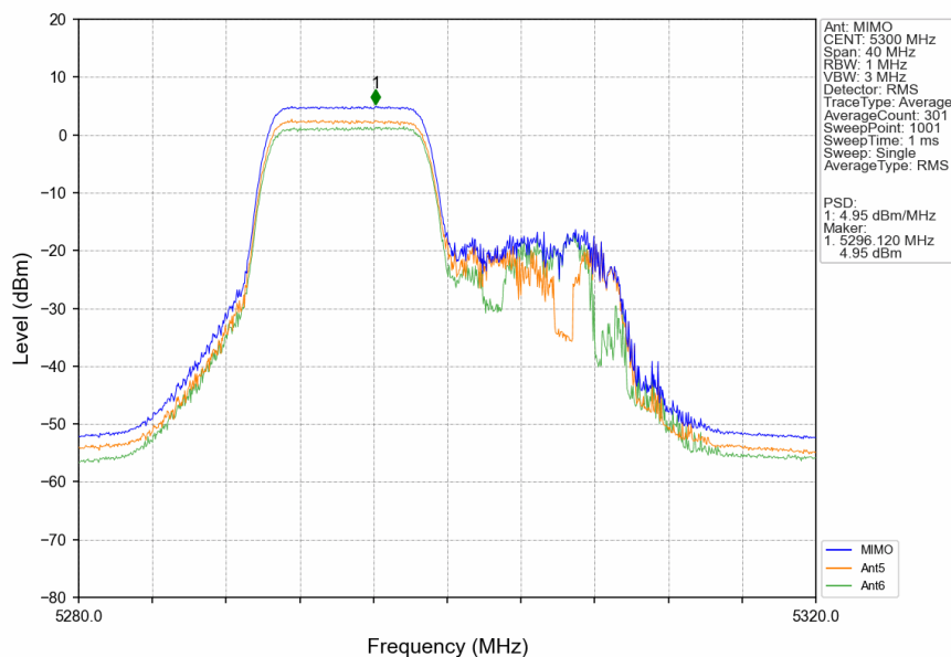
802.11ax(HEW20)_MCH_5300MHz_RU106_Left_MIMO_NTNV
