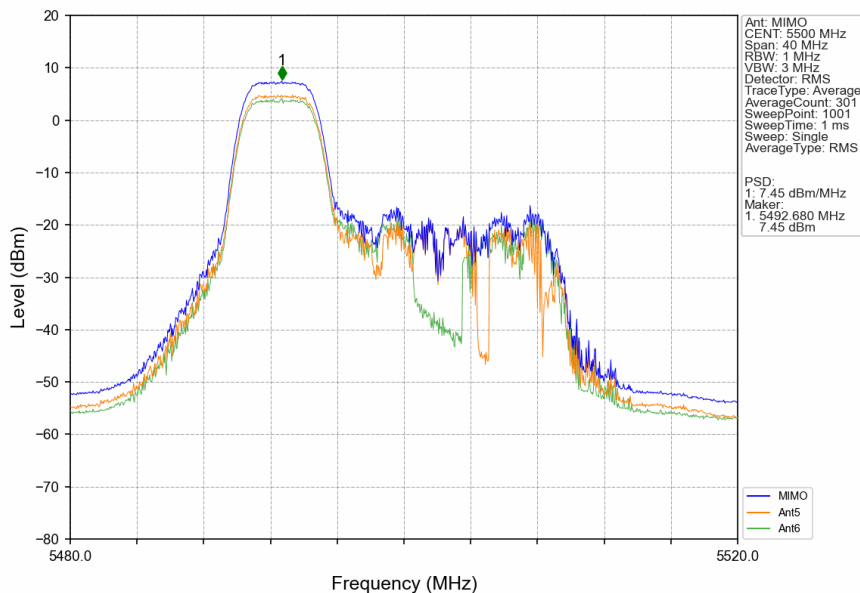
802.11ax(HEW20)_LCH_5500MHz_RU52_Left_MIMO_NTNV
