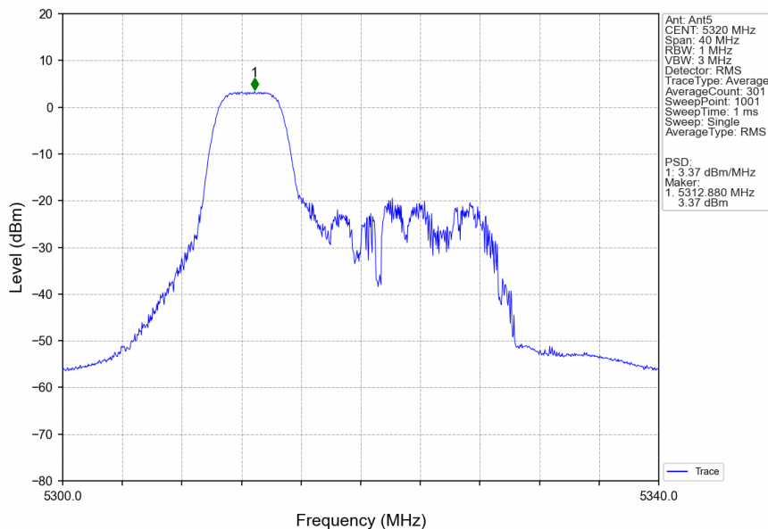
802.11ax(HEW20)_HCH_5320MHz_RU52_Left_Ant5_NTNV
