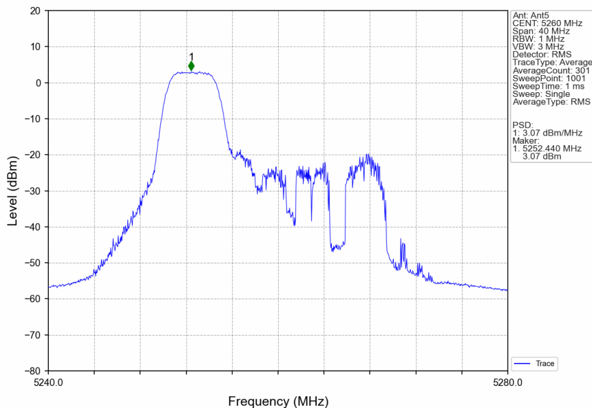
802.11ax(HEW20)_LCH_5260MHz_RU52_Left_Ant5_NTNV
