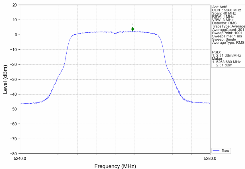
802.11ax(HEW20)_LCH_5260MHz_SU_/_Ant5_NTNV
