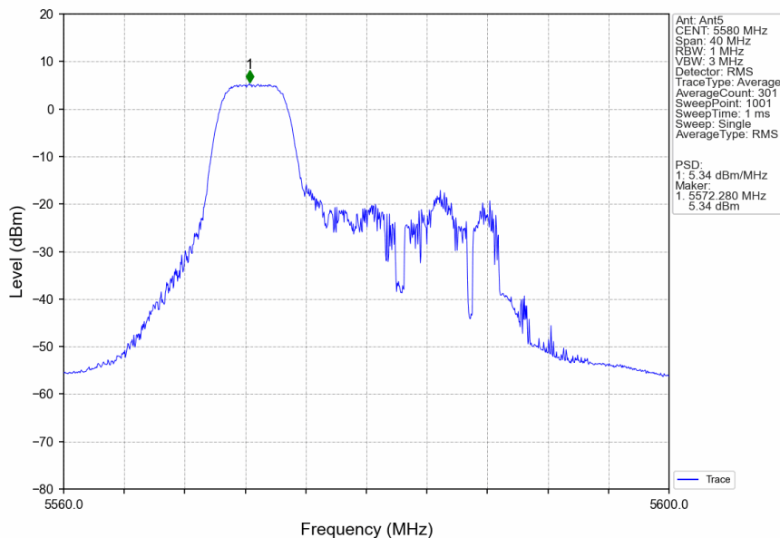
802.11ax(HEW20)_MCH_5580MHz_RU52_Left_Ant5_NTNV
