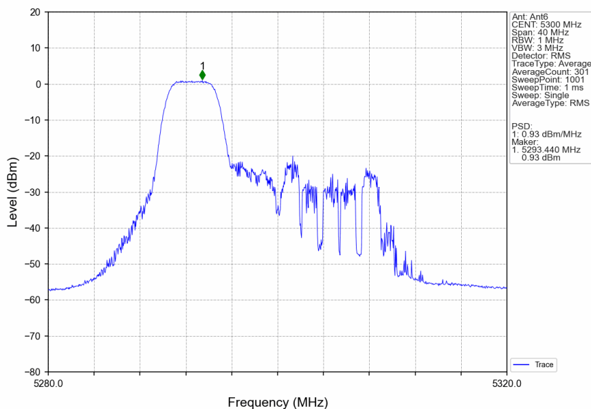
802.11ax(HEW20)_MCH_5300MHz_RU52_Left_Ant6_NTNV
