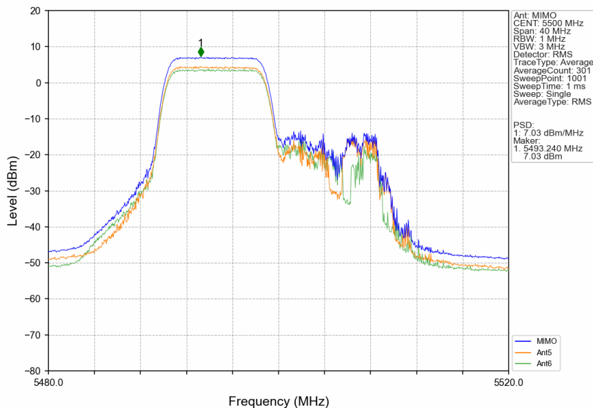
802.11ax(HEW20)_LCH_5500MHz_RU106_Left_MIMO_NTNV
