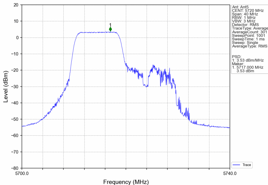
802.11ax(HEW20)_HCH_5720MHz_RU106_Left_Ant5_NTNV
