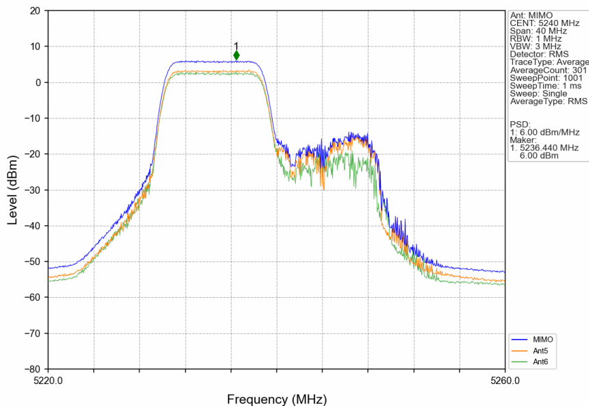
802.11ax(HEW20)_HCH_5240MHz_RU106_Left_MIMO_NTNV
