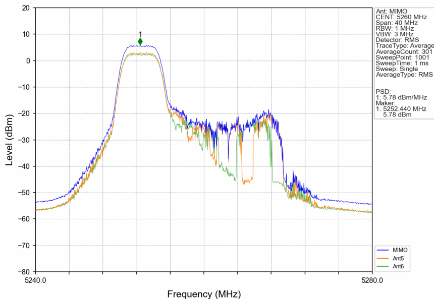
802.11ax(HEW20)_LCH_5260MHz_RU52_Left_MIMO_NTNV
