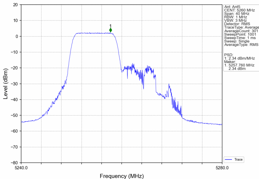
802.11ax(HEW20)_LCH_5260MHz_RU106_Left_Ant5_NTNV
