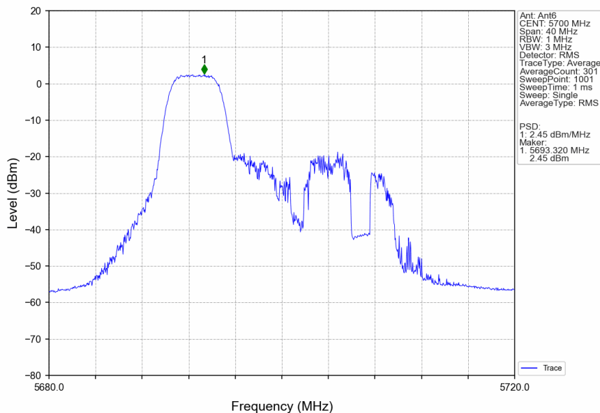
802.11ax(HEW20)_HCH_5700MHz_RU52_Left_Ant6_NTNV
