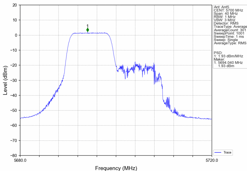
802.11ax(HEW20)_HCH_5700MHz_RU106_Left_Ant5_NTNV
