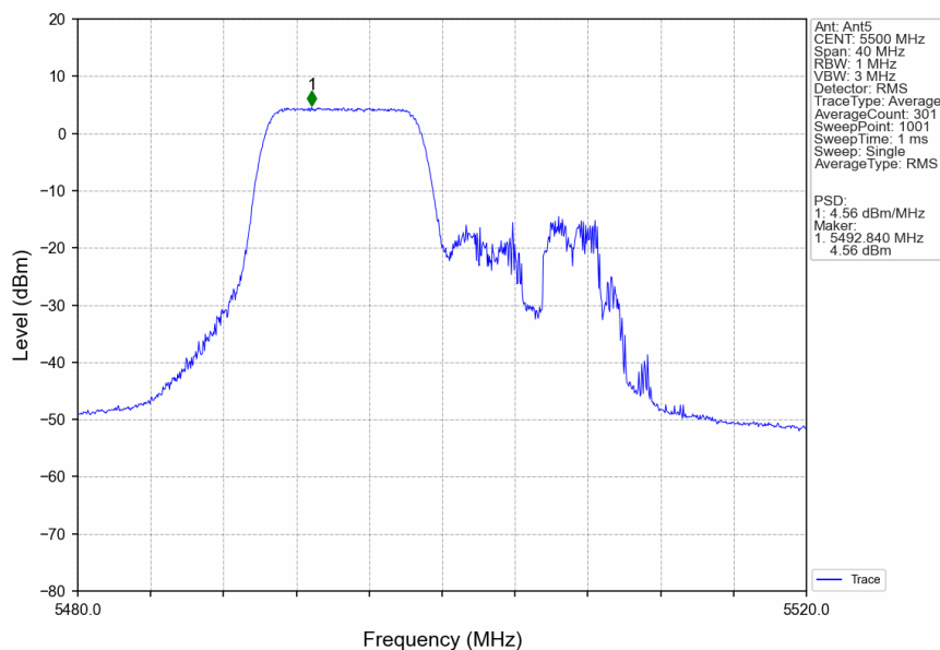
802.11ax(HEW20)_LCH_5500MHz_RU106_Left_Ant5_NTNV
