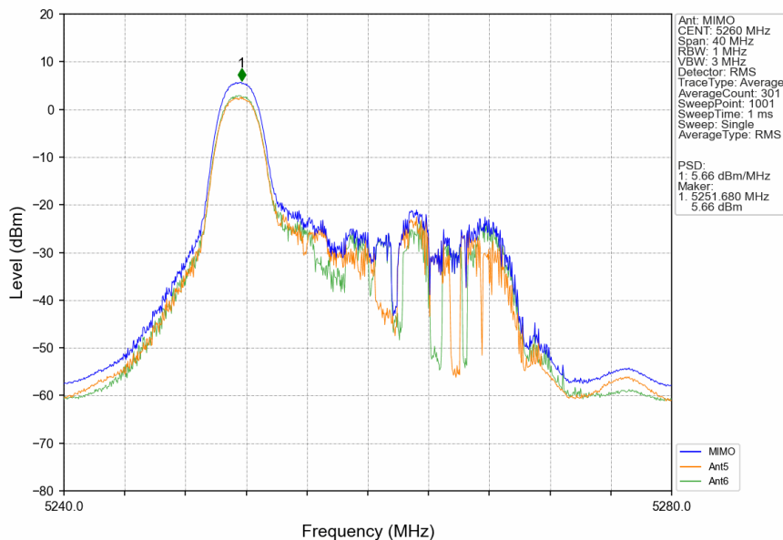
802.11ax(HEW20)_LCH_5260MHz_RU26_Left_MIMO_NTNV
