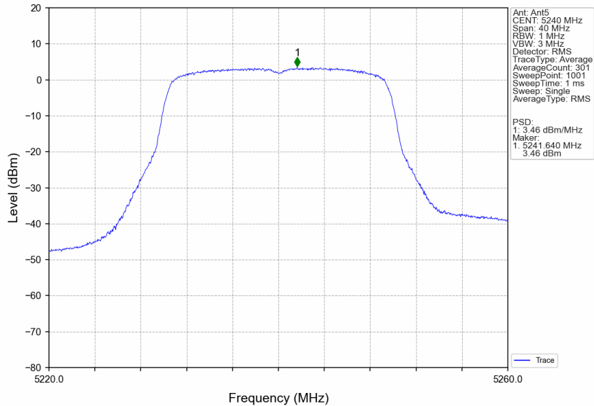
802.11ax(HEW20)_HCH_5240MHz_SU_/_Ant5_NTNV
