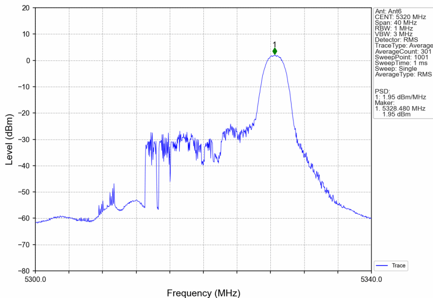
802.11ax(HEW20)_HCH_5320MHz_RU26_Right_Ant6_NTNV
