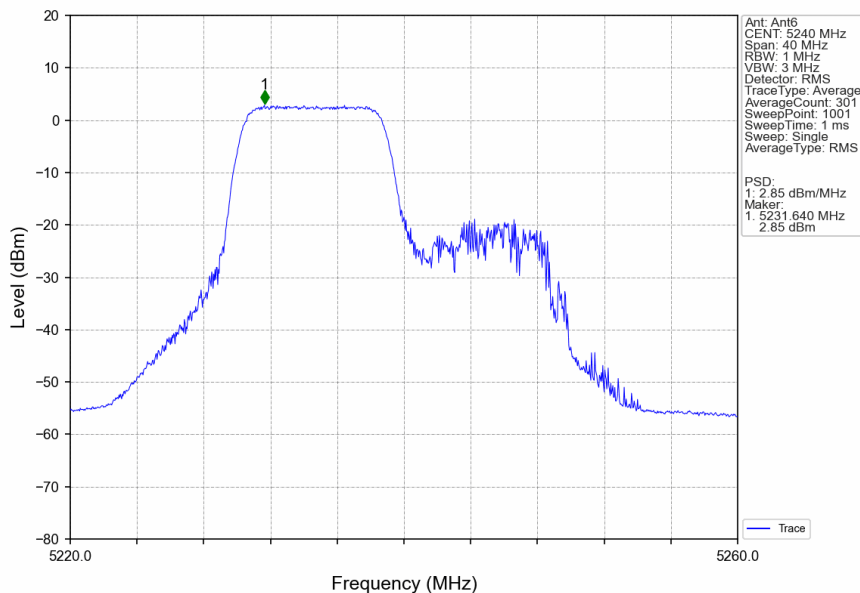
802.11ax(HEW20)_HCH_5240MHz_RU106_Left_Ant6_NTNV
