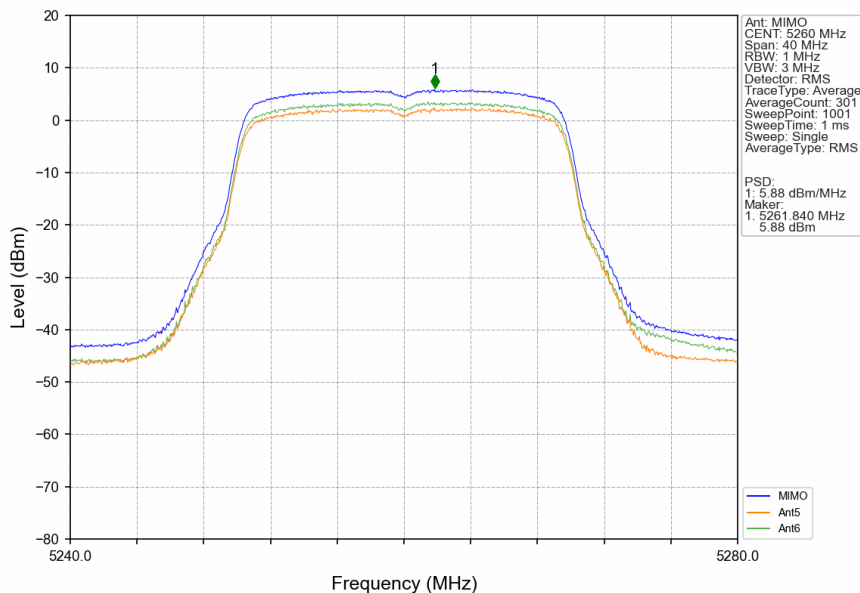
802.11ax(HEW20)_LCH_5260MHz_SU_/_MIMO_NTNV
