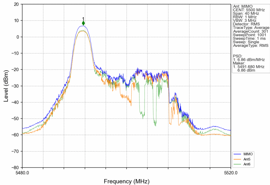
802.11ax(HEW20)_LCH_5500MHz_RU26_Left_MIMO_NTNV
