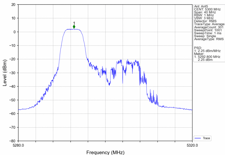
802.11ax(HEW20)_MCH_5300MHz_RU52_Left_Ant5_NTNV
