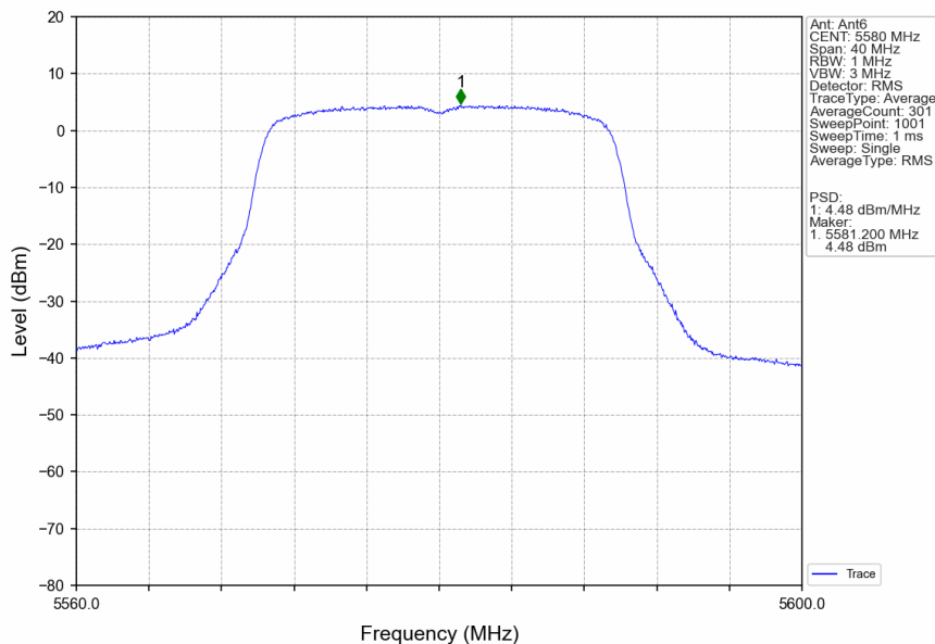
802.11ax(HEW20)_MCH_5580MHz_SU_/_Ant6_NTNV
