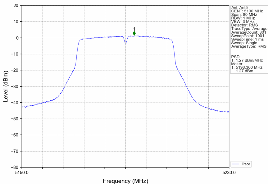
802.11ac(VHT40)_LCH_5190MHz_Ant5_NTNV
