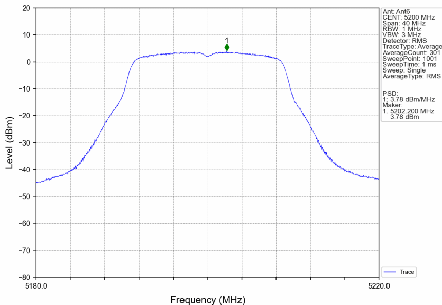
802.11ac(VHT20)_MCH_5200MHz_Ant6_NTNV
