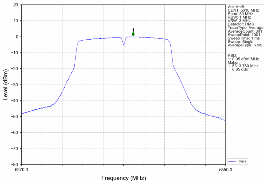
802.11ac(VHT40)_HCH_5310MHz_Ant5_NTNV
