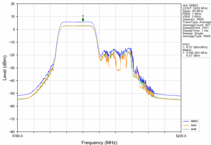
802.11ax(HEW20)_MCH_5200MHz_RU106_Left_MIMO_NTNV
