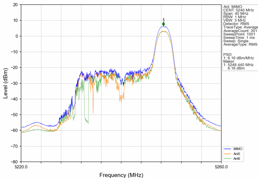
802.11ax(HEW20)_HCH_5240MHz_RU26_Right_MIMO_NTNV
