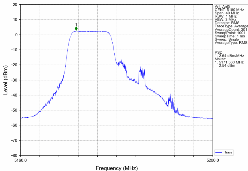
802.11ax(HEW20)_LCH_5180MHz_RU106_Left_Ant5_NTNV
