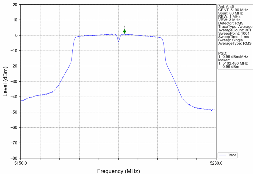
802.11ac(VHT40)_LCH_5190MHz_Ant6_NTNV
