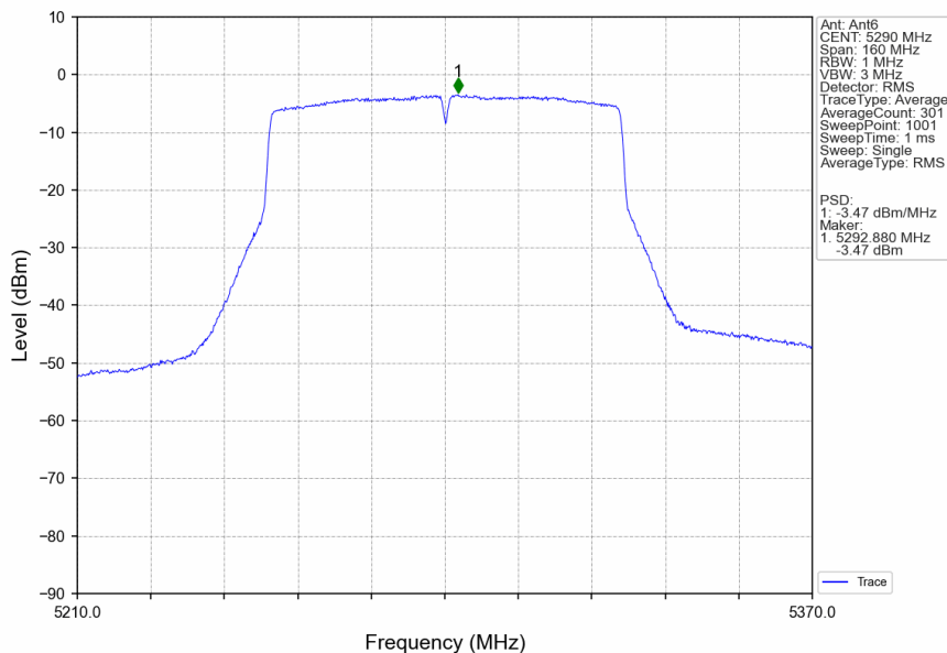
802.11ac(VHT80)_MCH_5290MHz_Ant6_NTNV
