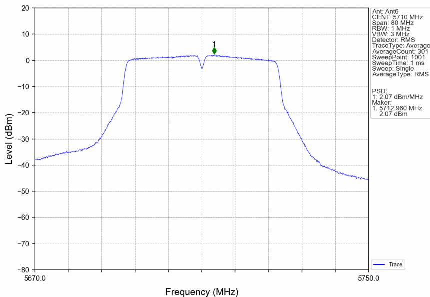
802.11ac(VHT40)_HCH_5710MHz_Ant6_NTNV
