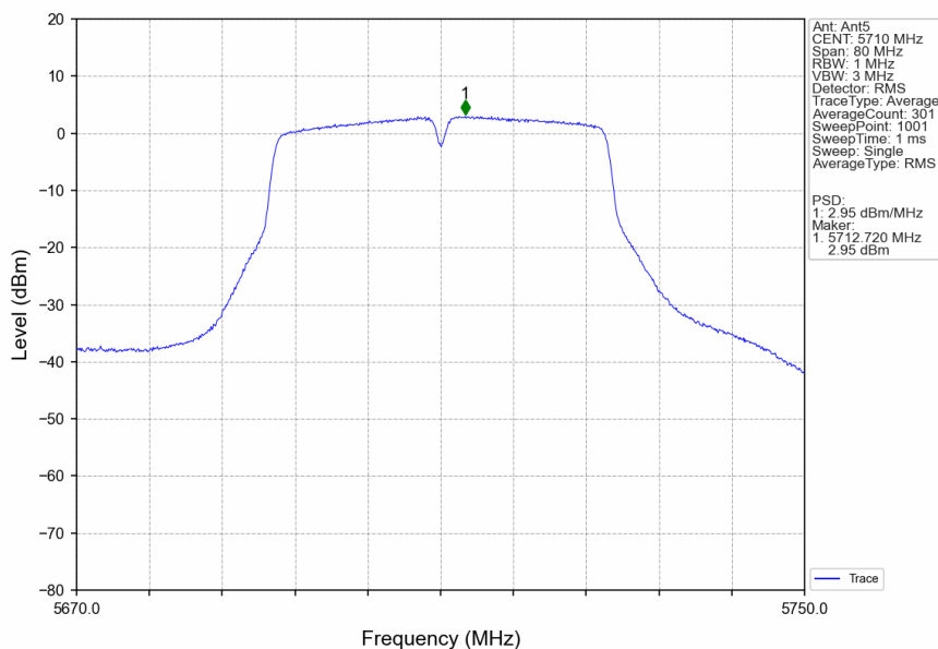
802.11ac(VHT40)_HCH_5710MHz_Ant5_NTNV
