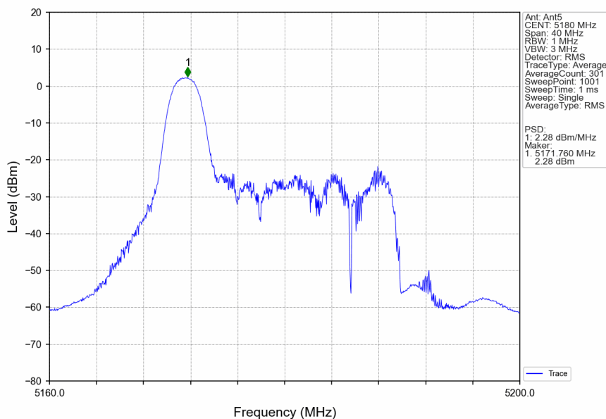
802.11ax(HEW20)_LCH_5180MHz_RU26_Left_Ant5_NTNV
