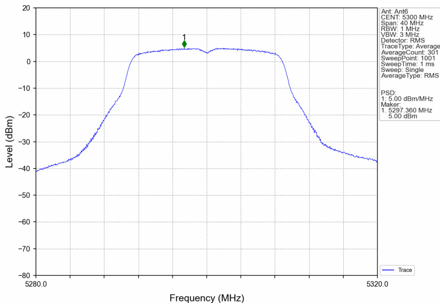
802.11ac(VHT20)_MCH_5300MHz_Ant6_NTNV
