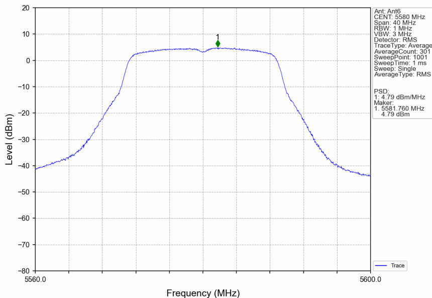
802.11ac(VHT20)_MCH_5580MHz_Ant6_NTNV
