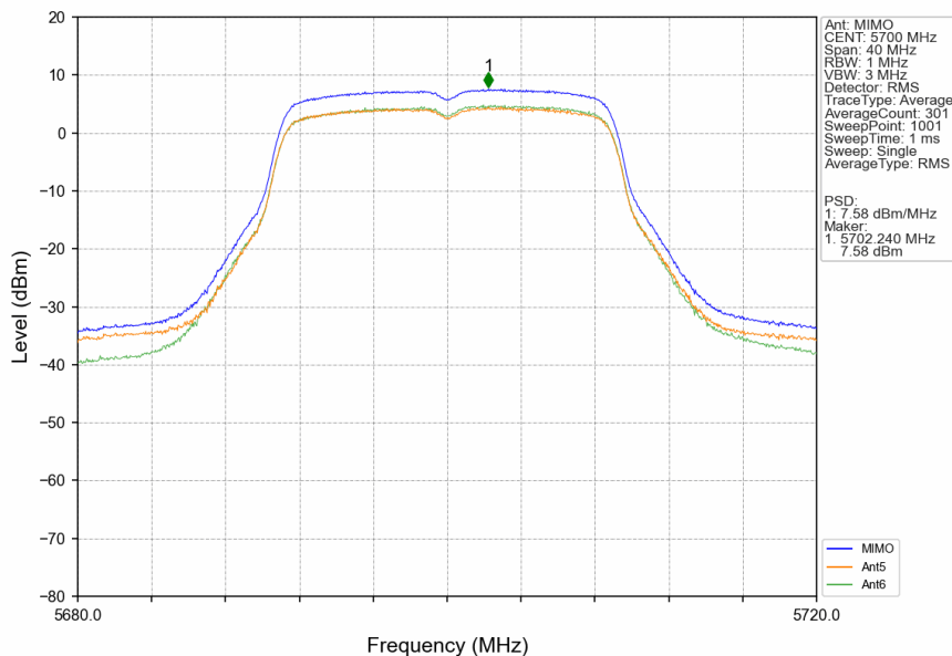
802.11ac(VHT20)_HCH_5700MHz_MIMO_NTNV
