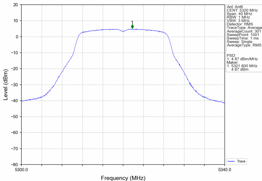
802.11ac(VHT20)_HCH_5320MHz_Ant6_NTNV
