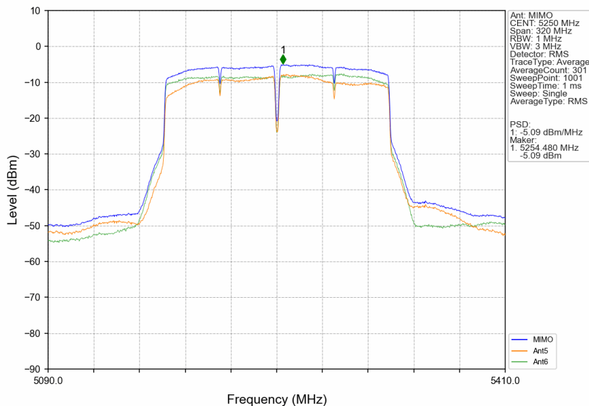
802.11ac(VHT160)_MCH_5250MHz_MIMO_NTNV
