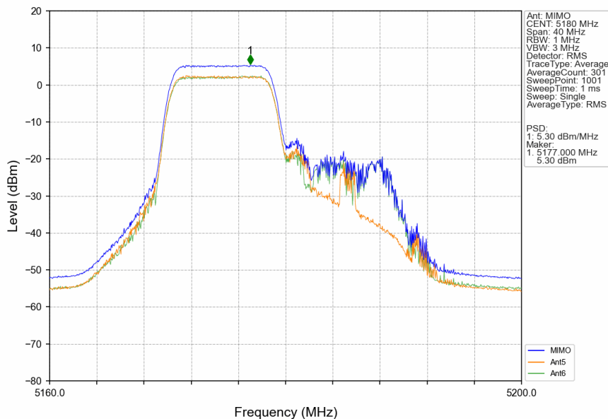
802.11ax(HEW20)_LCH_5180MHz_RU106_Left_MIMO_NTNV
