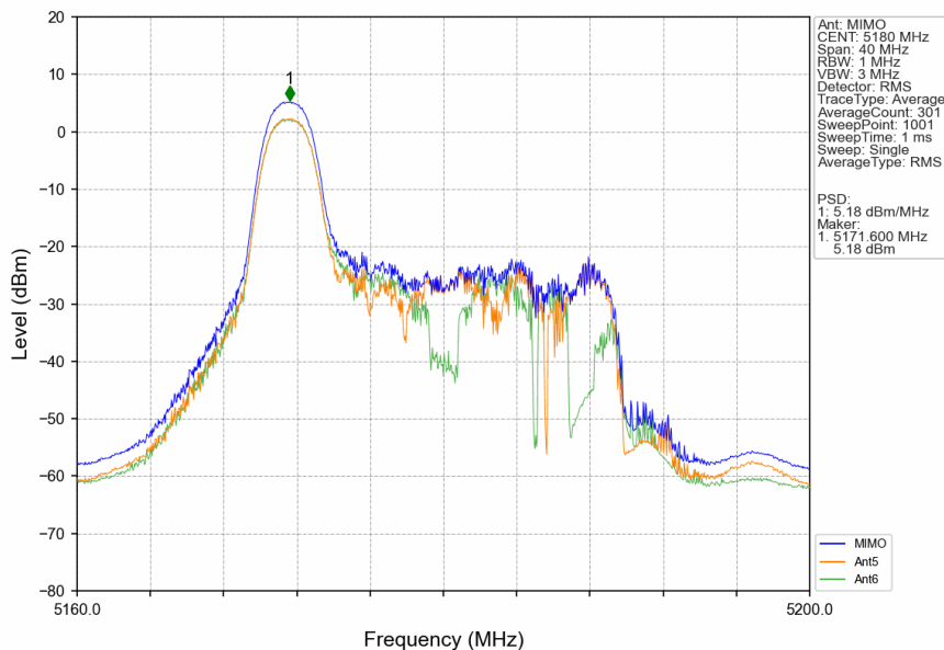
802.11ax(HEW20)_LCH_5180MHz_RU26_Left_MIMO_NTNV
