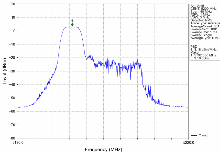
802.11ax(HEW20)_MCH_5200MHz_RU52_Left_Ant6_NTNV
