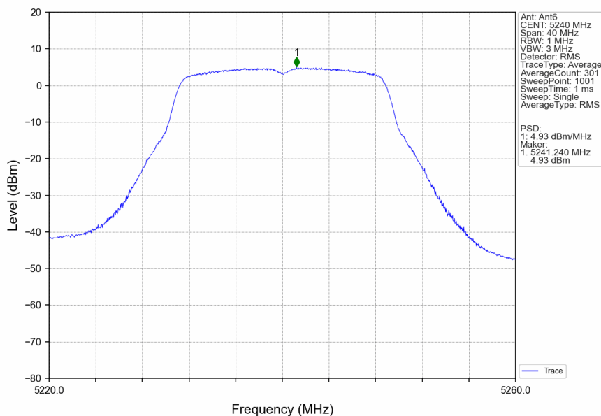
802.11ac(VHT20)_HCH_5240MHz_Ant6_NTNV
