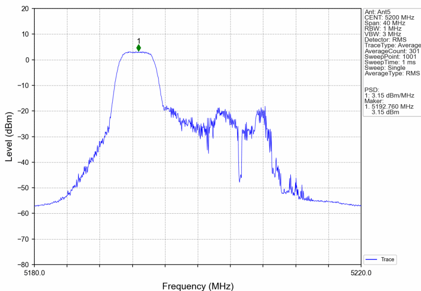
802.11ax(HEW20)_MCH_5200MHz_RU52_Left_Ant5_NTNV
