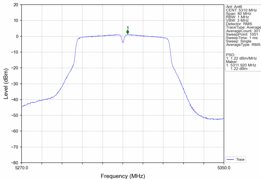
802.11ac(VHT40)_HCH_5310MHz_Ant6_NTNV
