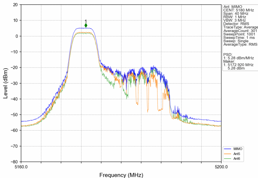
802.11ax(HEW20)_LCH_5180MHz_RU52_Left_MIMO_NTNV
