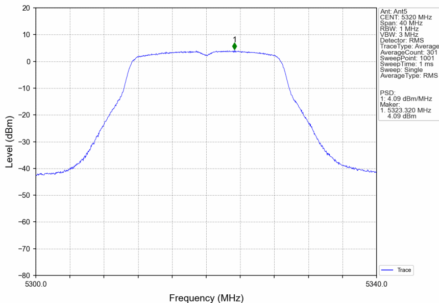
802.11ac(VHT20)_HCH_5320MHz_Ant5_NTNV
