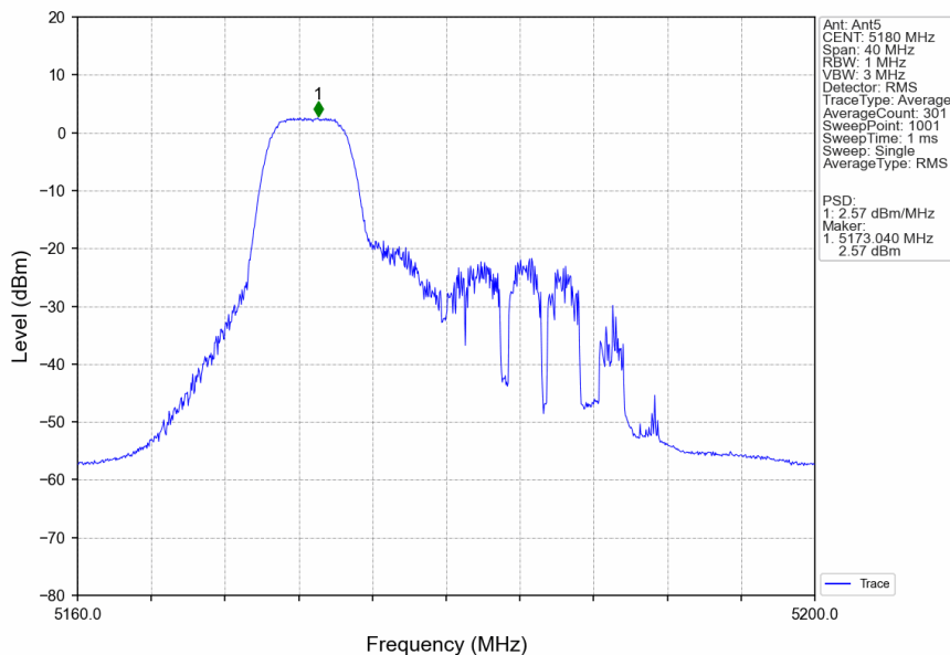
802.11ax(HEW20)_LCH_5180MHz_RU52_Left_Ant5_NTNV
