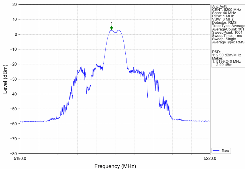
802.11ax(HEW20)_MCH_5200MHz_RU26_Mid_Ant5_NTNV
