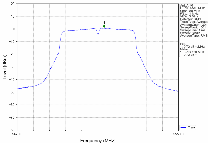
802.11ac(VHT40)_LCH_5510MHz_Ant6_NTNV
