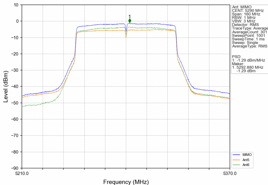
802.11ac(VHT80)_MCH_5290MHz_MIMO_NTNV
