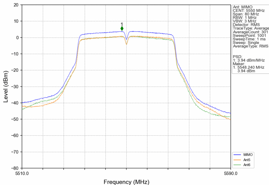
802.11ac(VHT40)_MCH_5550MHz_MIMO_NTNV
