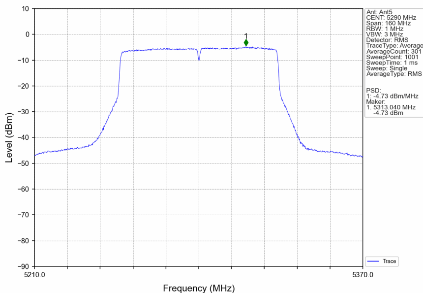
802.11ac(VHT80)_MCH_5290MHz_Ant5_NTNV
