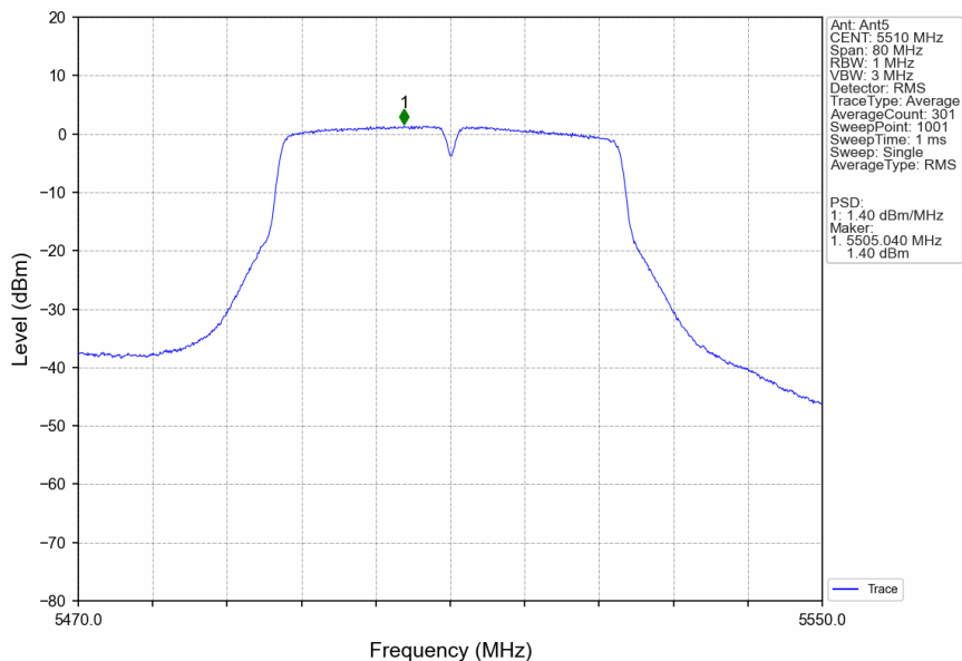
802.11ac(VHT40)_LCH_5510MHz_Ant5_NTNV
