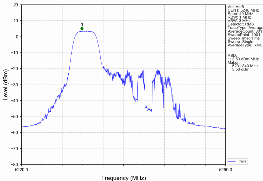
802.11ax(HEW20)_HCH_5240MHz_RU52_Left_Ant5_NTNV
