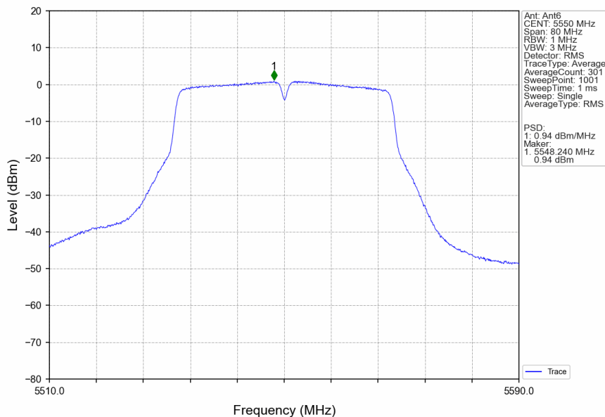
802.11ac(VHT40)_MCH_5550MHz_Ant6_NTNV
