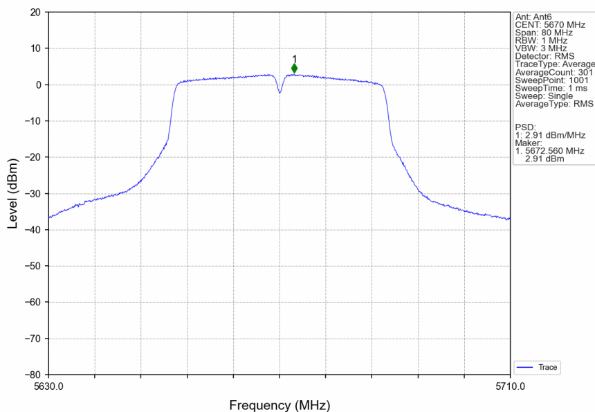
802.11ac(VHT40)_HCH_5670MHz_Ant6_NTNV
