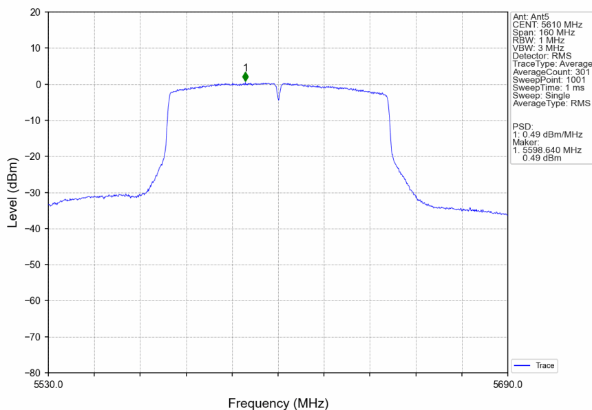
802.11ac(VHT80)_HCH_5610MHz_Ant5_NTNV
