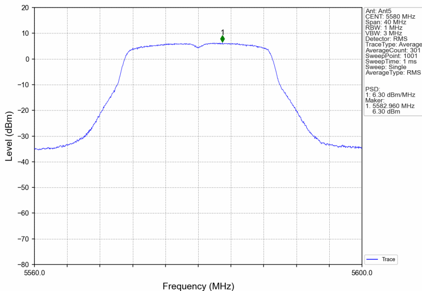
802.11ac(VHT20)_MCH_5580MHz_Ant5_NTNV
