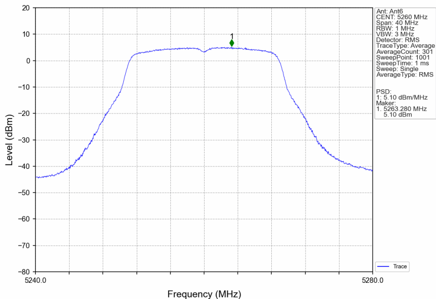
802.11ac(VHT20)_LCH_5260MHz_Ant6_NTNV
