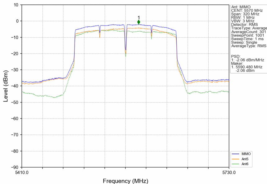
802.11ac(VHT160)_MCH_5570MHz_MIMO_NTNV
