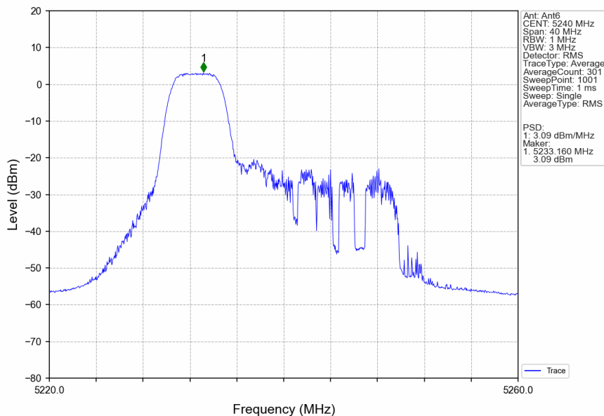
802.11ax(HEW20)_HCH_5240MHz_RU52_Left_Ant6_NTNV
