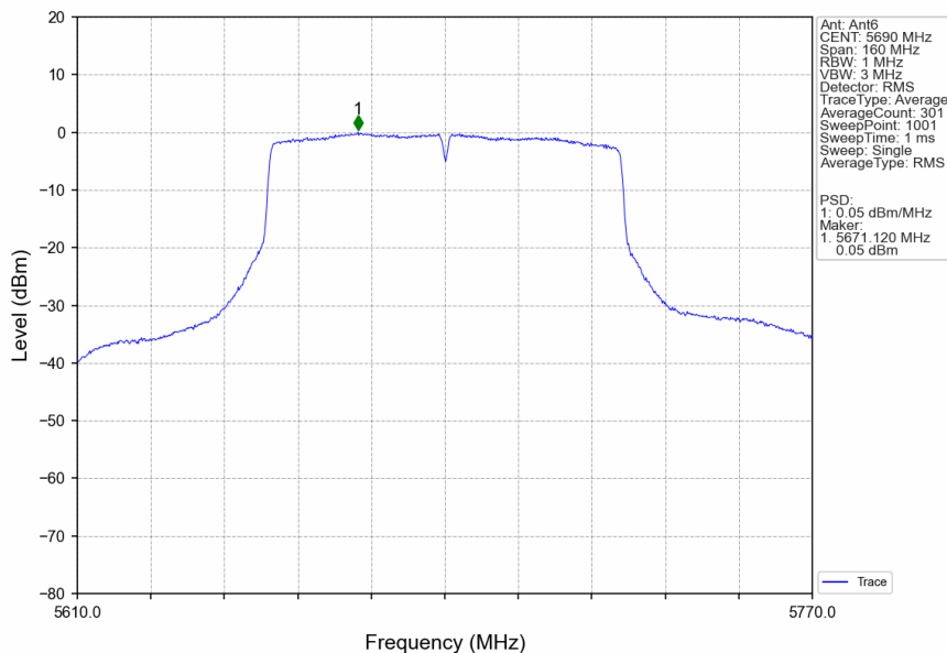
802.11ac(VHT80)_HCH_5690MHz_Ant6_NTNV
