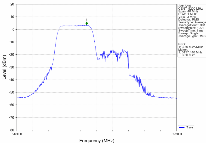
802.11ax(HEW20)_MCH_5200MHz_RU106_Left_Ant6_NTNV
