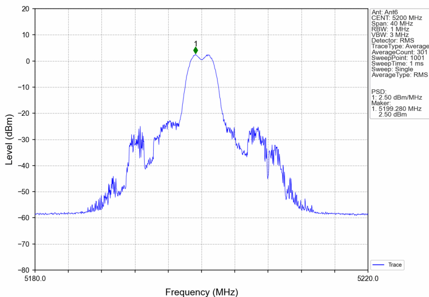
802.11ax(HEW20)_MCH_5200MHz_RU26_Mid_Ant6_NTNV
