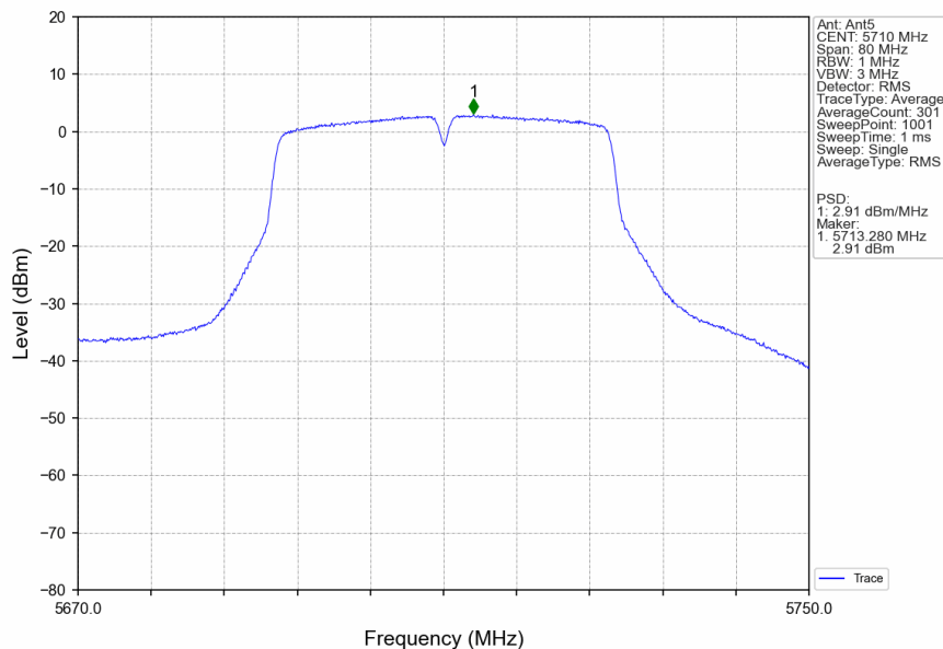
802.11n(HT40)_HCH_5710MHz_Ant5_NTNV
