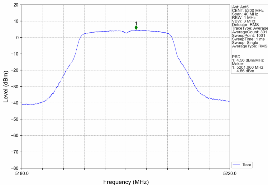
802.11n(HT20)_MCH_5200MHz_Ant5_NTNV
