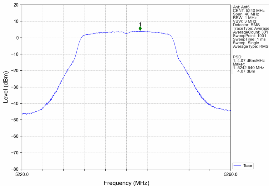
802.11n(HT20)_HCH_5240MHz_Ant5_NTNV
