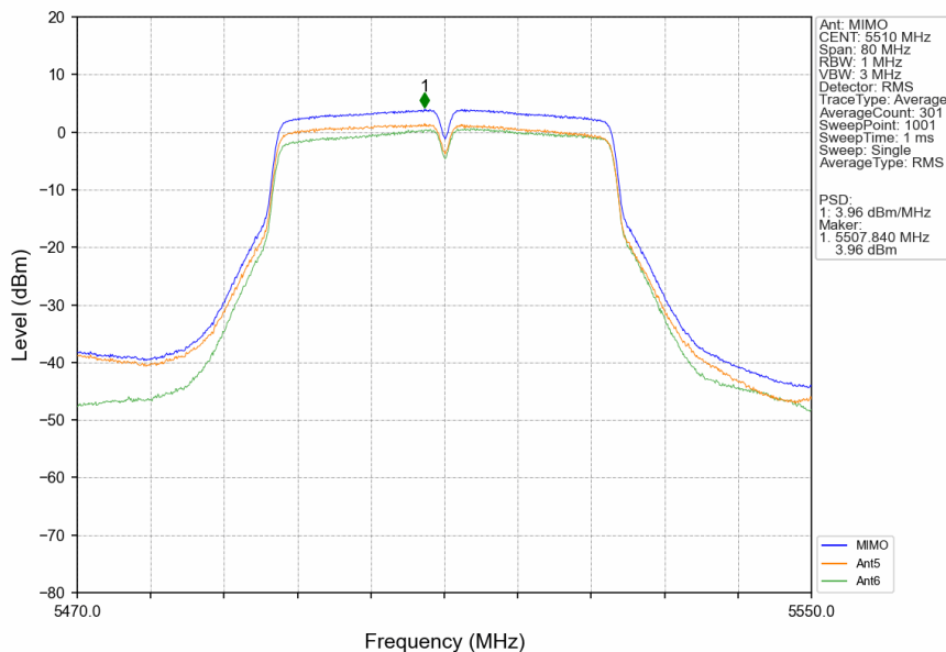
802.11n(HT40)_LCH_5510MHz_MIMO_NTNV
