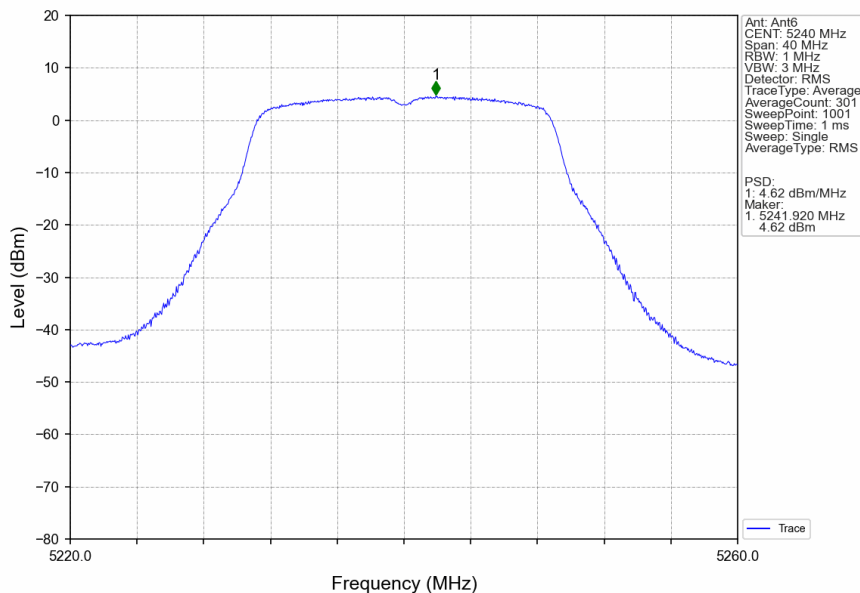
802.11n(HT20)_HCH_5240MHz_Ant6_NTNV
