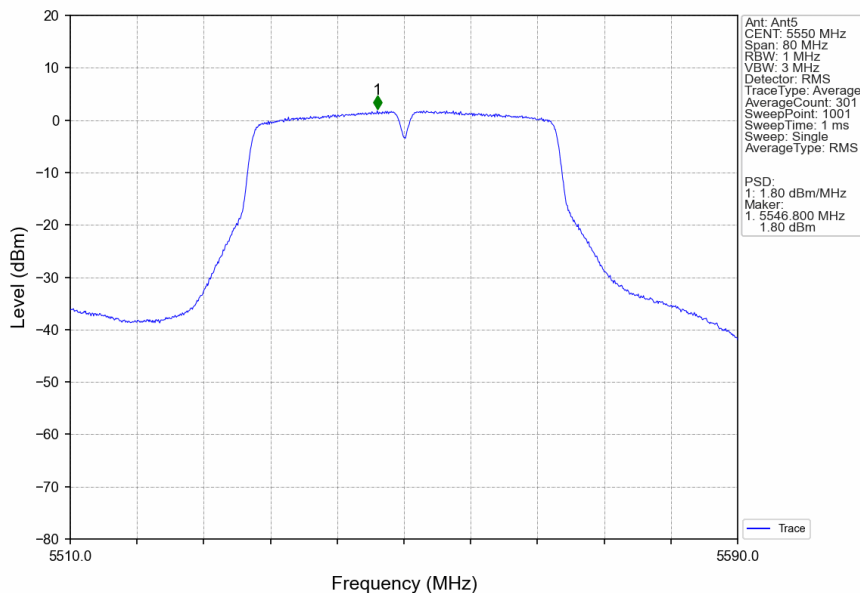
802.11n(HT40)_MCH_5550MHz_Ant5_NTNV
