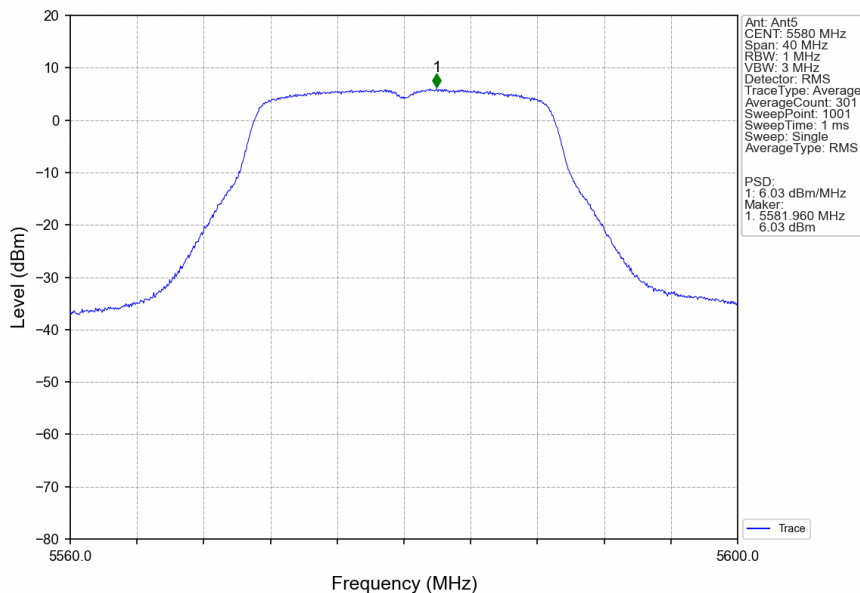
802.11n(HT20)_MCH_5580MHz_Ant5_NTNV
