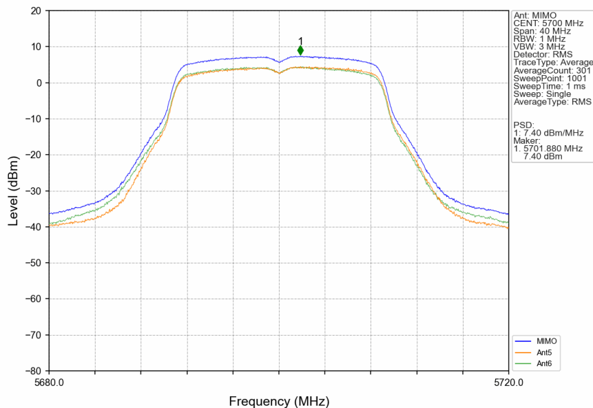
802.11n(HT20)_HCH_5700MHz_MIMO_NTNV
