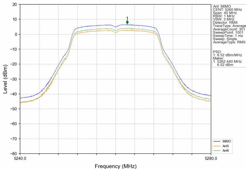
802.11n(HT20)_LCH_5260MHz_MIMO_NTNV
