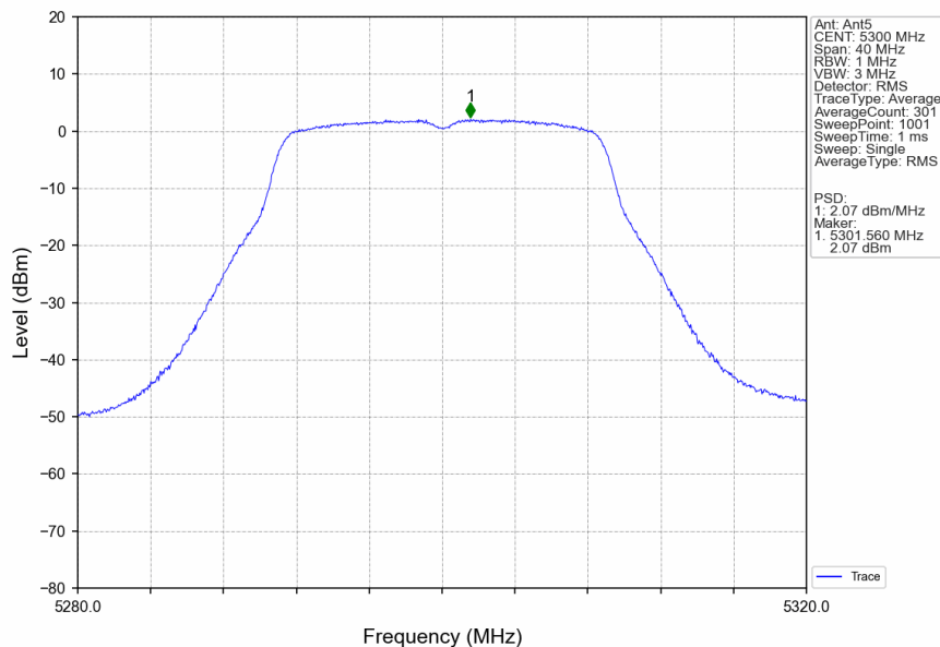
802.11n(HT20)_MCH_5300MHz_Ant5_NTNV
