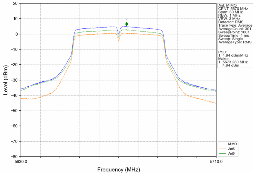
802.11n(HT40)_HCH_5670MHz_MIMO_NTNV
