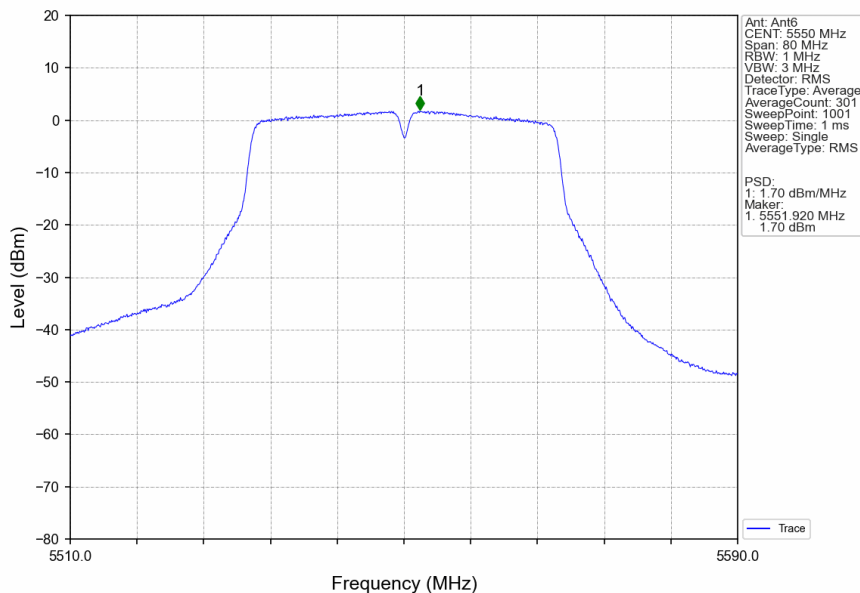
802.11n(HT40)_MCH_5550MHz_Ant6_NTNV
