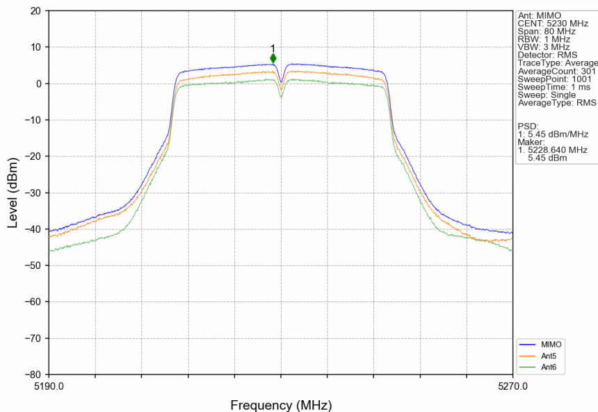
802.11n(HT40)_HCH_5230MHz_MIMO_NTNV
