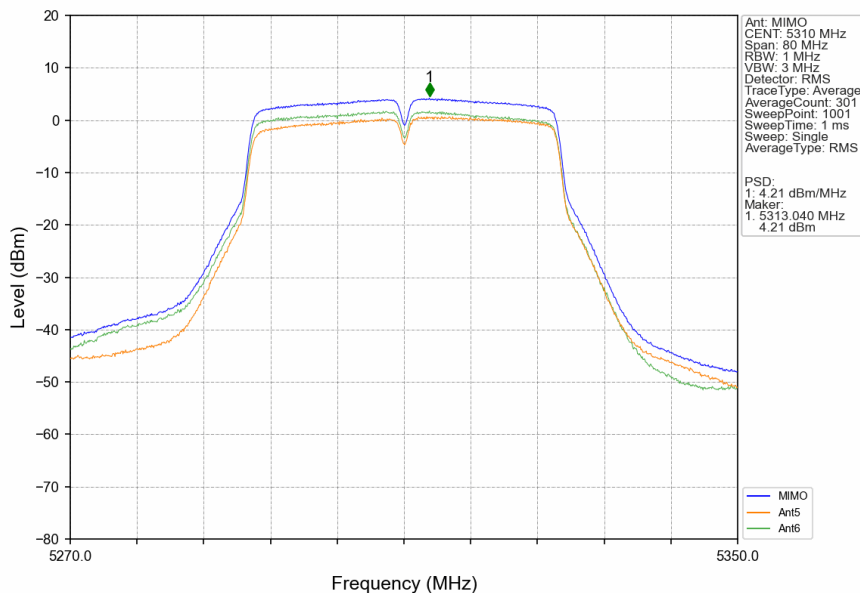
802.11n(HT40)_HCH_5310MHz_MIMO_NTNV
