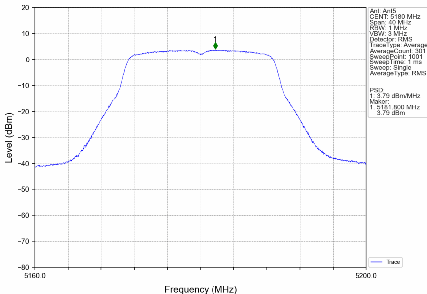
802.11ac(VHT20)_LCH_5180MHz_Ant5_NTNV
