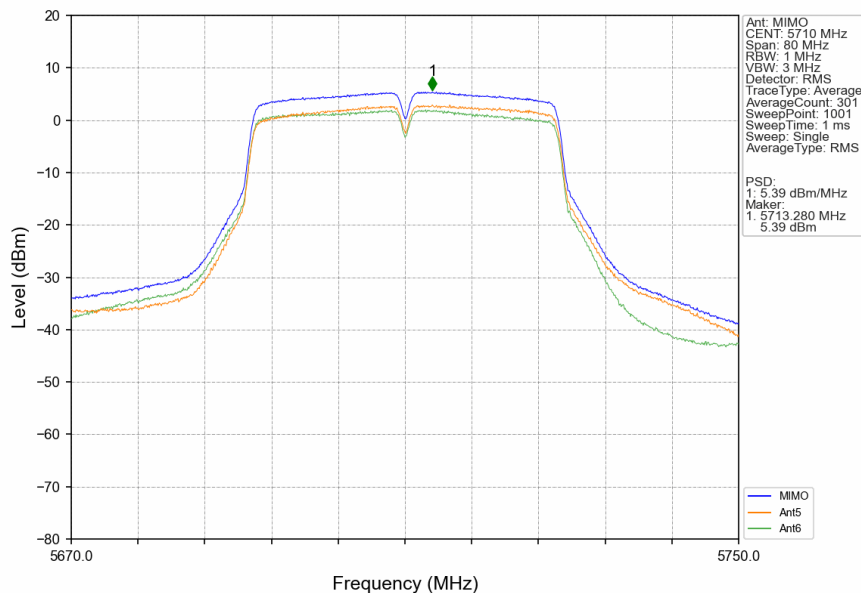
802.11n(HT40)_HCH_5710MHz_MIMO_NTNV
