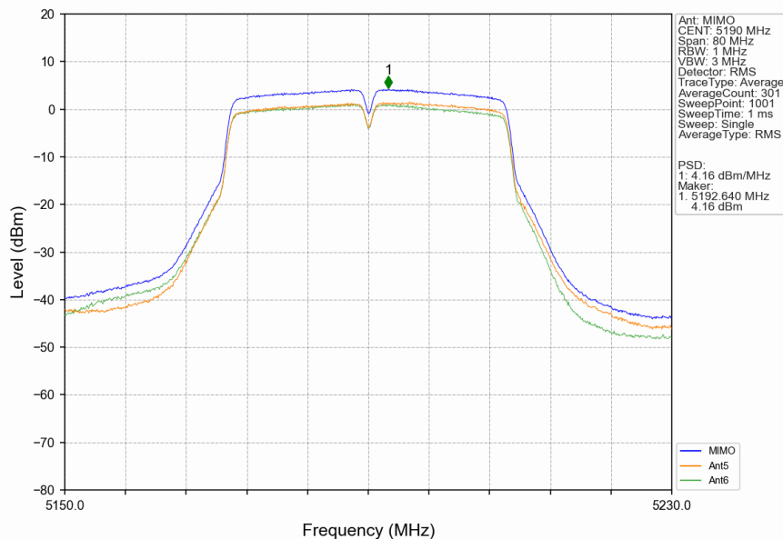
802.11n(HT40)_LCH_5190MHz_MIMO_NTNV
