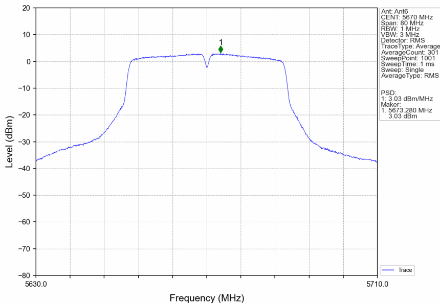
802.11n(HT40)_HCH_5670MHz_Ant6_NTNV
