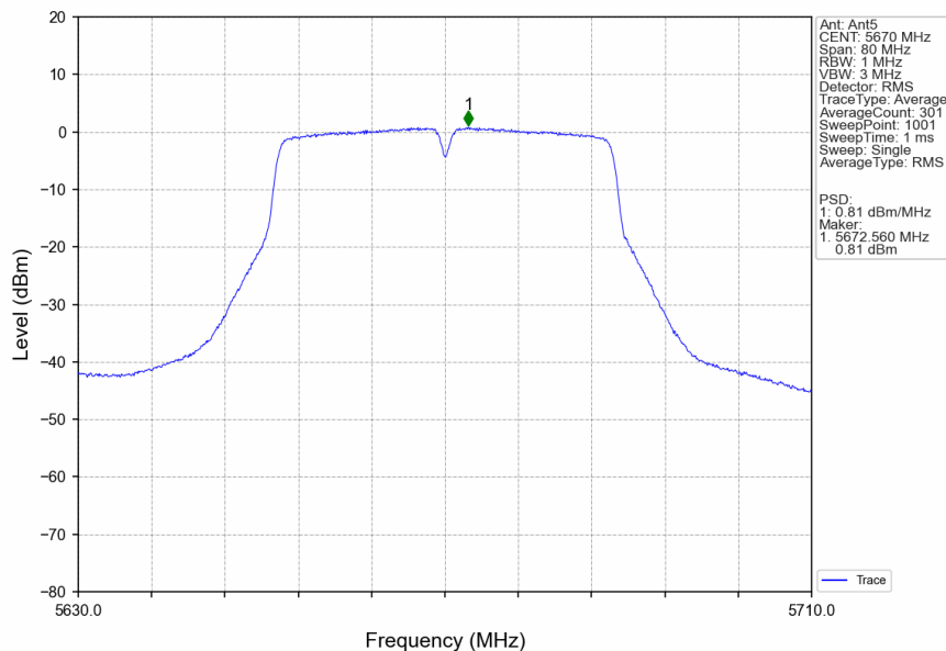
802.11n(HT40)_HCH_5670MHz_Ant5_NTNV
