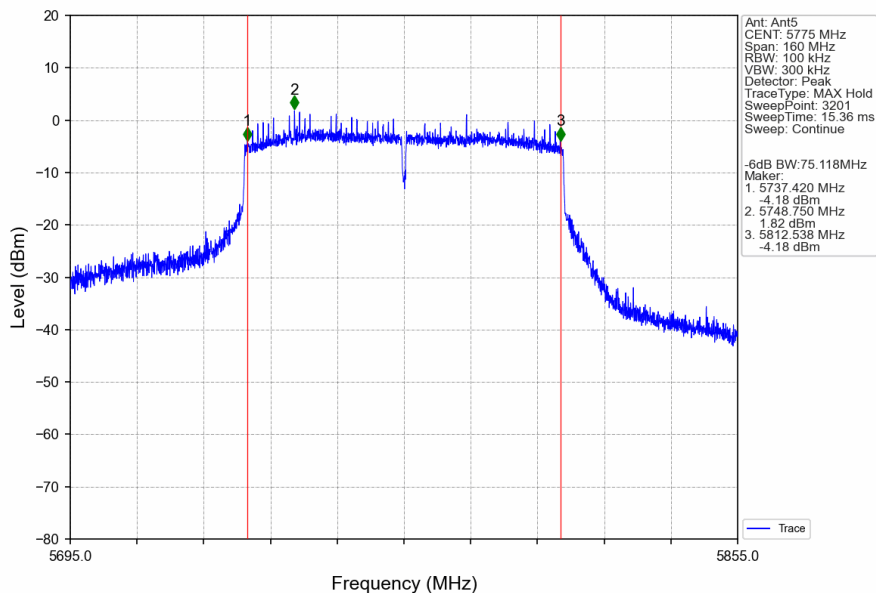
802.11ac(VHT80)_MCH_5775MHz_Ant5_NTNV
