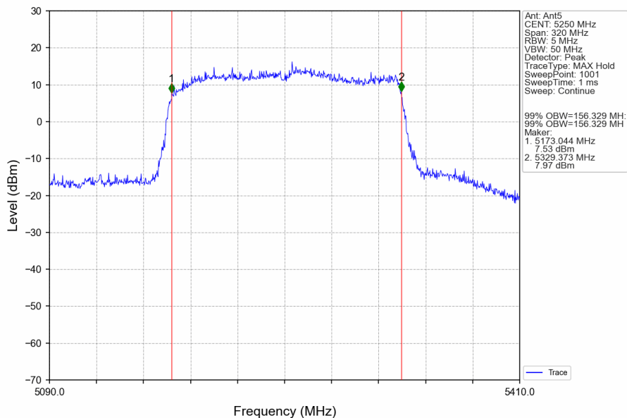
802.11ax(HEW160)_MCH_5250MHz_SU_/_Ant5_NTNV
