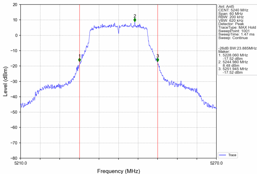
802.11n(HT20)_HCH_5240MHz_Ant5_NTNV
