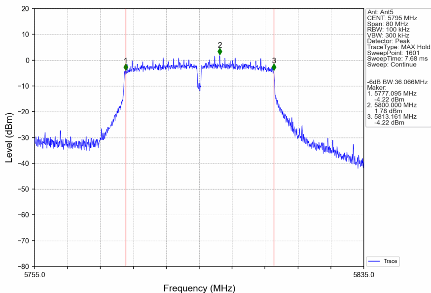
802.11n(HT40)_HCH_5795MHz_Ant5_NTNV
