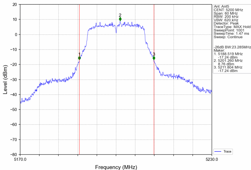
802.11n(HT20)_MCH_5200MHz_Ant5_NTNV
