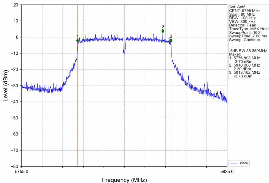
802.11ac(VHT40)_HCH_5795MHz_Ant5_NTNV
