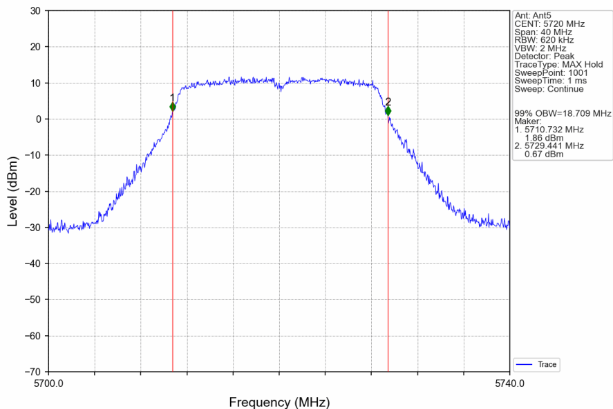
802.11ac(VHT20)_HCH_5720MHz_Ant5_NTNV
