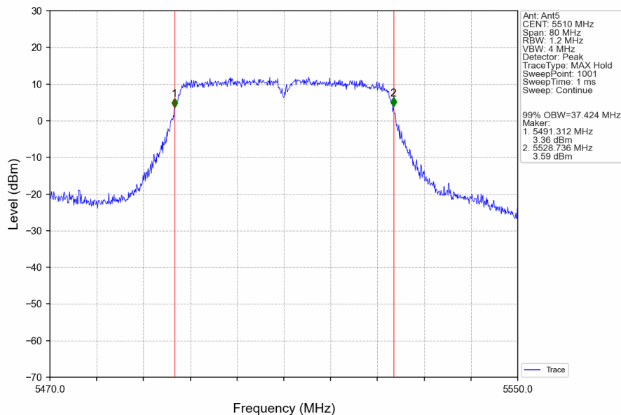
802.11ac(VHT40)_LCH_5510MHz_Ant5_NTNV
