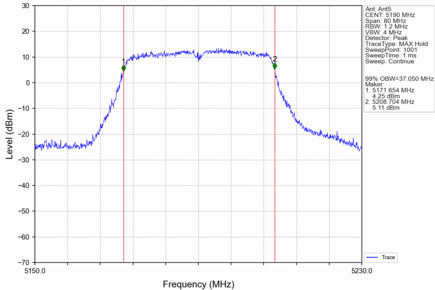
802.11ac(VHT40)_LCH_5190MHz_Ant5_NTNV
