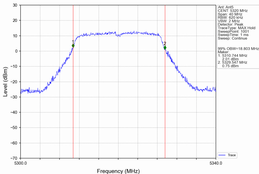
802.11ac(VHT20)_HCH_5320MHz_Ant5_NTNV
