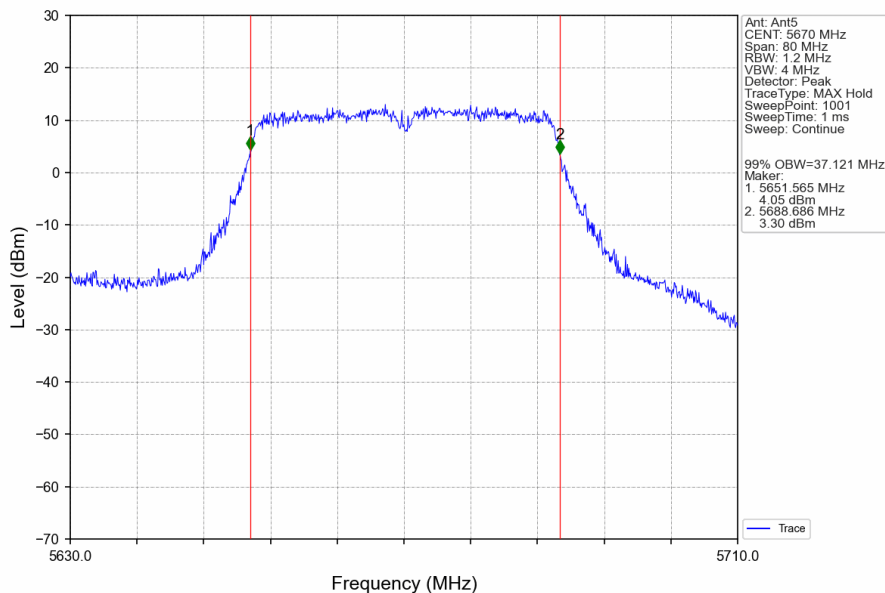
802.11ac(VHT40)_HCH_5670MHz_Ant5_NTNV
