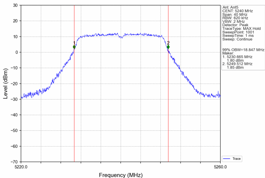
802.11ac(VHT20)_HCH_5240MHz_Ant5_NTNV
