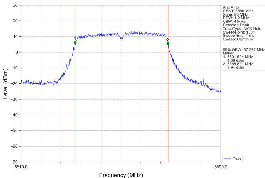
802.11ac(VHT40)_MCH_5550MHz_Ant5_NTNV
