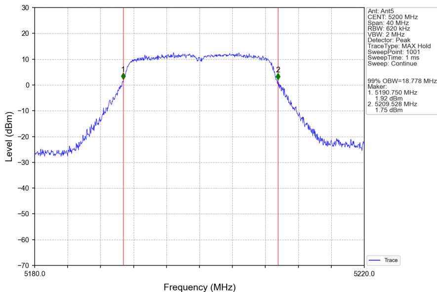
802.11ac(VHT20)_MCH_5200MHz_Ant5_NTNV
