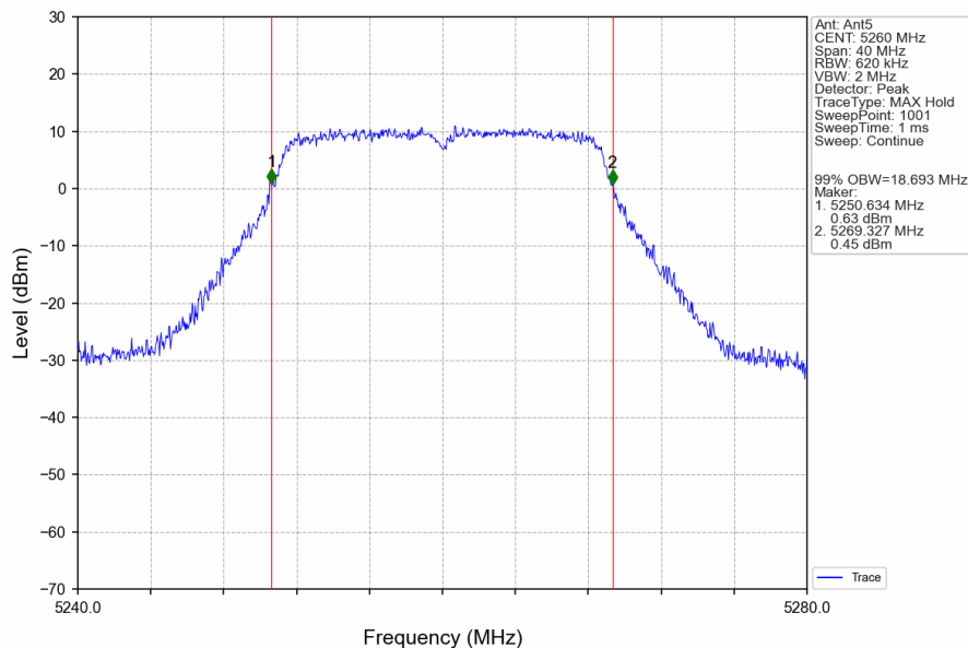
802.11n(HT20)_LCH_5260MHz_Ant5_NTNV
