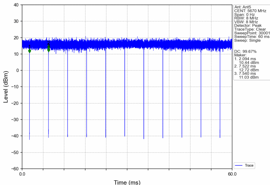
802.11ac(VHT40)_HCH_5670MHz_Ant5_NTNV
