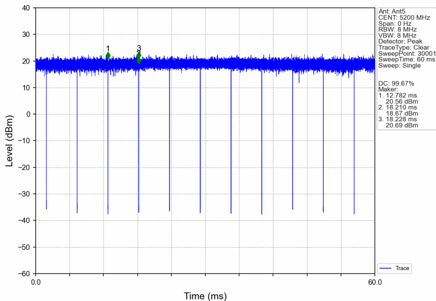
802.11ac(VHT20)_MCH_5200MHz_Ant5_NTNV
