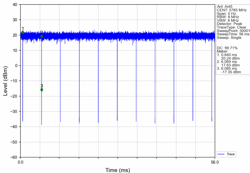
802.11n(HT20)_MCH_5785MHz_Ant5_NTNV
