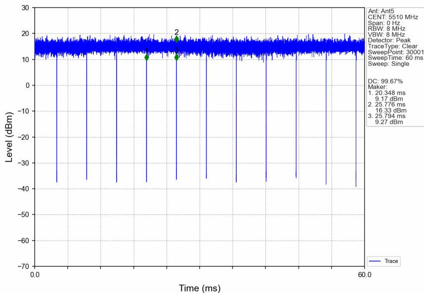
802.11ac(VHT40)_LCH_5510MHz_Ant5_NTNV
