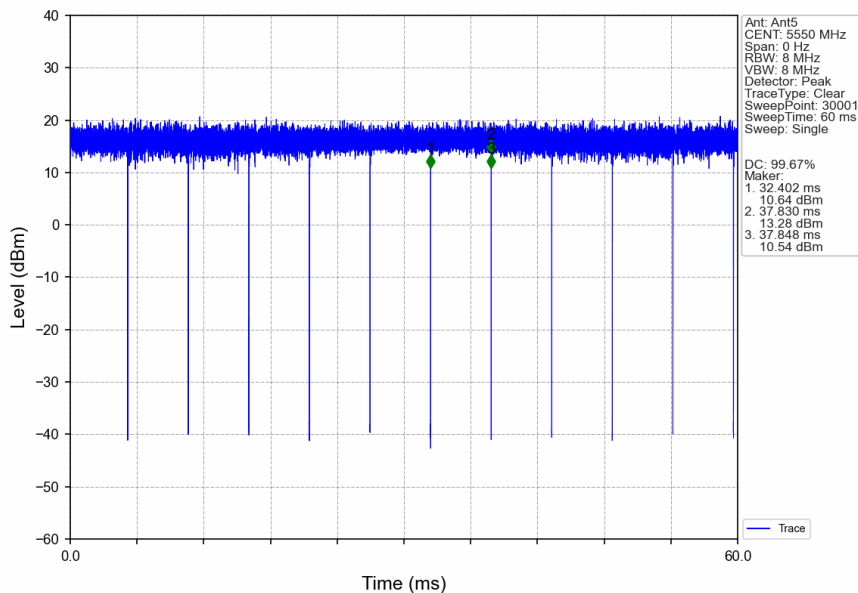
802.11ac(VHT40)_MCH_5550MHz_Ant5_NTNV
