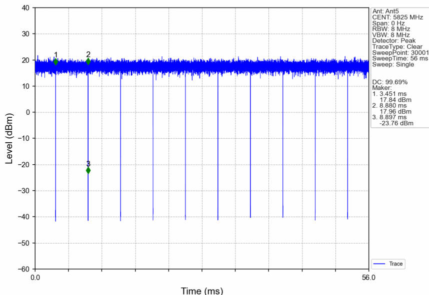
802.11n(HT20)_HCH_5825MHz_Ant5_NTNV
