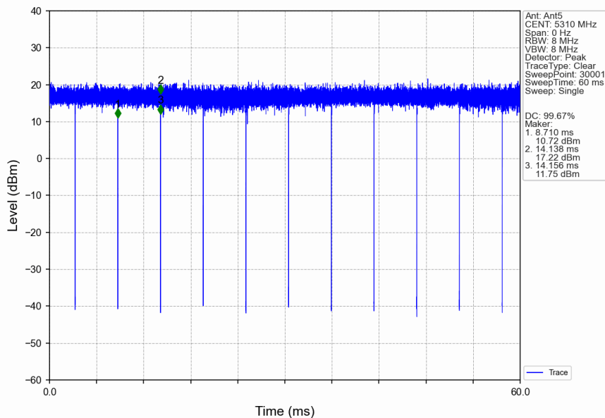
802.11n(HT40)_HCH_5310MHz_Ant5_NTNV
