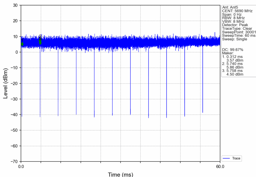
802.11ac(VHT80)_HCH_5690MHz_Ant5_NTNV
