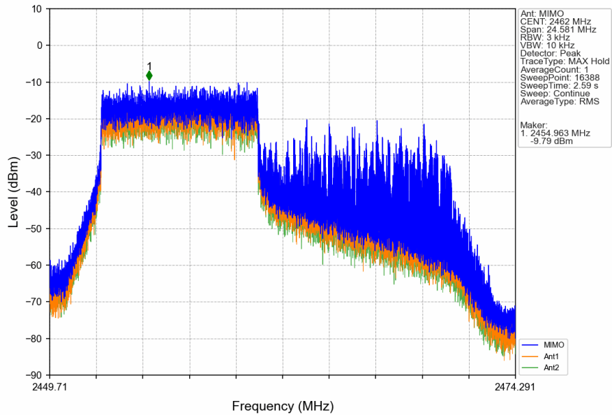
802.11ax(HEW20)_HCH_2462MHz_RU106_Left_MIMO_NTNV
