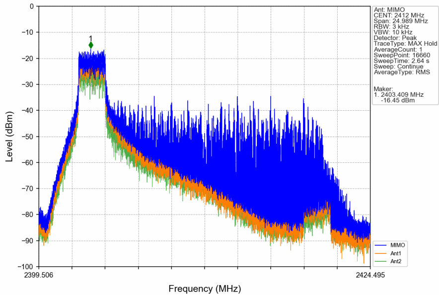
802.11ax(HEW20)_LCH_2412MHz_RU26_Left_MIMO_NTNV
