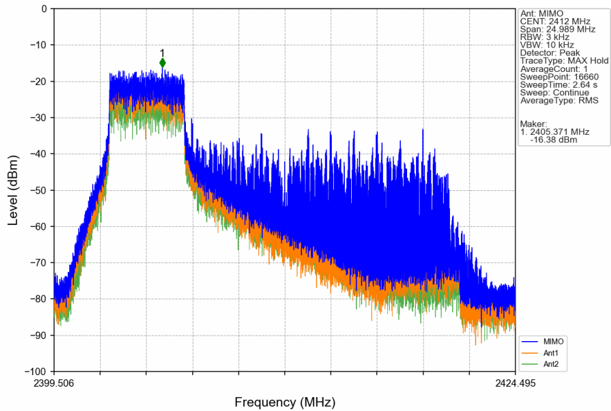
802.11ax(HEW20)_LCH_2412MHz_RU52_Left_MIMO_NTNV
