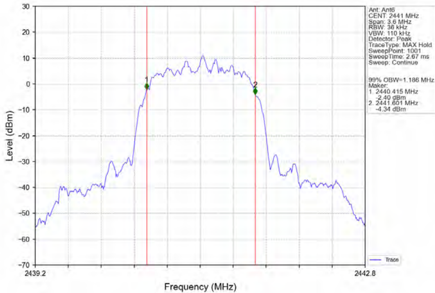
Pi/4DQPSK_2DH5_MCH_2441MHz_Ant6_NTNV
