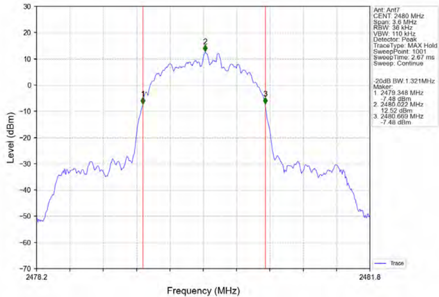
8DPSK_3DH5_HCH_2480MHz_Ant7_NTNV
