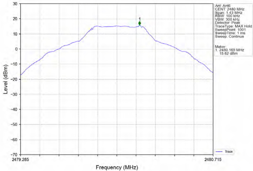
GFSK_DH5_HCH_2480MHz_Ant6_NTNV
