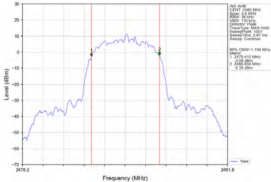
8DPSK_3DH5_HCH_2480MHz_Ant6_NTNV
