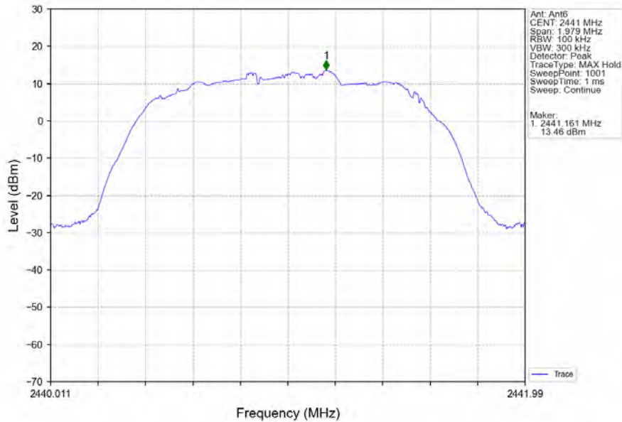
8DPSK_3DH5_MCH_2441MHz_Ant6_NTNV
