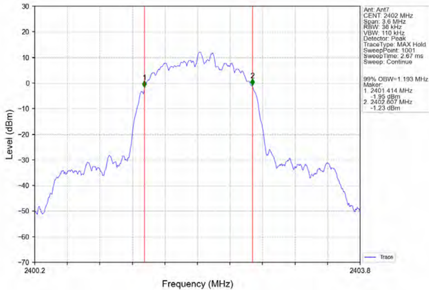
8DPSK_3DH5_LCH_2402MHz_Ant7_NTNV
