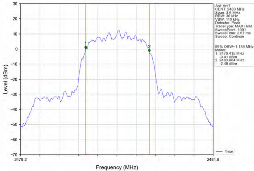
Pi/4DQPSK_2DH5_HCH_2480MHz_Ant7_NTNV
