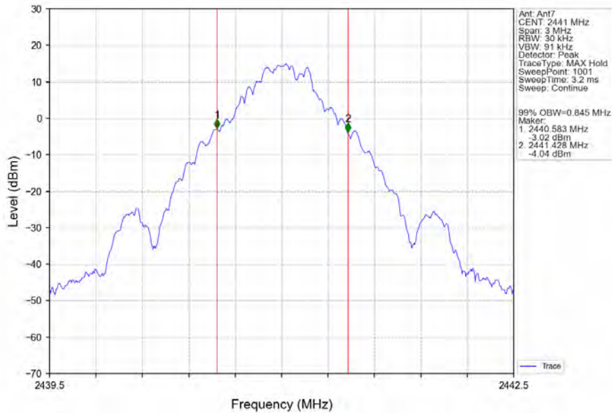
GFSK_DH5_MCH_2441MHz_Ant7_NTNV
