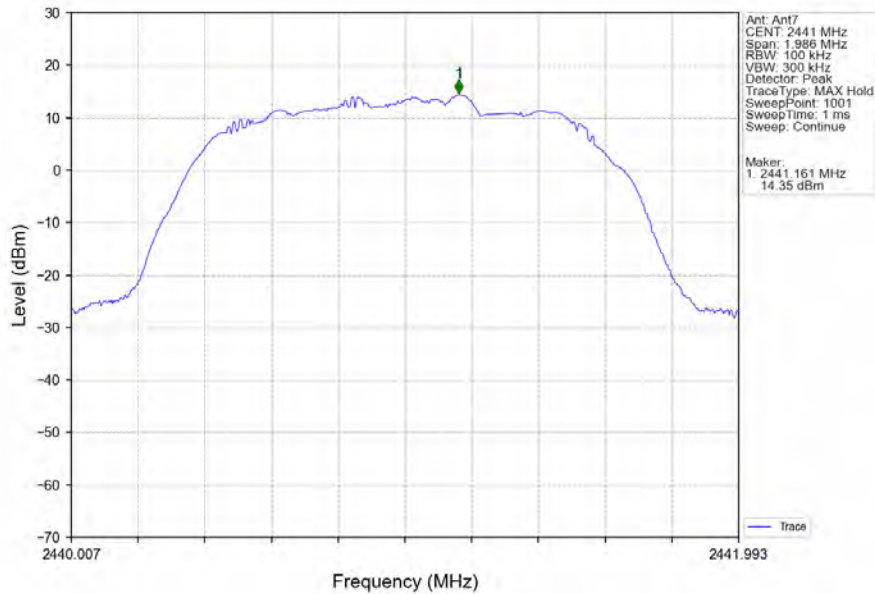
8DPSK_3DH5_MCH_2441MHz_Ant7_NTNV
