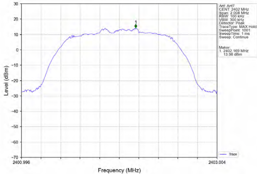
Pi/4DQPSK_2DH5_LCH_2402MHz_Ant7_NTNV
