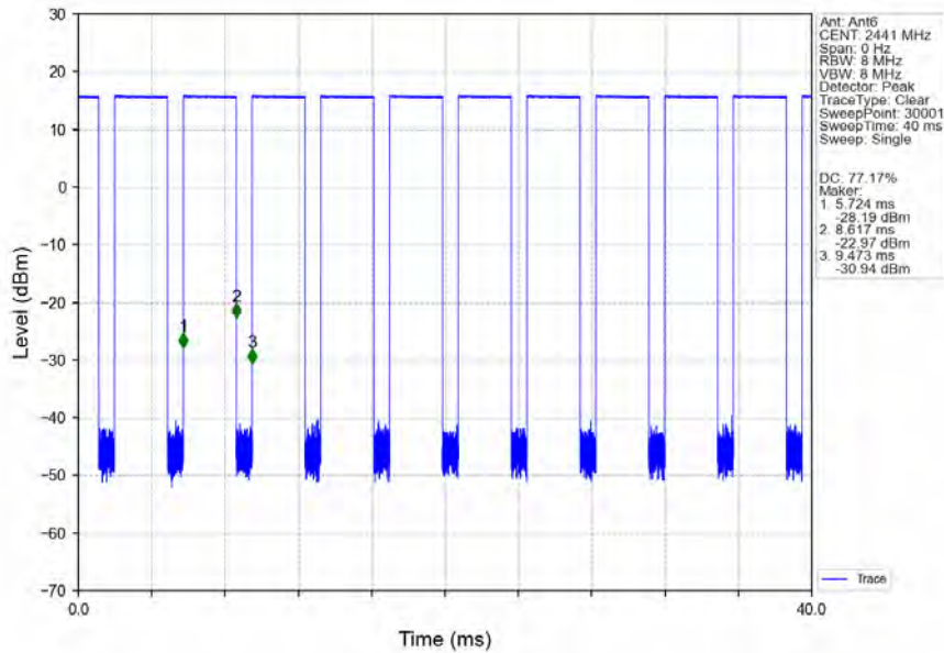
GFSK_DH5_MCH_2441MHz_Ant6_NTNV
