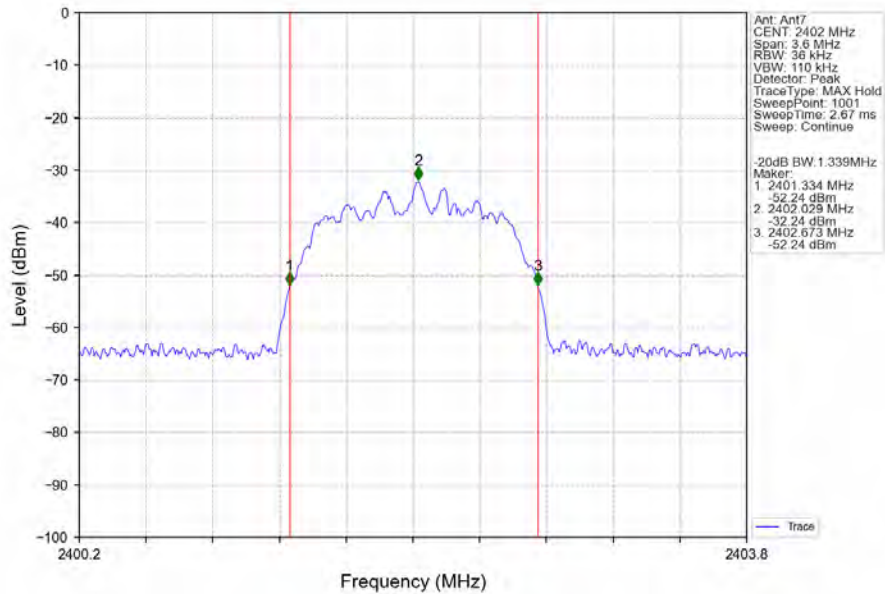
Pi/4DQPSK_2DH5_LCH_2402MHz_Ant7_NTNV
