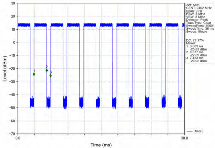
Pi/4DQPSK_2DH5_LCH_2402MHz_Ant6_NTNV
