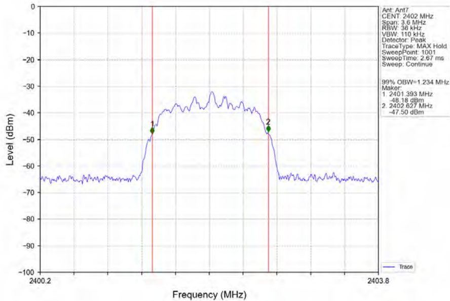
Pi/4DQPSK_2DH5_LCH_2402MHz_Ant7_NTNV
