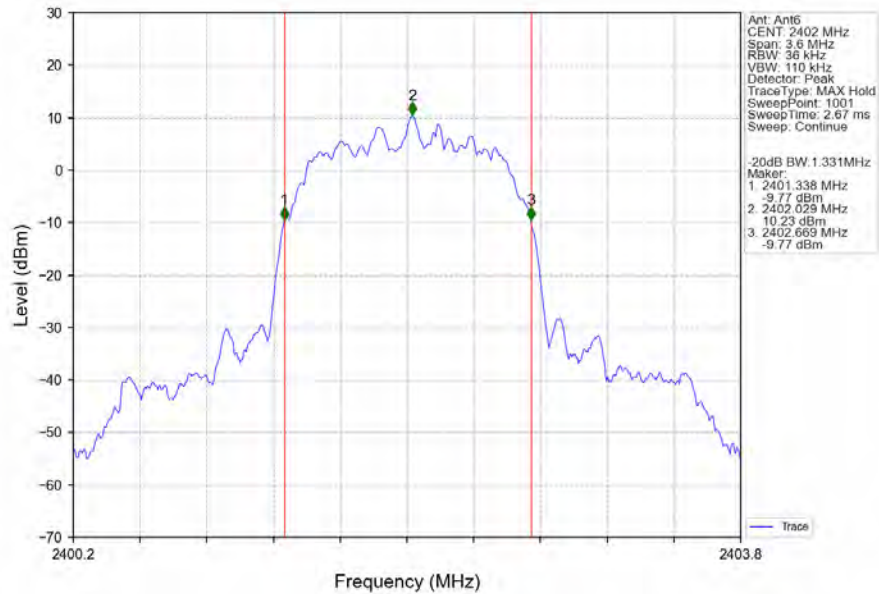
Pi/4DQPSK_2DH5_LCH_2402MHz_Ant6_NTNV
