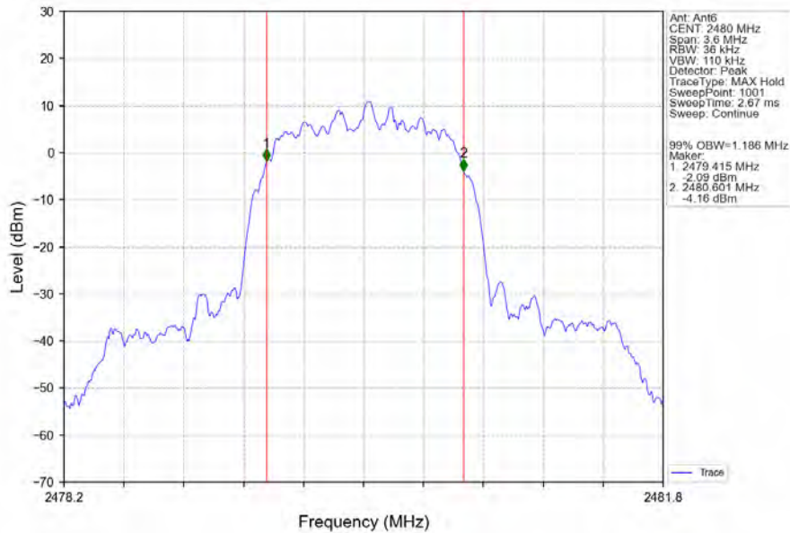
Pi/4DQPSK_2DH5_HCH_2480MHz_Ant6_NTNV
