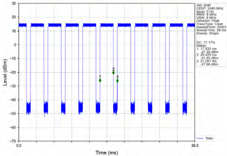
Pi/4DQPSK_2DH5_HCH_2480MHz_Ant6_NTNV
