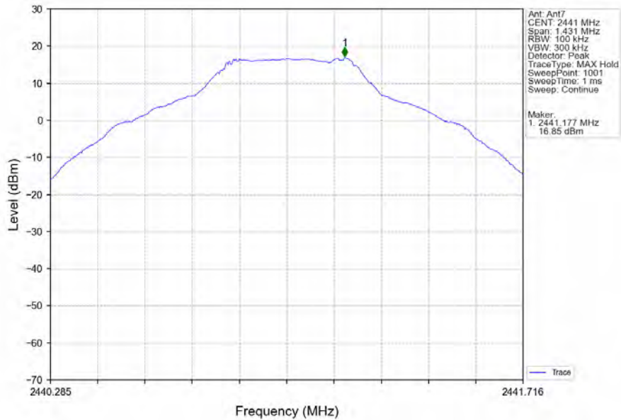
GFSK_DH5_MCH_2441MHz_Ant7_NTNV
