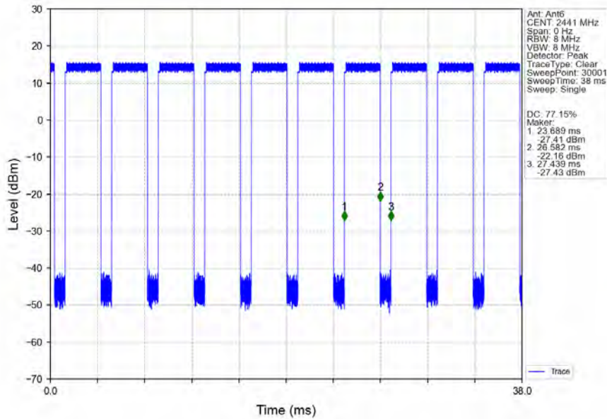
Pi/4DQPSK_2DH5_MCH_2441MHz_Ant6_NTNV
