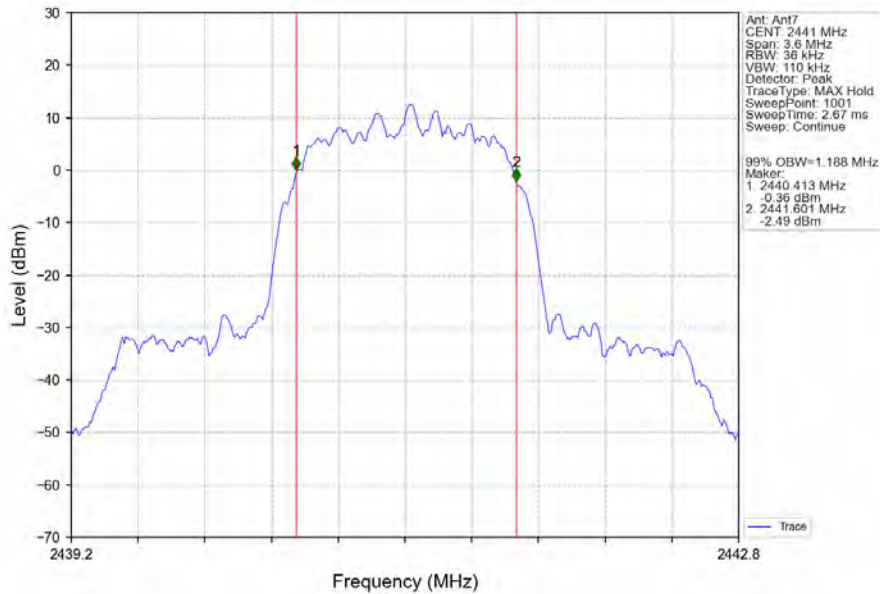
Pi/4DQPSK_2DH5_MCH_2441MHz_Ant7_NTNV
