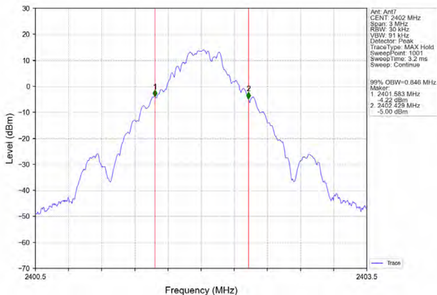
GFSK_DH5_LCH_2402MHz_Ant7_NTNV
