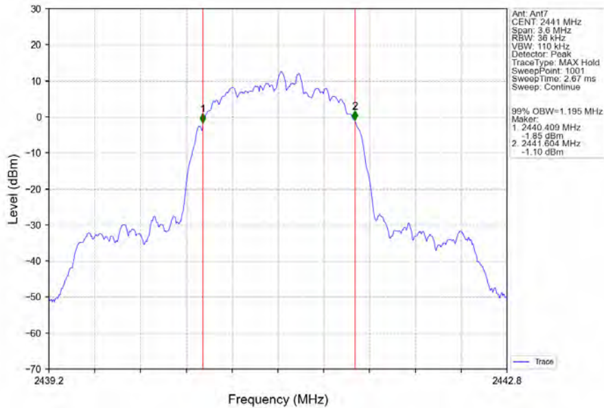
8DPSK_3DH5_MCH_2441MHz_Ant7_NTNV
