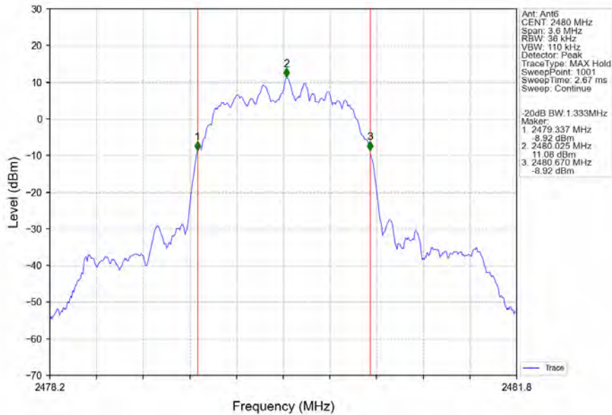
Pi/4DQPSK_2DH5_HCH_2480MHz_Ant6_NTNV
