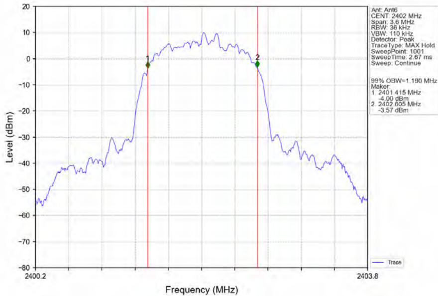
8DPSK_3DH5_LCH_2402MHz_Ant6_NTNV
