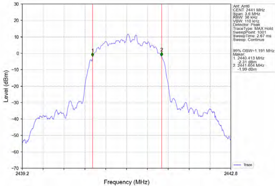
8DPSK_3DH5_MCH_2441MHz_Ant6_NTNV
