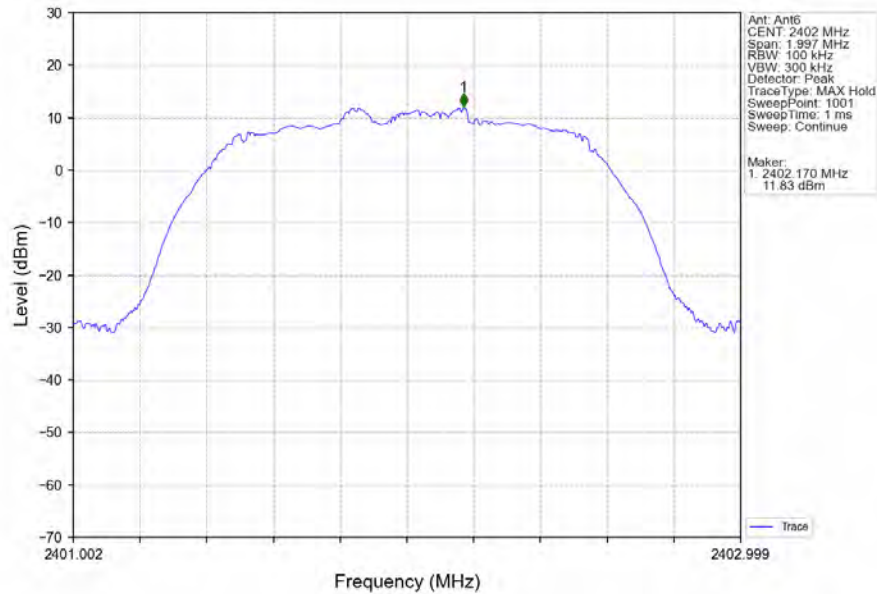
Pi/4DQPSK_2DH5_LCH_2402MHz_Ant6_NTNV
