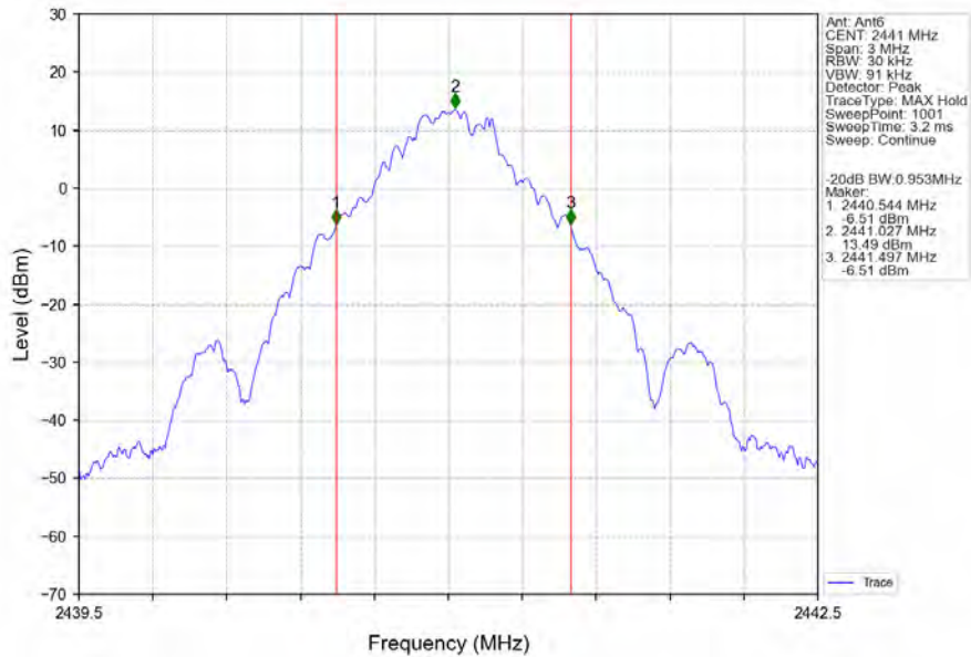
GFSK_DH5_MCH_2441MHz_Ant6_NTNV
