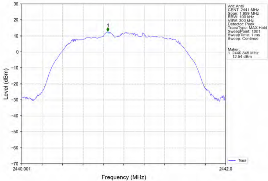
Pi/4DQPSK_2DH5_MCH_2441MHz_Ant6_NTNV
