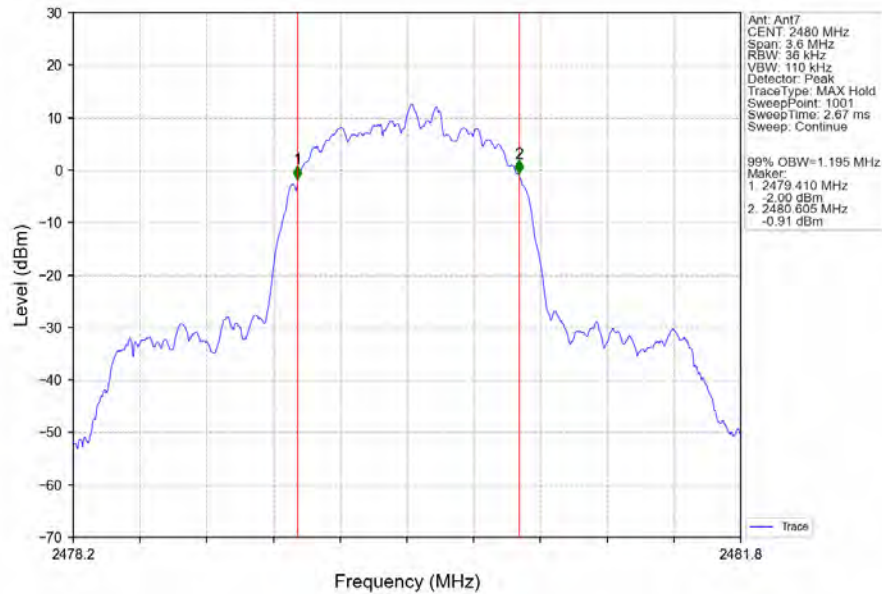
8DPSK_3DH5_HCH_2480MHz_Ant7_NTNV
