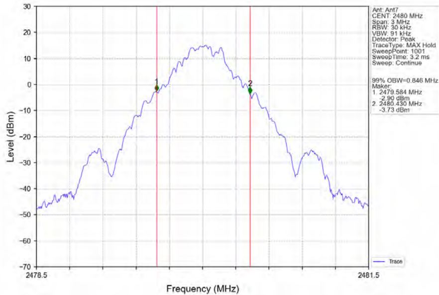
GFSK_DH5_HCH_2480MHz_Ant7_NTNV
