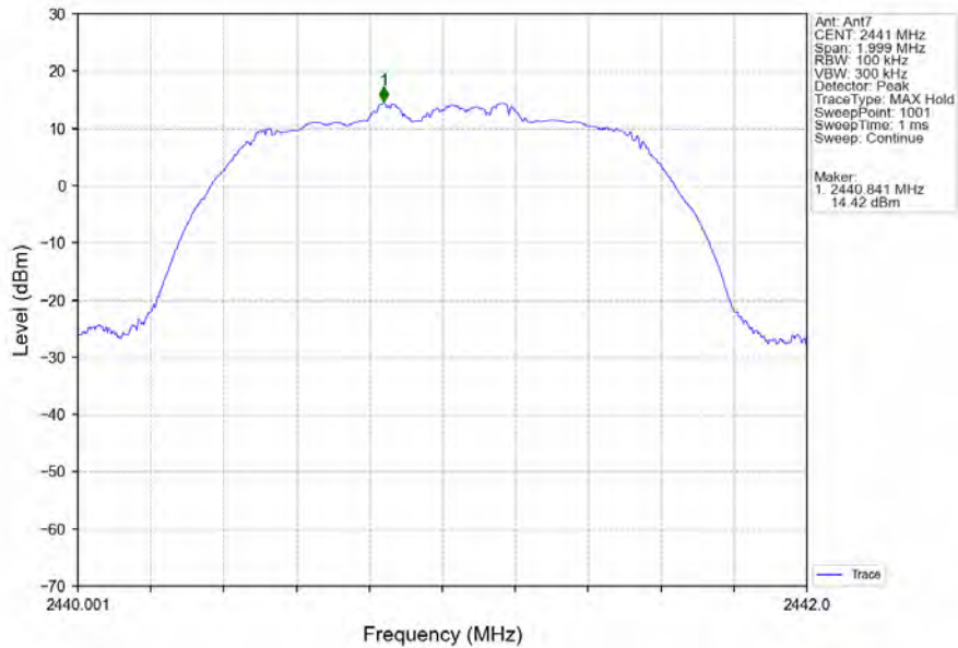
Pi/4DQPSK_2DH5_MCH_2441MHz_Ant7_NTNV
