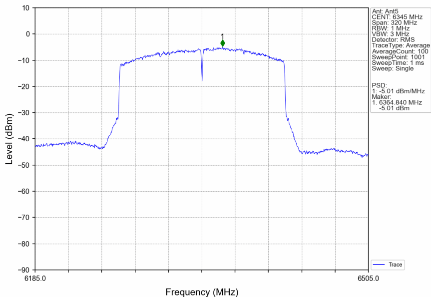
802.11be(EHT160)_HCH_6345MHz_SU_/_Ant5_NTNV
