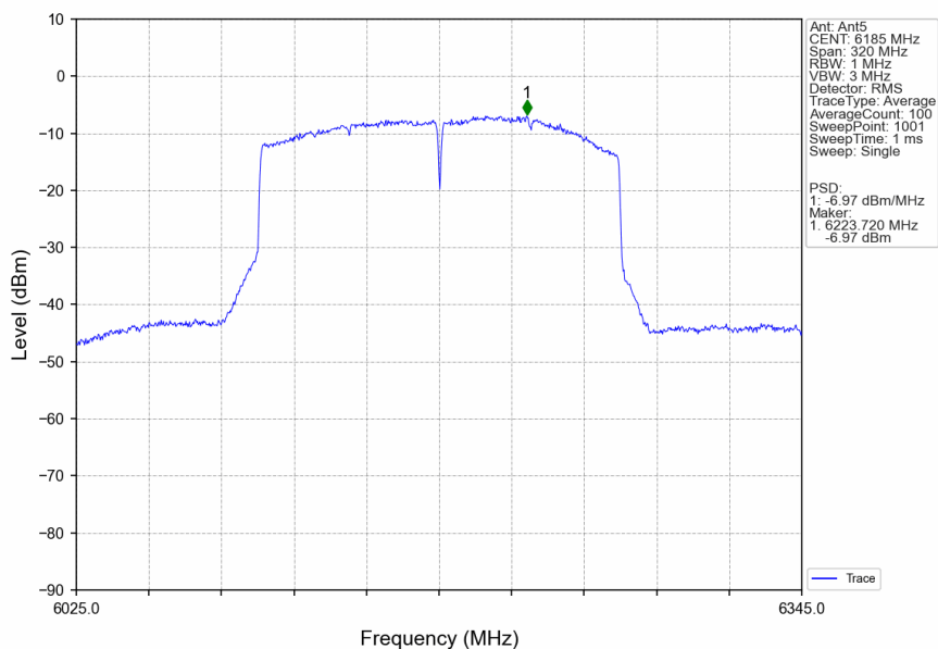
802.11be(EHT160)_MCH_6185MHz_SU_/_Ant5_NTNV
