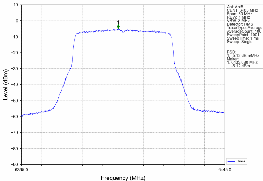
802.11be(EHT40)_HCH_6405MHz_SU_/_Ant5_NTNV
