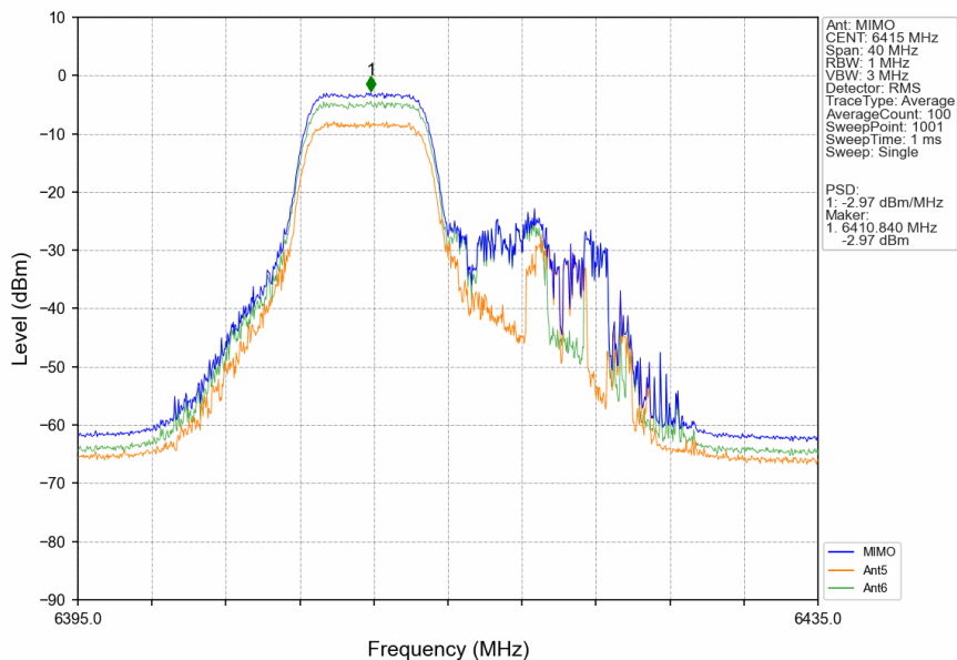
802.11be(EHT20)_HCH_6415MHz_26+52_/_MIMO_NTNV
