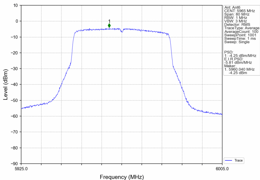
802.11ax(HEW40)_LCH_5965MHz_SU_/_Ant6_NTNV
