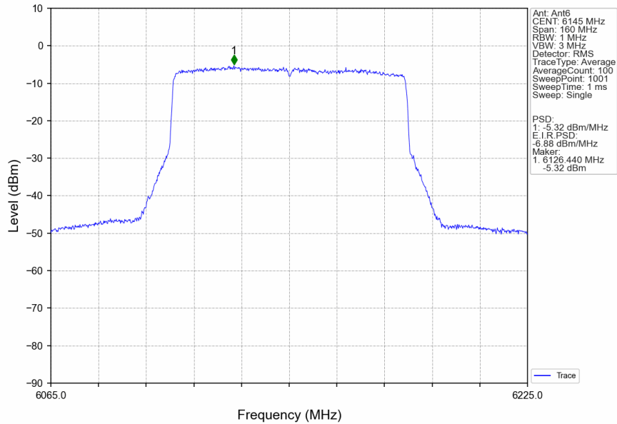
802.11ax(HEW80)_MCH_6145MHz_SU_/_Ant6_NTNV
