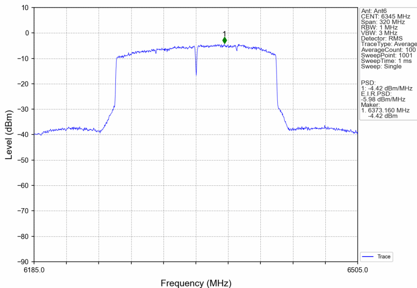
802.11ax(HEW160)_HCH_6345MHz_SU_/_Ant6_NTNV
