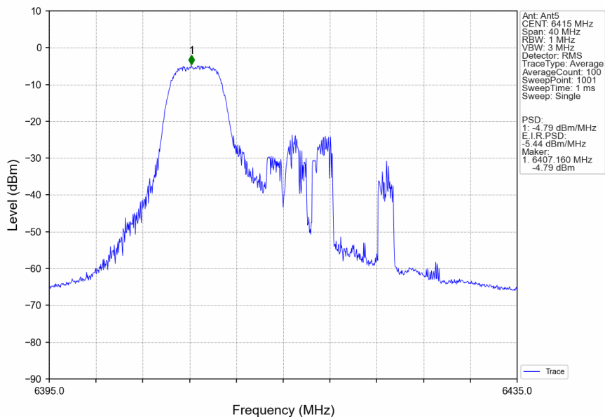
802.11ax(HEW20)_HCH_6415MHz_RU52_Left_Ant5_NTNV
