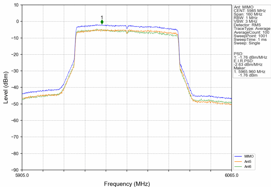
802.11ax(HEW80)_LCH_5985MHz_SU_/_MIMO_NTNV
