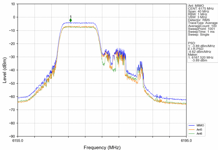
802.11ax(HEW20)_MCH_6175MHz_RU106_Left_MIMO_NTNV
