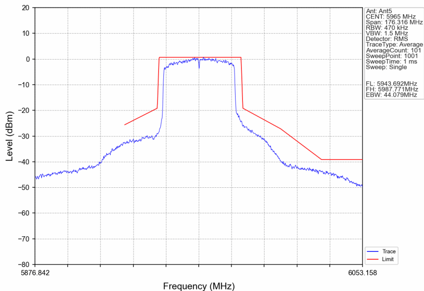
802.11ax(HEW40)_LCH_5965MHz_SU_/_Ant5_NTNV
