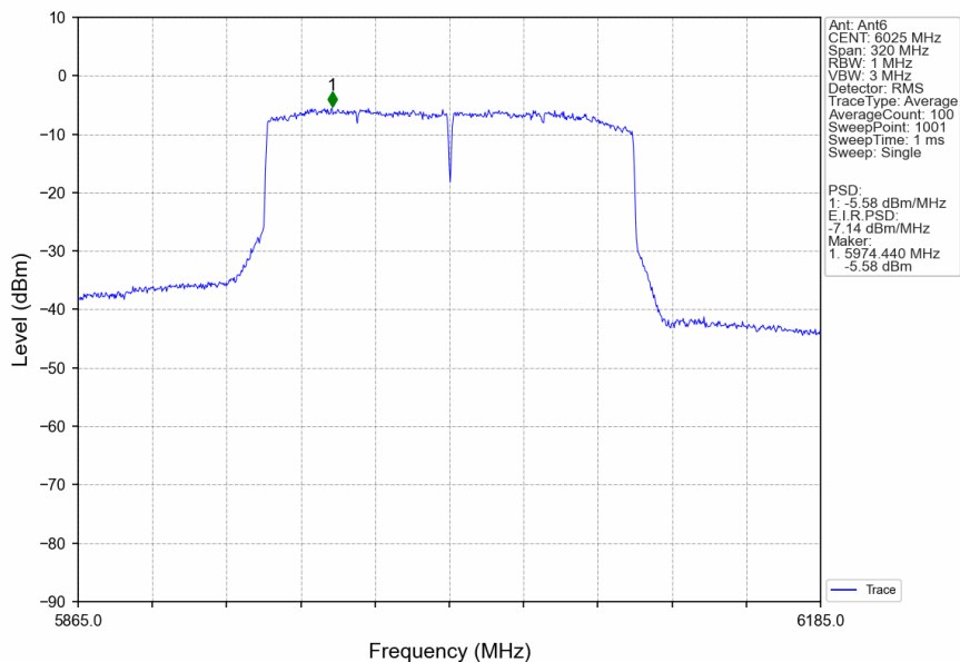
802.11ax(HEW160)_LCH_6025MHz_SU_/_Ant6_NTNV
