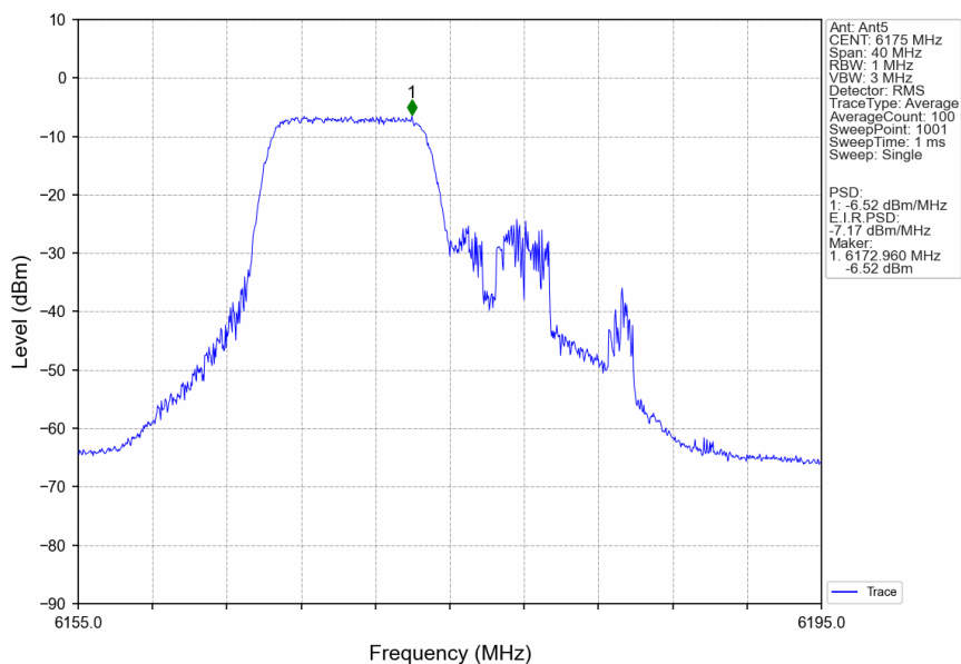
802.11ax(HEW20)_MCH_6175MHz_RU106_Left_Ant5_NTNV
