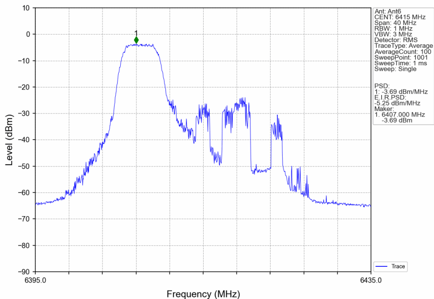
802.11ax(HEW20)_HCH_6415MHz_RU52_Left_Ant6_NTNV
