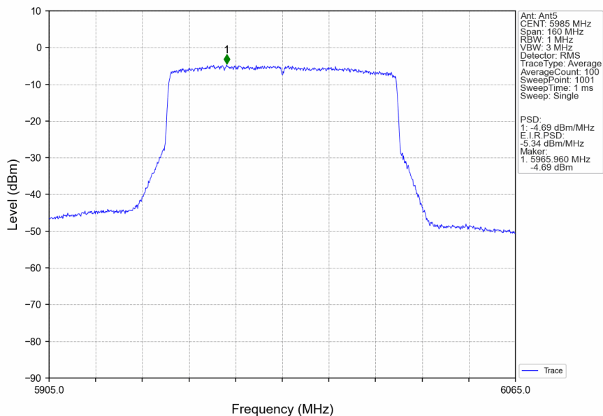
802.11ax(HEW80)_LCH_5985MHz_SU_/_Ant5_NTNV
