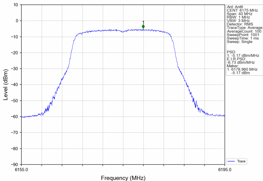
802.11ax(HEW20)_MCH_6175MHz_SU_/_Ant6_NTNV
