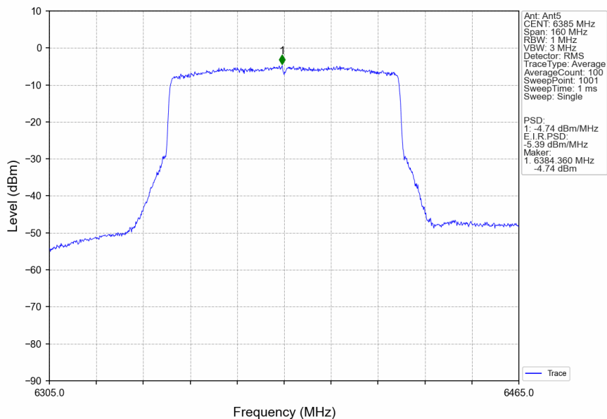
802.11ax(HEW80)_HCH_6385MHz_SU_/_Ant5_NTNV
