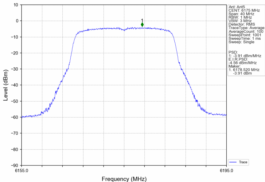
802.11ax(HEW20)_MCH_6175MHz_SU_/_Ant5_NTNV
