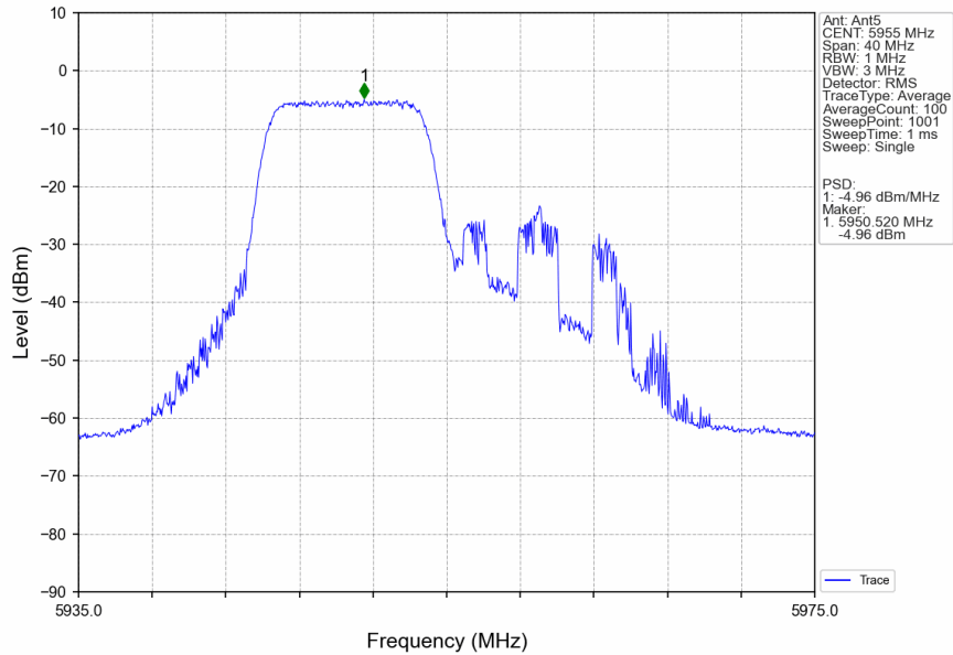
802.11ax(HEW20)_LCH_5955MHz_RU106_Left_Ant5_NTNV
