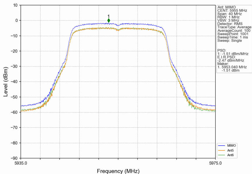
802.11ax(HEW20)_LCH_5955MHz_SU_/_MIMO_NTNV
