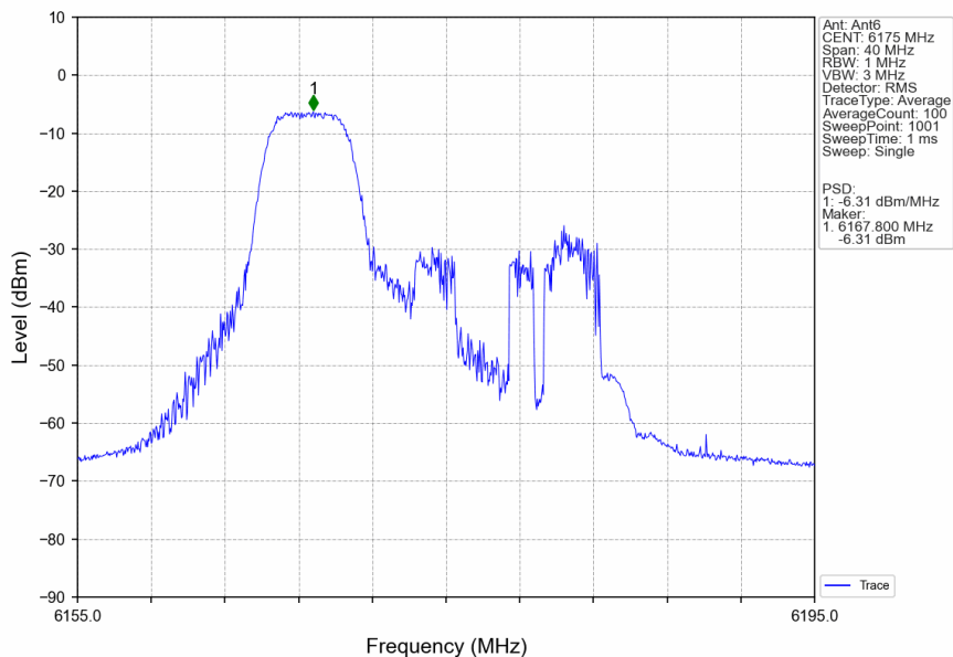
802.11ax(HEW20)_MCH_6175MHz_RU52_Left_Ant6_NTNV
