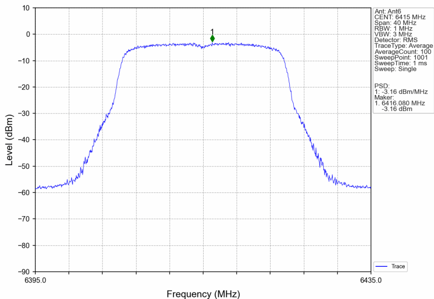
802.11ax(HEW20)_HCH_6415MHz_SU_/_Ant6_NTNV
