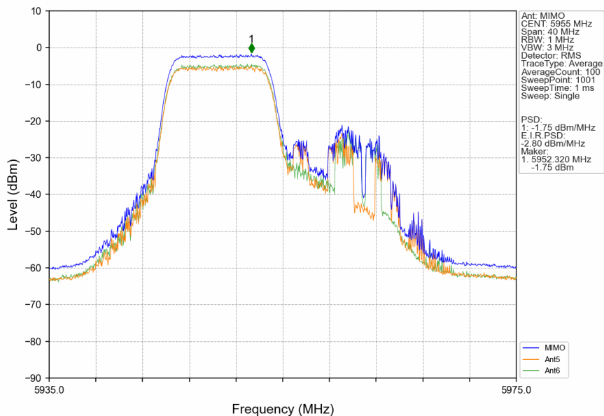
802.11ax(HEW20)_LCH_5955MHz_RU106_Left_MIMO_NTNV
