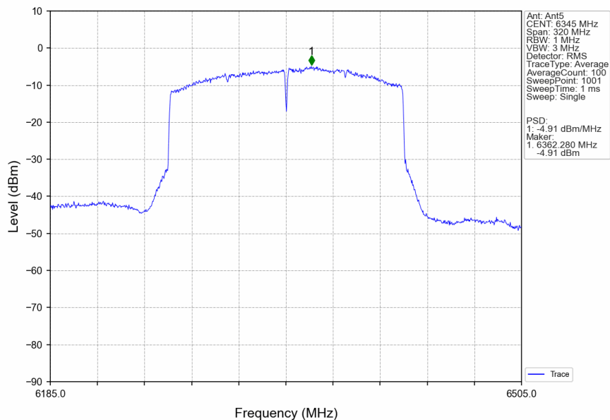
802.11ax(HEW160)_HCH_6345MHz_SU_/_Ant5_NTNV
