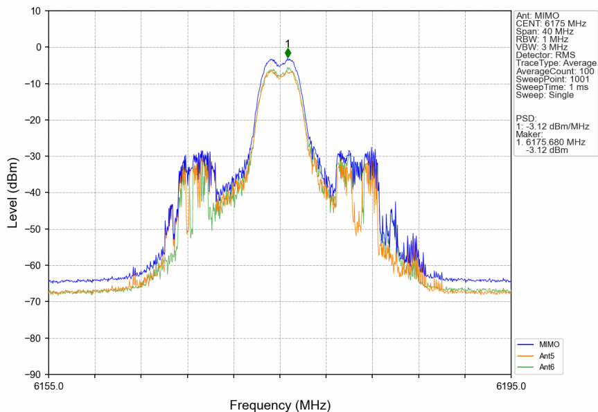
802.11ax(HEW20)_MCH_6175MHz_RU26_Mid_MIMO_NTNV
