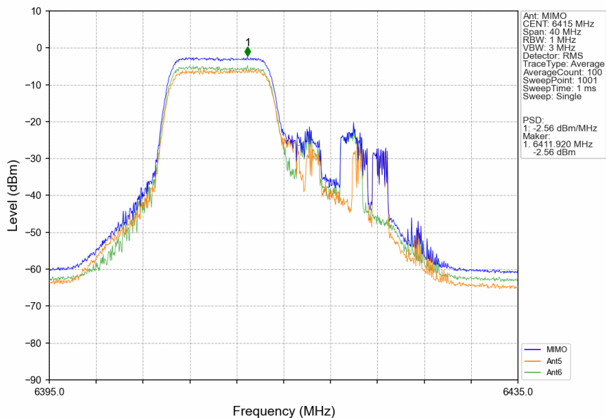
802.11ax(HEW20)_HCH_6415MHz_RU106_Left_MIMO_NTNV
