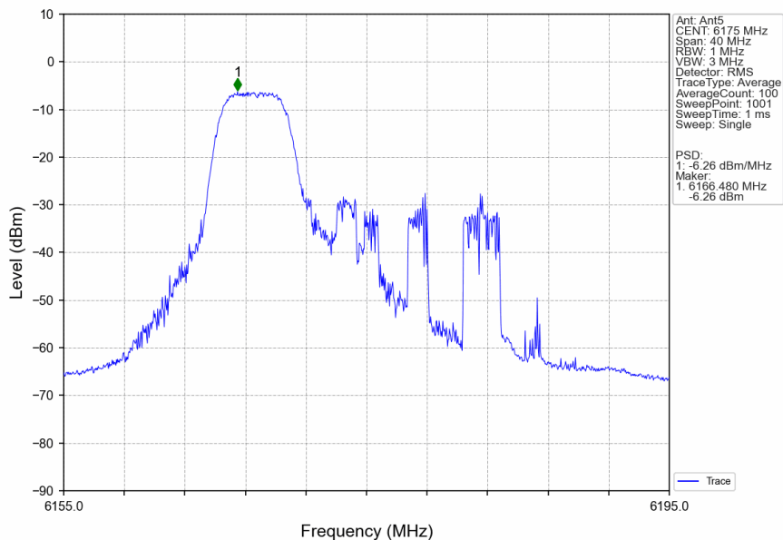
802.11ax(HEW20)_MCH_6175MHz_RU52_Left_Ant5_NTNV
