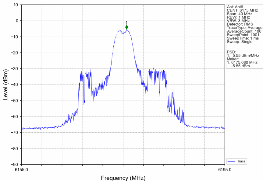
802.11ax(HEW20)_MCH_6175MHz_RU26_Mid_Ant6_NTNV
