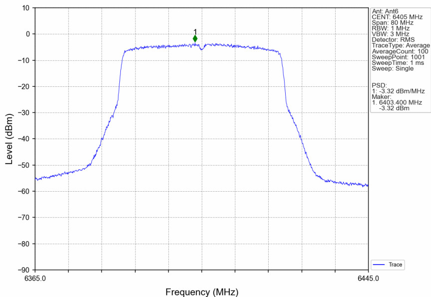
802.11ax(HEW40)_HCH_6405MHz_SU_/_Ant6_NTNV
