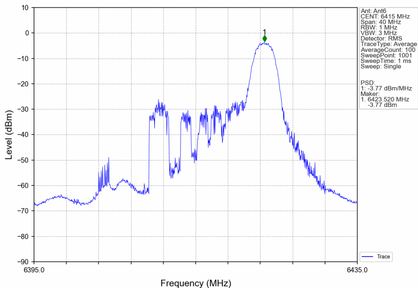
802.11ax(HEW20)_HCH_6415MHz_RU26_Right_Ant6_NTNV
