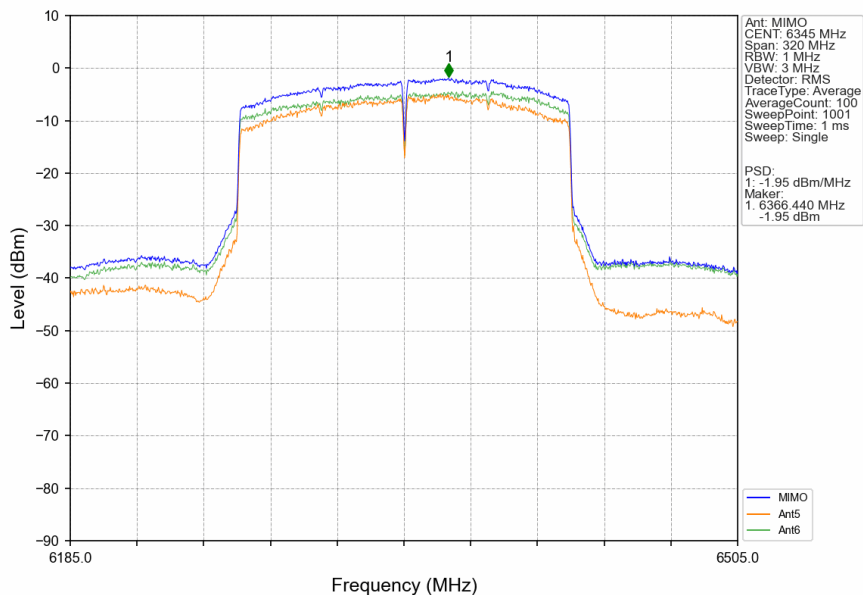
802.11ax(HEW160)_HCH_6345MHz_SU_/_MIMO_NTNV
