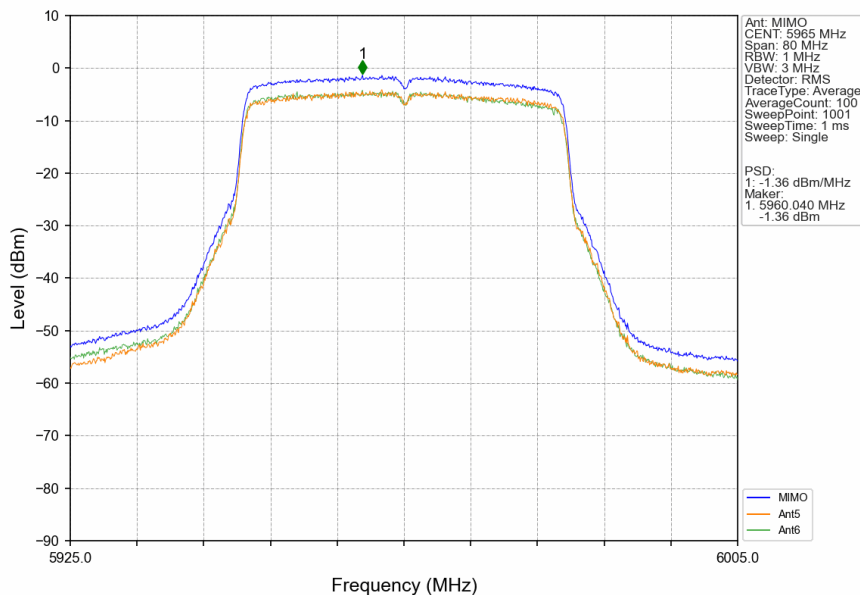
802.11ax(HEW40)_LCH_5965MHz_SU_/_MIMO_NTNV
