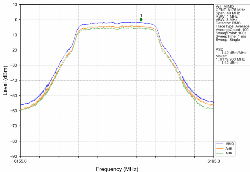
802.11a_MCH_6175MHz_MIMO_NTNV
