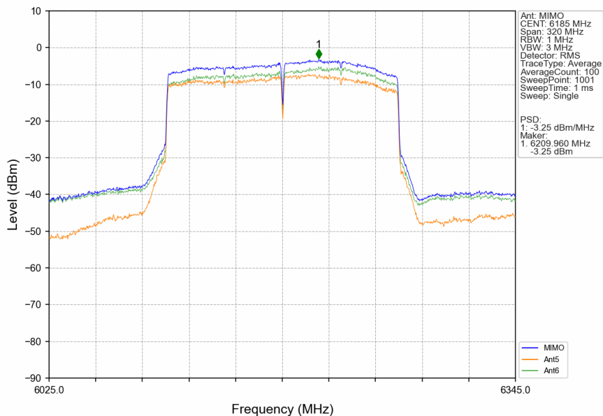
802.11ax(HEW160)_MCH_6185MHz_SU_/_MIMO_NTNV
