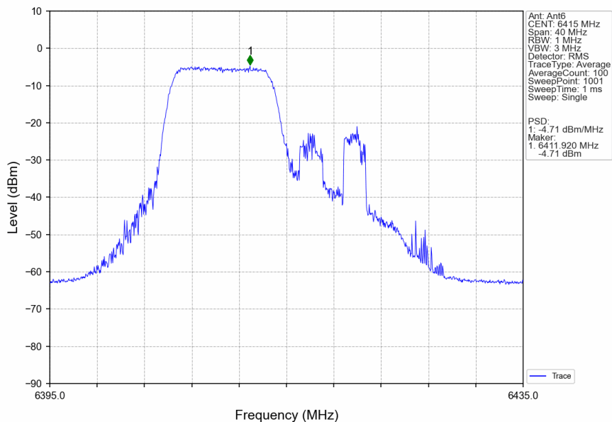
802.11ax(HEW20)_HCH_6415MHz_RU106_Left_Ant6_NTNV
