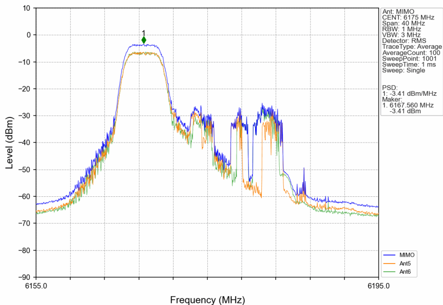
802.11ax(HEW20)_MCH_6175MHz_RU52_Left_MIMO_NTNV
