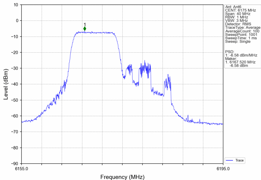
802.11ax(HEW20)_MCH_6175MHz_RU106_Left_Ant6_NTNV
