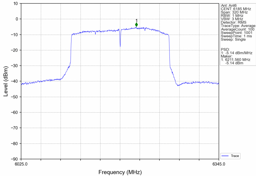
802.11ax(HEW160)_MCH_6185MHz_SU_/_Ant6_NTNV
