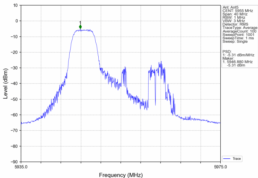
802.11ax(HEW20)_LCH_5955MHz_RU52_Left_Ant5_NTNV
