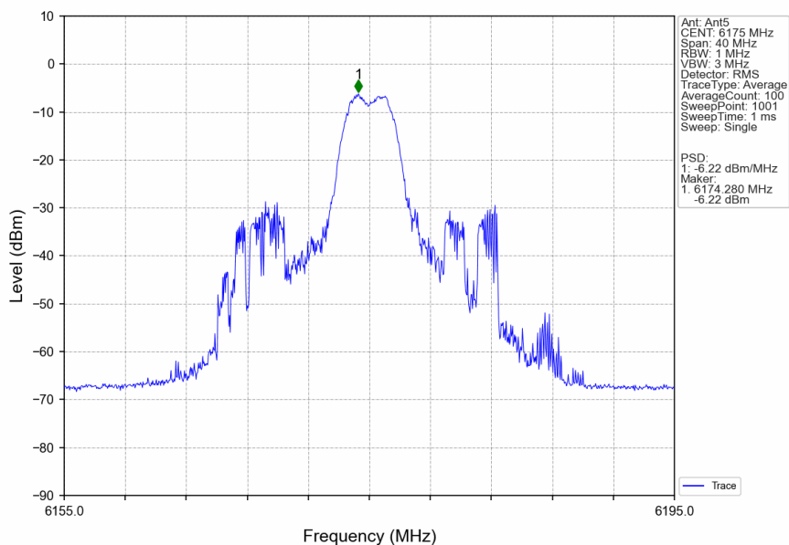
802.11ax(HEW20)_MCH_6175MHz_RU26_Mid_Ant5_NTNV
