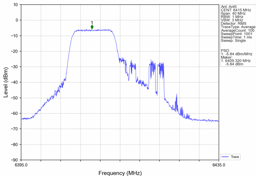
802.11ax(HEW20)_HCH_6415MHz_RU106_Left_Ant5_NTNV
