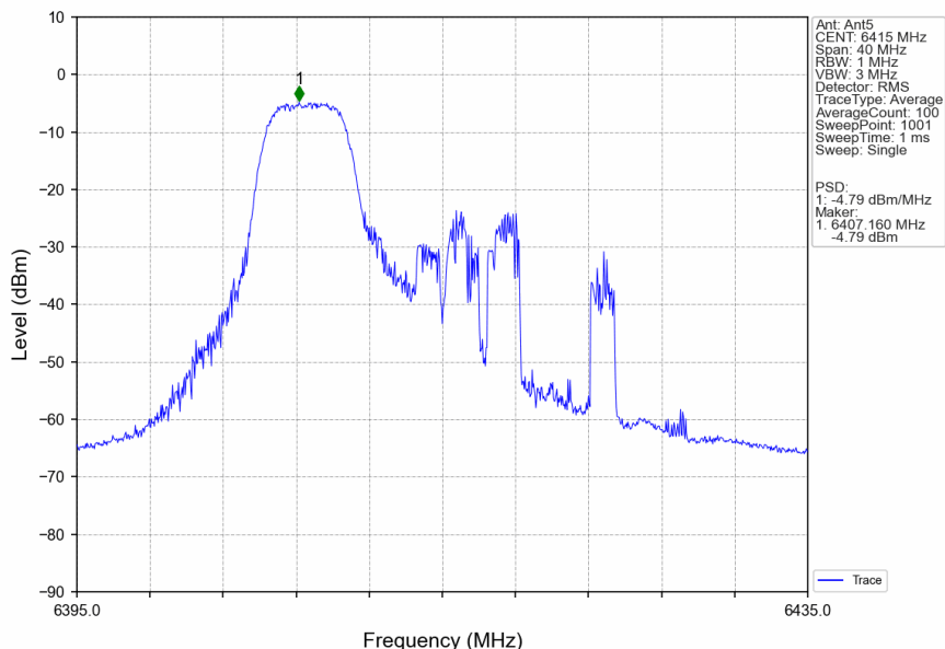
802.11ax(HEW20)_HCH_6415MHz_RU52_Left_Ant5_NTNV
