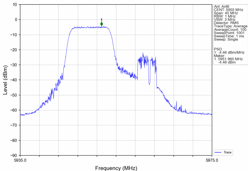
802.11ax(HEW20)_LCH_5955MHz_RU106_Left_Ant6_NTNV
