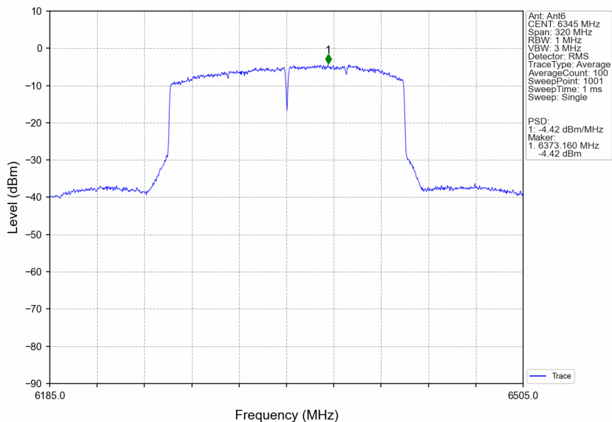
802.11ax(HEW160)_HCH_6345MHz_SU_/_Ant6_NTNV
