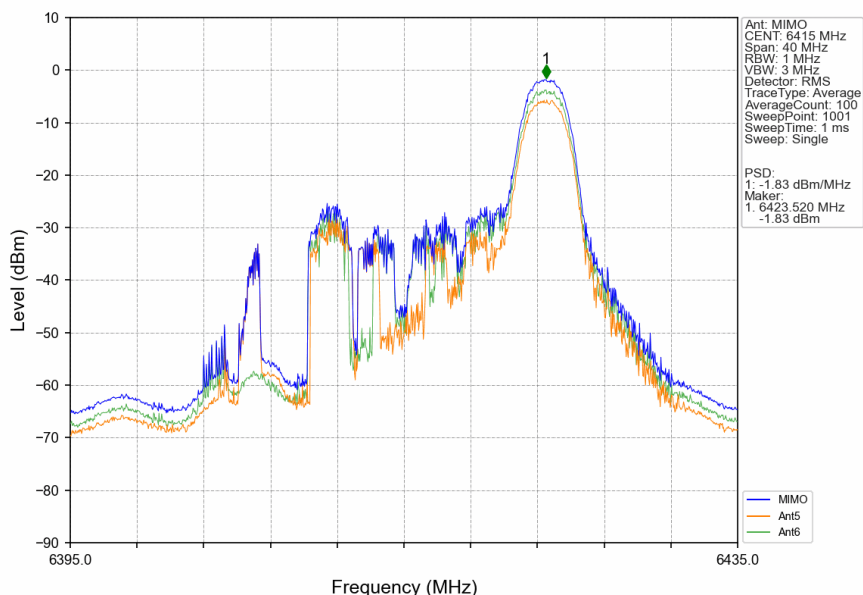
802.11ax(HEW20)_HCH_6415MHz_RU26_Right_MIMO_NTNV
