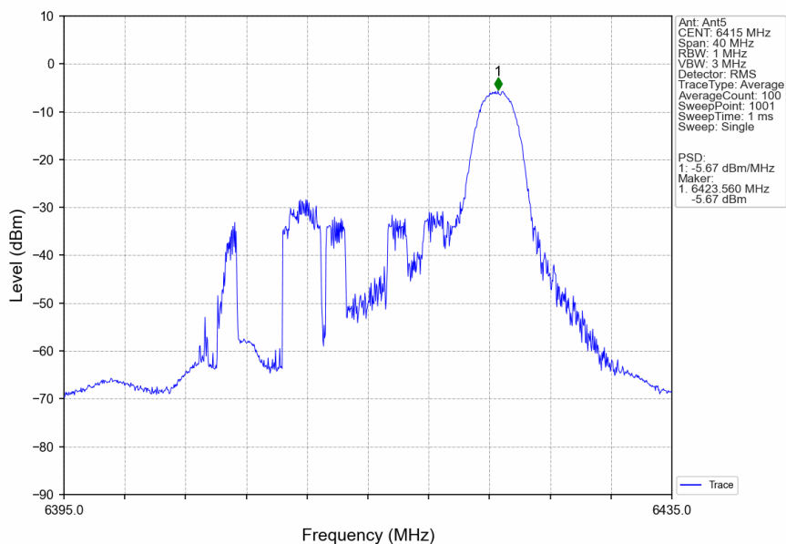
802.11ax(HEW20)_HCH_6415MHz_RU26_Right_Ant5_NTNV
