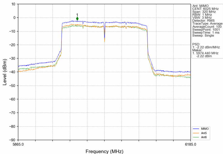
802.11ax(HEW160)_LCH_6025MHz_SU_/_MIMO_NTNV
