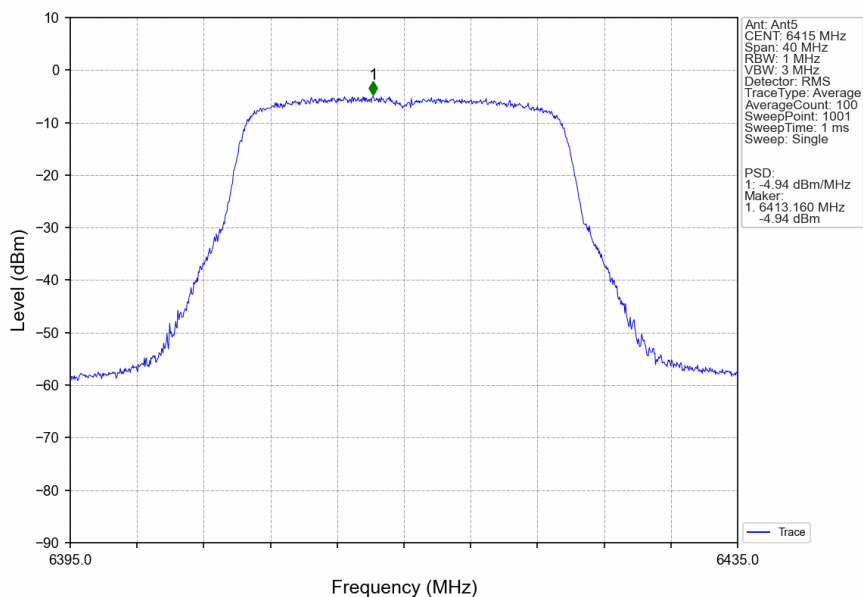
802.11ax(HEW20)_HCH_6415MHz_SU_/_Ant5_NTNV
