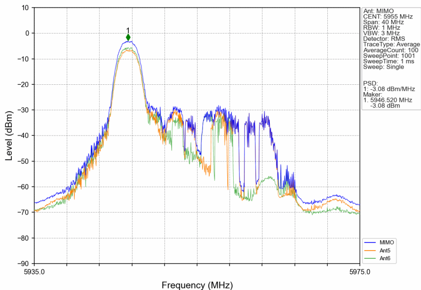
802.11ax(HEW20)_LCH_5955MHz_RU26_Left_MIMO_NTNV
