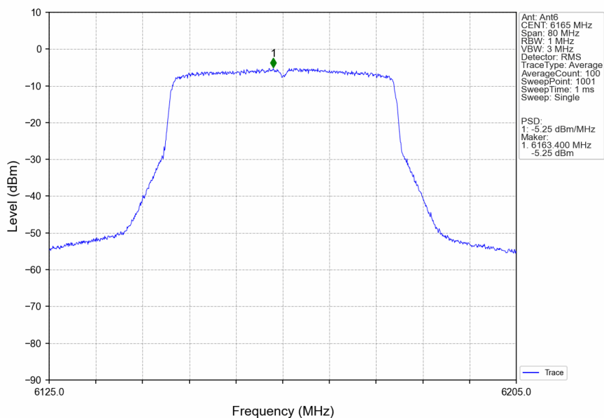
802.11ax(HEW40)_MCH_6165MHz_SU_/_Ant6_NTNV
