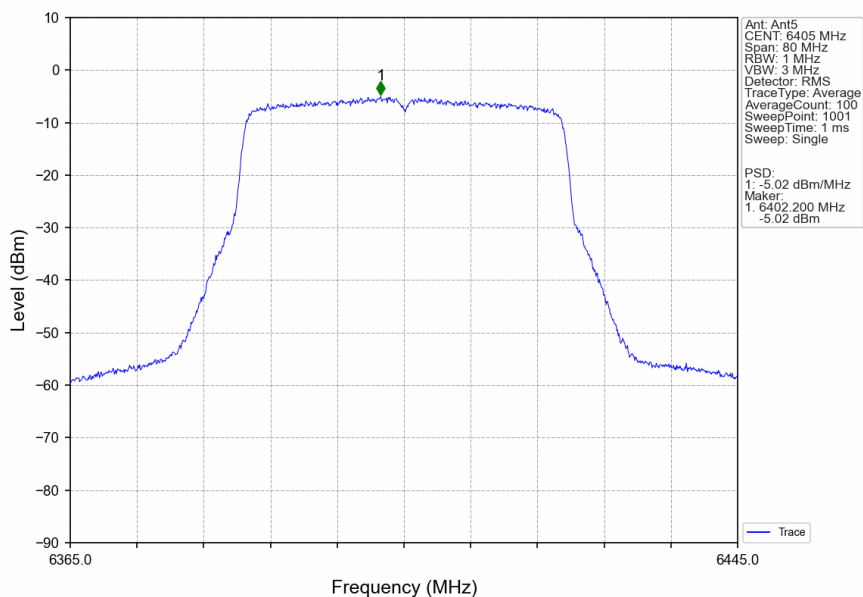
802.11ax(HEW40)_HCH_6405MHz_SU_/_Ant5_NTNV
