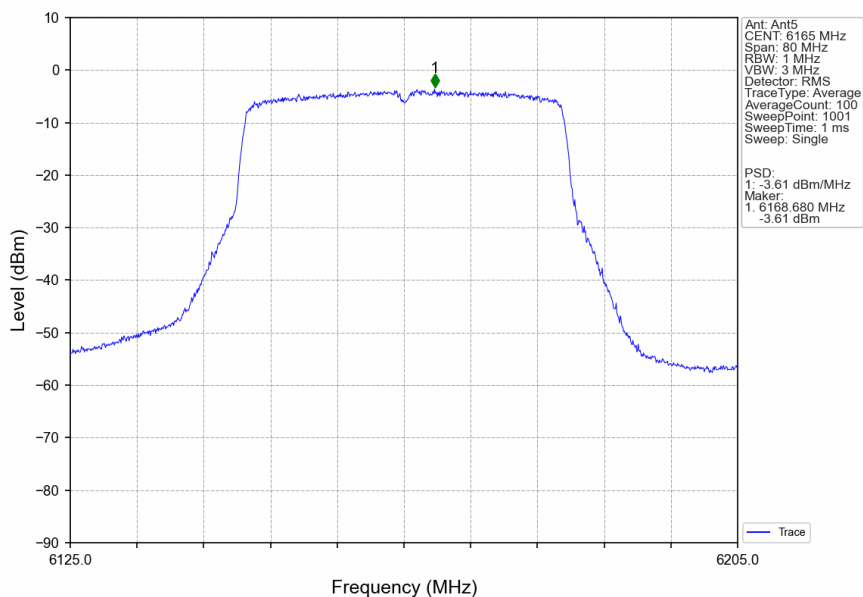
802.11ax(HEW40)_MCH_6165MHz_SU_/_Ant5_NTNV
