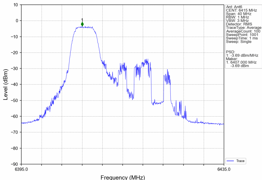
802.11ax(HEW20)_HCH_6415MHz_RU52_Left_Ant6_NTNV
