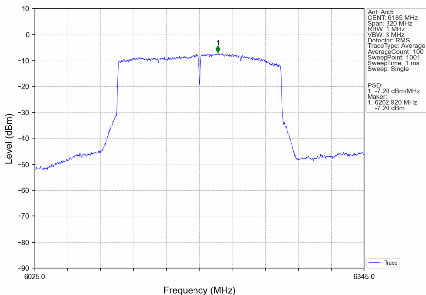
802.11ax(HEW160)_MCH_6185MHz_SU_/_Ant5_NTNV
