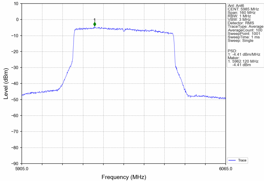
802.11ax(HEW80)_LCH_5985MHz_SU_/_Ant6_NTNV
