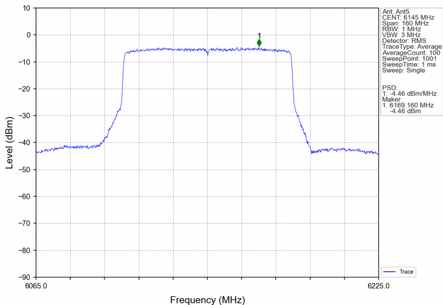
802.11ax(HEW80)_MCH_6145MHz_SU_/_Ant5_NTNV
