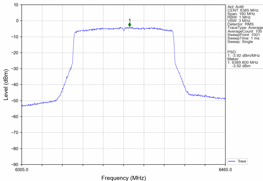
802.11ax(HEW80)_HCH_6385MHz_SU_/_Ant6_NTNV
