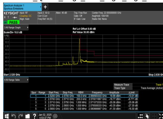
N7(10M)_DFT-s- OFDM_QPSK_Edge_1RB_Right_High_CH
