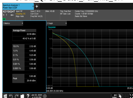
N7(20M)_DFT-s-OFDM_QPSK_Outer_Full_Mid_CH
