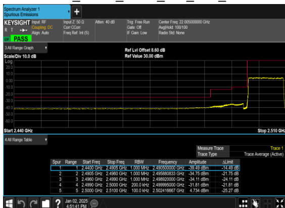
N7(10M)_DFT-s- OFDM_BPSK_Outer_Full_Low_CH
