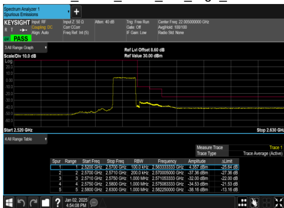
N7(10M)_DFT-s- OFDM_BPSK_Outer_Full_High_CH
