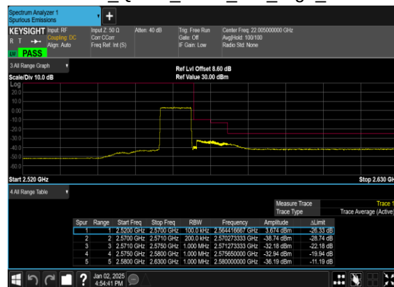
N7(10M)_DFT-s- OFDM_QPSK_Outer_Full_High_CH
