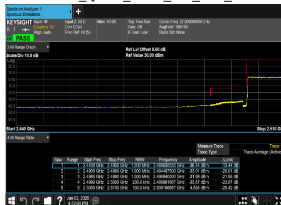
N7(10M)_DFT-s- OFDM_QPSK_Outer_Full_Low_CH
