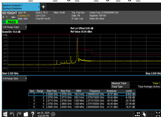
N7(10M)_DFT-s- OFDM_BPSK_Edge_1RB_Right_High_CH
