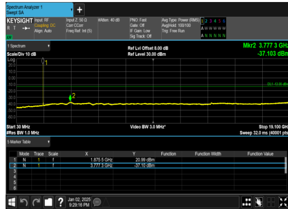
N2(10M)_DFT-s- OFDM_QPSK_Edge_1RB_Left_Mid_CH
