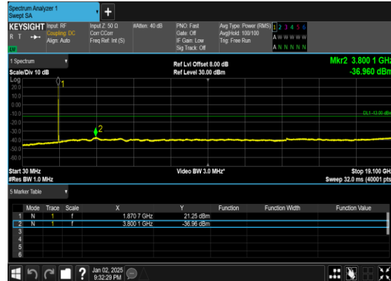
N2(20M)_DFT-s- OFDM_QPSK_Edge_1RB_Left_Mid_CH
