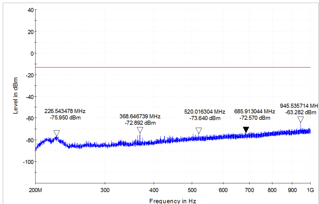
Horizontal Polarization
