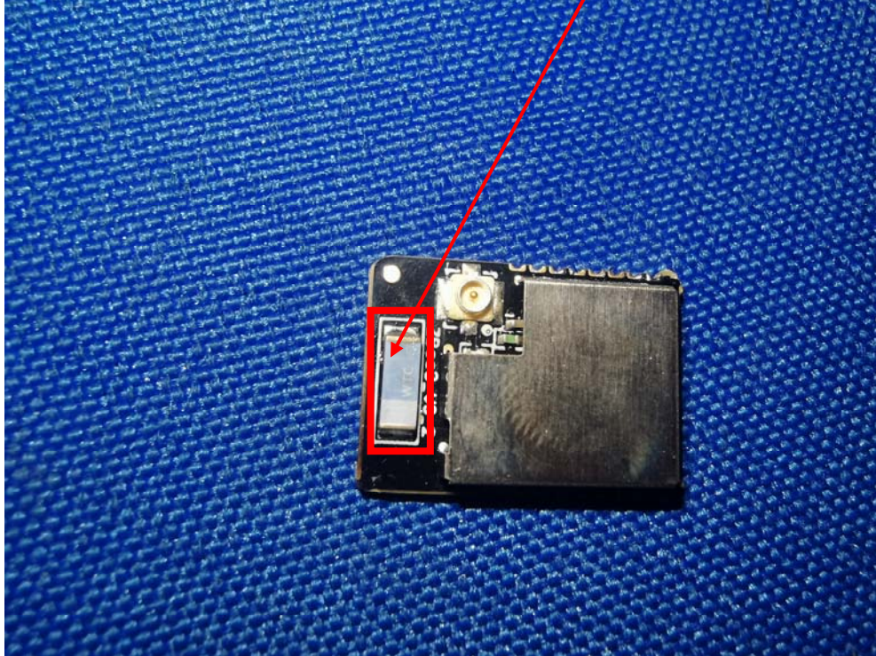
Chip Antenna
