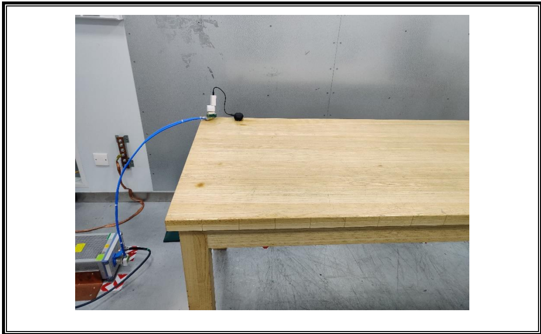
POWERLINE CONDUCTED EMISSIONS MEASUREMENT SETUP
