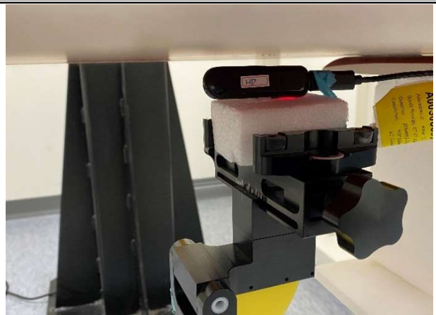
Photo 4: Vertical Back_0.5cm
