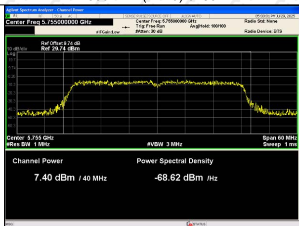
5802.11n(HT40)-5755
