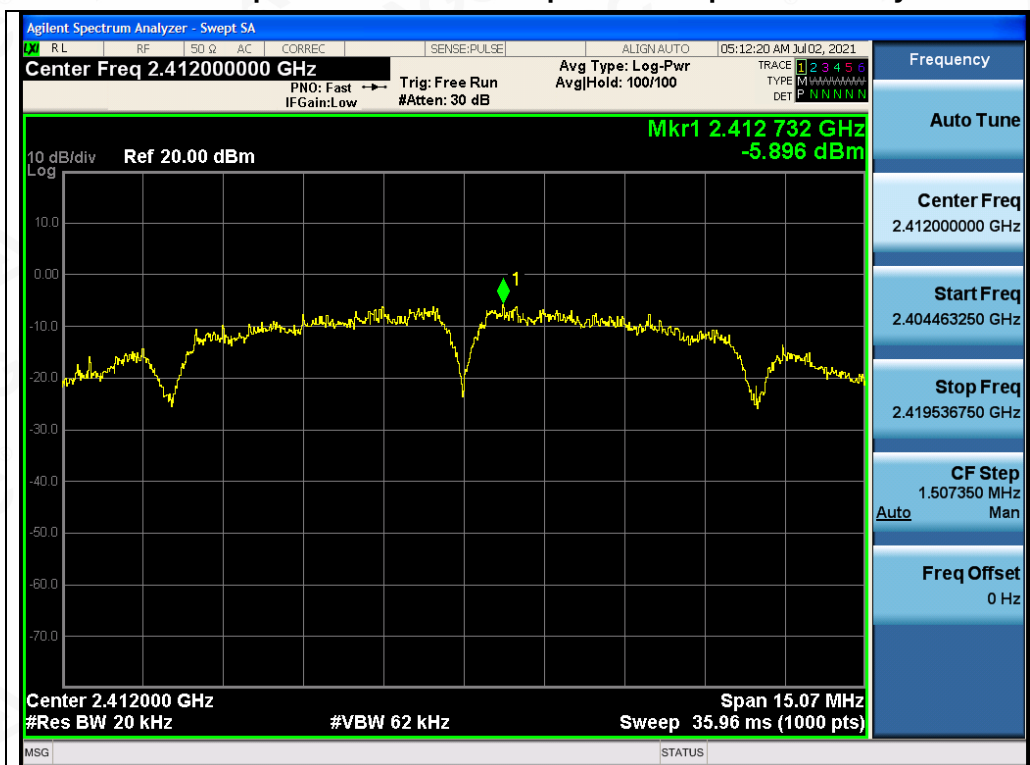
Test Graph 802.11b ANT1 2412 1Mbps PSD
