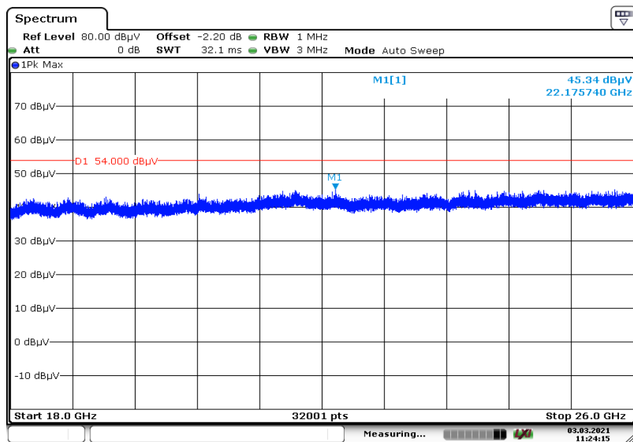
Plot 4: 18 GHz to 26 GHz, TX mode, 2440 MHz, vertical & horizontal polarization, O-QPSK
