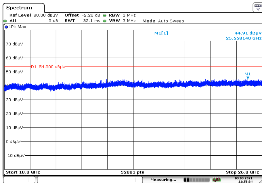
Plot 6: 18 GHz to 26 GHz, TX mode, 2475 MHz, vertical & horizontal polarization, O-QPSK
