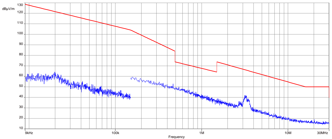
Plot 2: 9 kHz to 30 MHz, 2426MHz, transmit mode, 1 Msps
