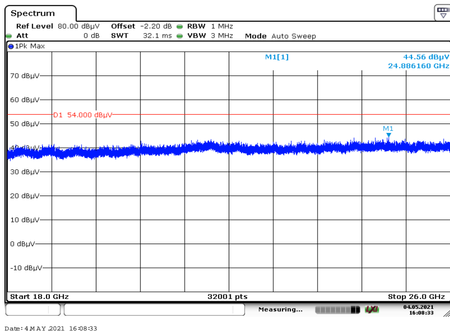
Plot 4: 18 GHz to 26 GHz, TX mode, 2426MHz, vertical & horizontal polarization, 1 Msp/s
