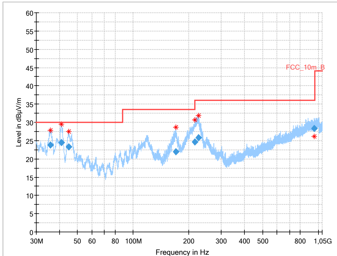
Plot 2: 30 MHz to 1 GHz, TX mode, 2426MHz, vertical & horizontal polarization, 1 Msps
