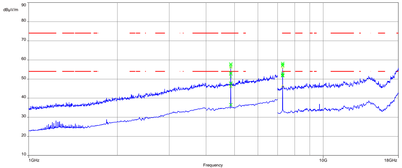
Plot 3: 1 GHz to 18 GHz, TX mode, 2426MHz, vertical & horizontal polarization, 1 Msp/s
