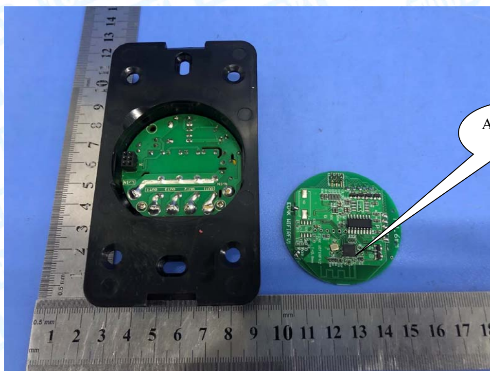
Photo 9 Internal of PCB
