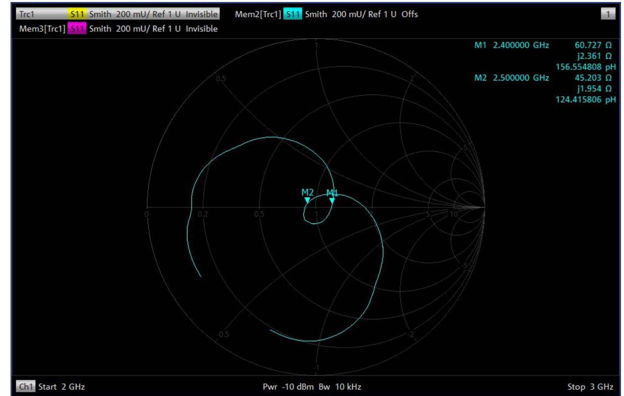
Smith Chart
