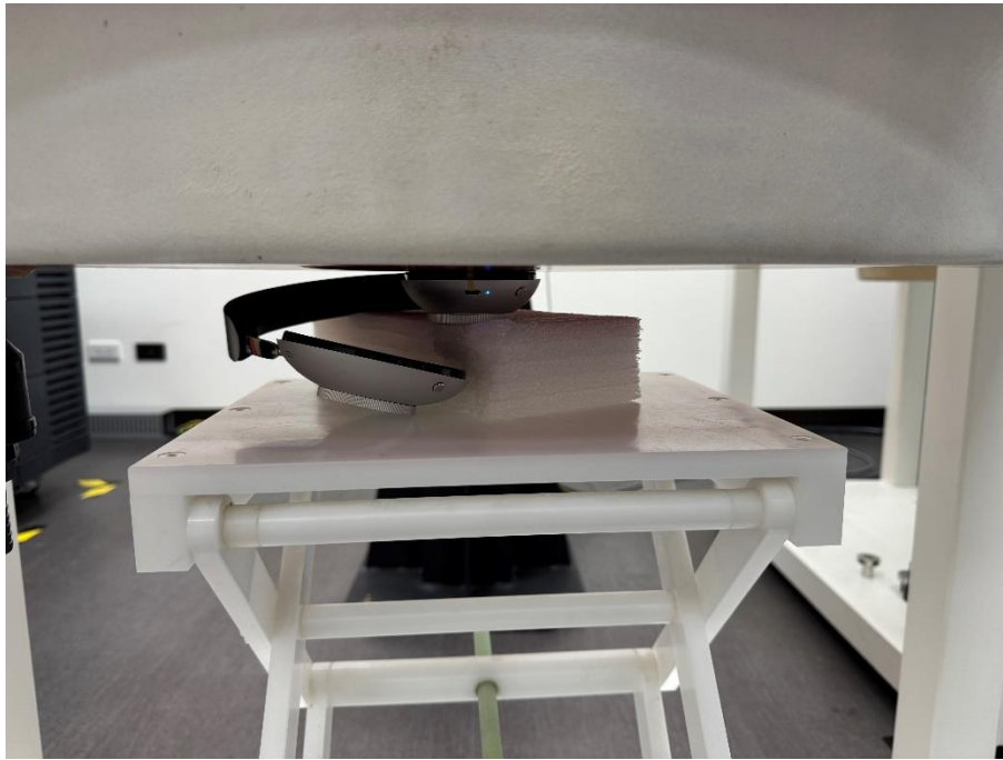
Inner ear
