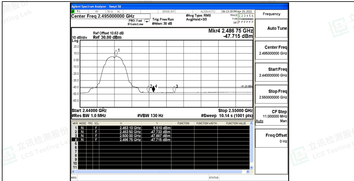
11B_Ant_High_2462_Peak
