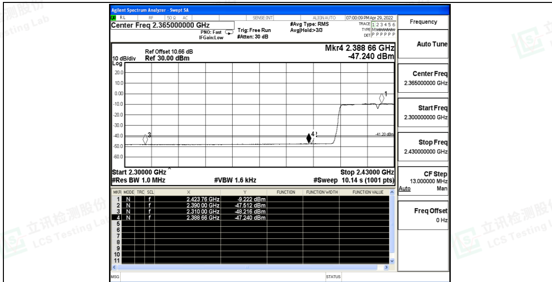
11N40SISO_Ant_Low_2422_Peak
