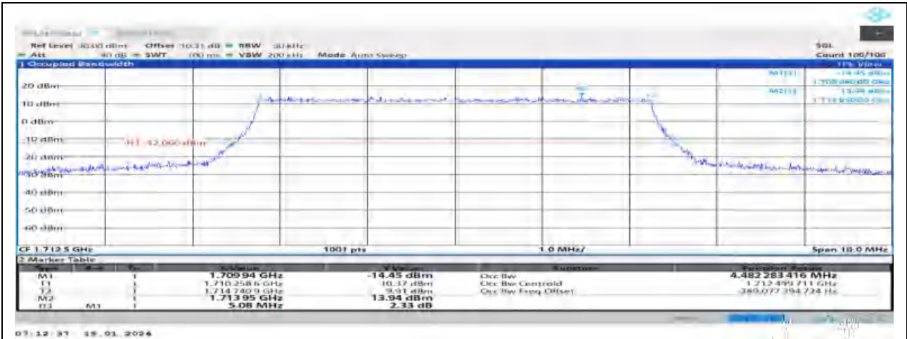
Band4-5MHz-QPSK-20175-25RB#0
