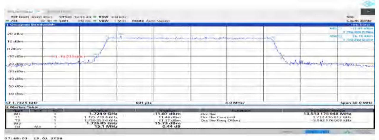
Band4-15MHz-16QAM-20325-75RB#0
