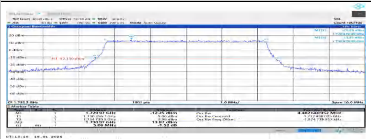
Band4-5MHz-QPSK-20375-25RB#0
