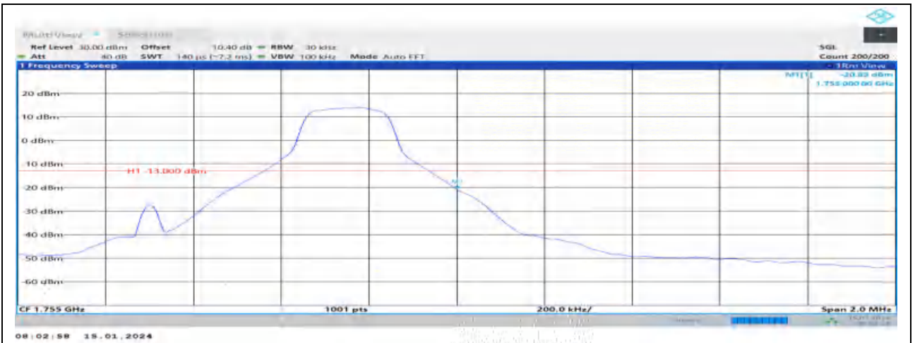
Band4-1.4MHz-16QAM-20393-6RB#0
