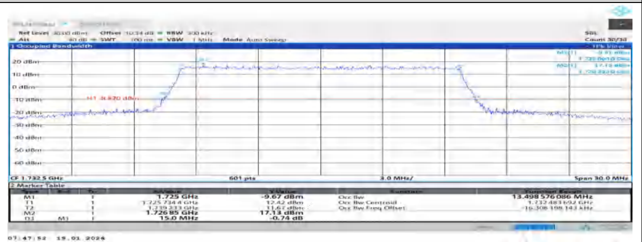
Band4-15MHz-QPSK-20325-75RB#0
