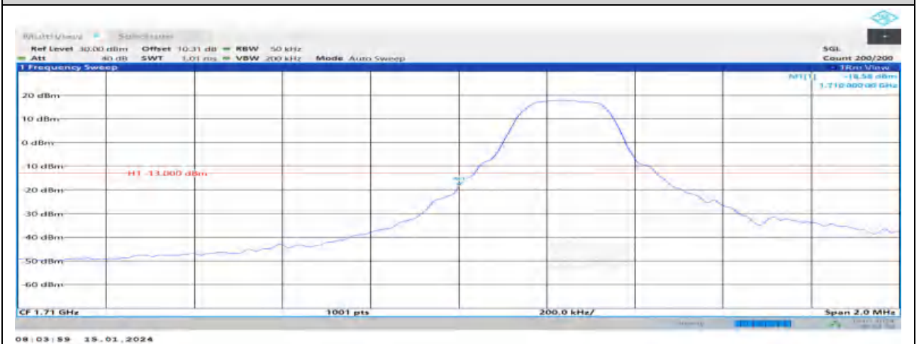
Band4-3MHz-QPSK-19965-15RB#0
