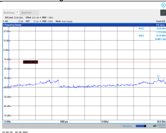
Band66-10MHz-16QAM-132022-1RB#0- Range2:1000~20000MHz
