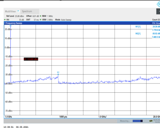
Band66-1.4MHz-16QAM-132665-1RB#0- Range2:1000~20000MHz
