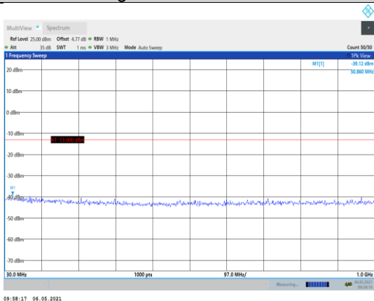
Band2-20MHz-16QAM-18900-1RB#0- Range1:30~1000MHz
