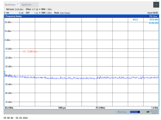
Band2-20MHz-QPSK-19100-1RB#0- Range1:30~1000MHz
