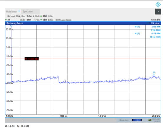
Band4-5MHz-16QAM-20175-1RB#0- Range2:1000~20000MHz
