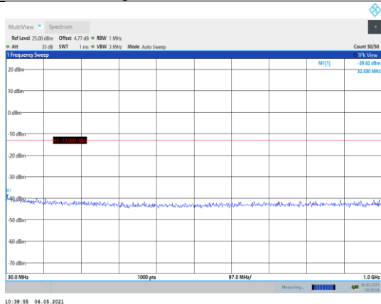
Band66-1.4MHz-16QAM-132322-1RB#0- Range1:30~1000MHz
