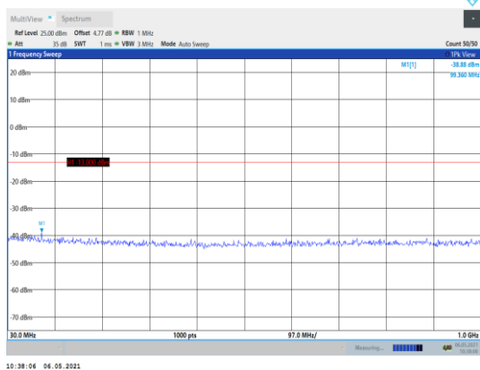
Band66-1.4MHz-16QAM-131979-1RB#0- Range1:30~1000MHz
