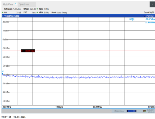
Band2-20MHz-QPSK-18900-1RB#0- Range1:30~1000MHz
