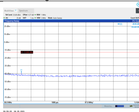
Band2-20MHz-16QAM-19100-1RB#0- Range1:30~1000MHz
