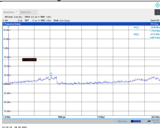
Band4-10MHz-16QAM-20000-1RB#0- Range2:1000~20000MHz
