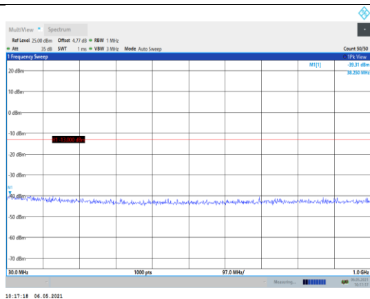
Band4-5MHz-QPSK-19975-1RB#0- Range1:30~1000MHz
