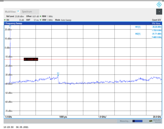
Band4-15MHz-16QAM-20175-1RB#0- Range2:1000~20000MHz
