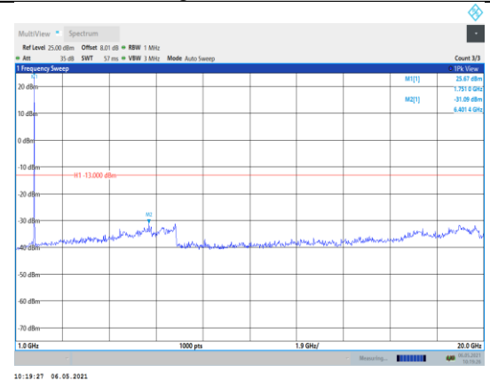
Band4-5MHz-16QAM-20375-1RB#0- Range2:1000~20000MHz
