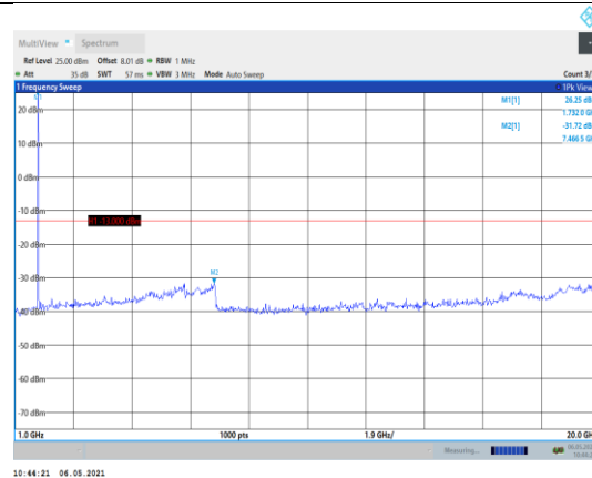
Band66-10MHz-16QAM-132322-1RB#0- Range2:1000~20000MHz
