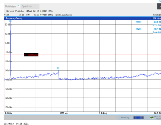
Band66-1.4MHz-16QAM-132322-1RB#0- Range2:1000~20000MHz
