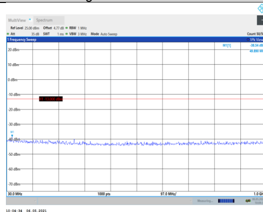
Band2-5MHz-16QAM-19175-1RB#0- Range1:30~1000MHz
