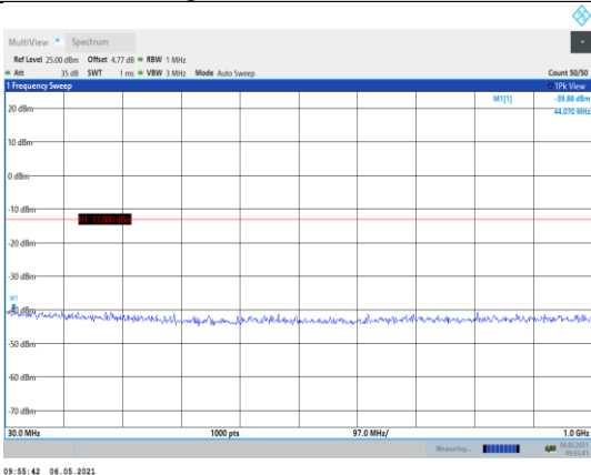
Band2-1.4MHz-16QAM-18900-1RB#0- Range1:30~1000MHz
