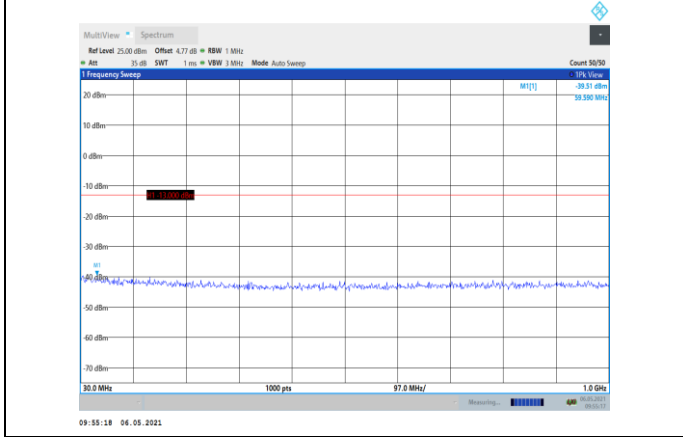
Band2-1.4MHz-QPSK-18900-1RB#0- Range1:30~1000MHz
