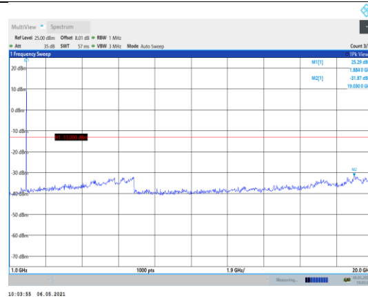
Band2-5MHz-16QAM-18900-1RB#0- Range2:1000~20000MHz
