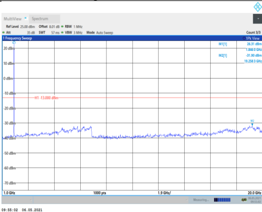
Band2-1.4MHz-16QAM-18607-1RB#0- Range2:1000~20000MHz
