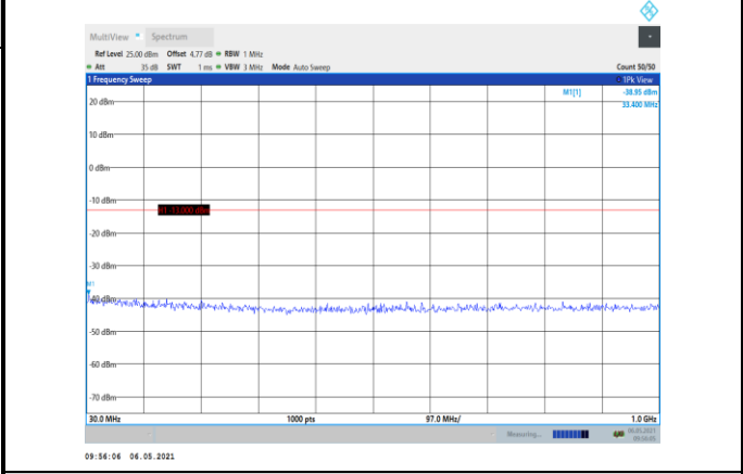
Band2-1.4MHz-QPSK-19193-1RB#0- Range1:30~1000MHz
