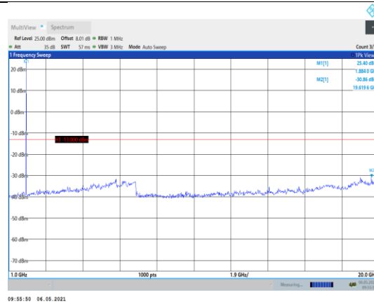
Band2-1.4MHz-16QAM-18900-1RB#0- Range2:1000~20000MHz
