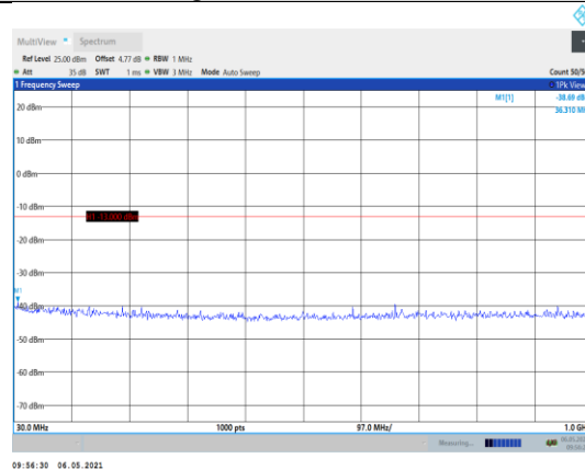
Band2-1.4MHz-16QAM-19193-1RB#0- Range1:30~1000MHz
