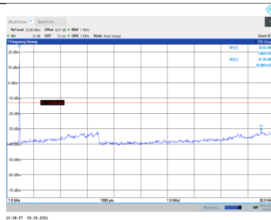
Band2-10MHz-QPSK-18900-1RB#0- Range2:1000~20000MHz
