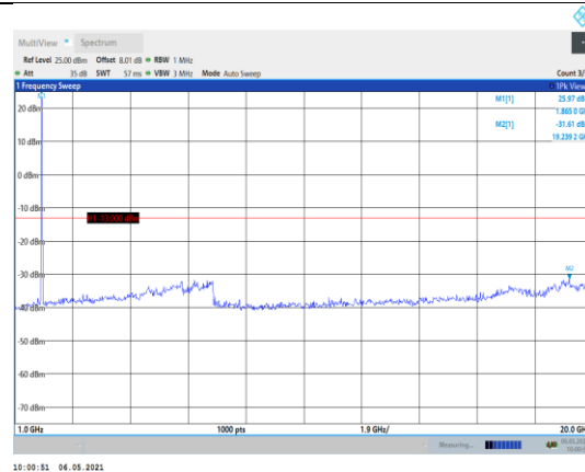
Band2-15MHz-QPSK-18900-1RB#0- Range2:1000~20000MHz
