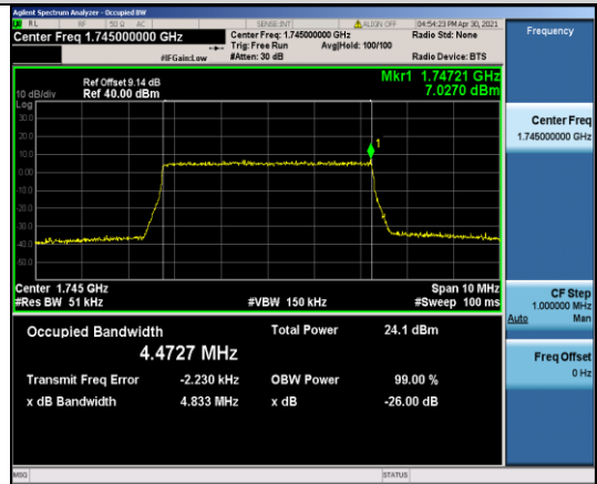
Band66-5MHz-16QAM-132322-25RB#0-4.4727
