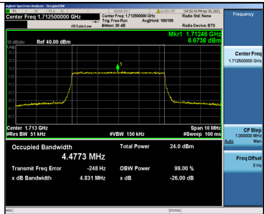
Band66-5MHz-16QAM-131997-25RB#0-4.4773
