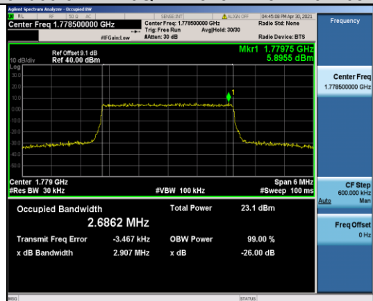
Band66-3MHz-16QAM-132657-15RB#0-2.6862
