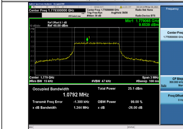
Band66-1.4MHz-QPSK-132665-6RB#0-1.0792
