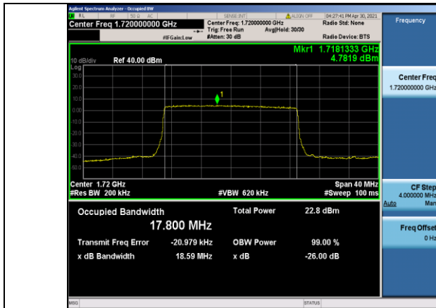
Band66-20MHz-QPSK-132072-100RB#0-17.800
