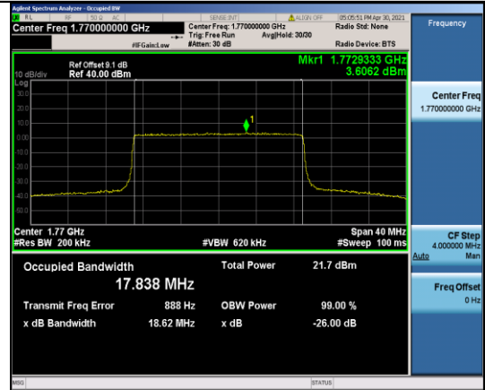
Band66-20MHz-16QAM-132572-100RB#0-17.838
