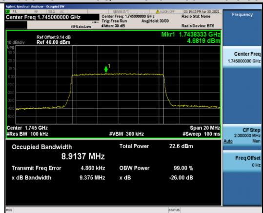
Band66-10MHz-16QAM-132322-50RB#0-8.9137
