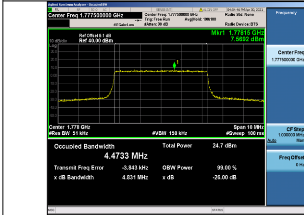
Band66-5MHz-QPSK-132647-25RB#0-4.4733
