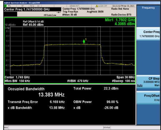
Band4-15MHz-16QAM-20325-75RB#0-13.383
