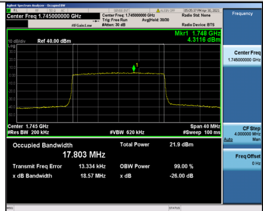
Band66-20MHz-16QAM-132322-100RB#0-17.803
