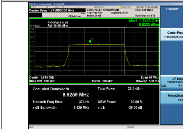
Band66-10MHz-QPSK-132322-50RB#0-8.9259
