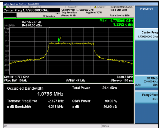
Band66-1.4MHz-16QAM-132665-6RB#0-1.0796
