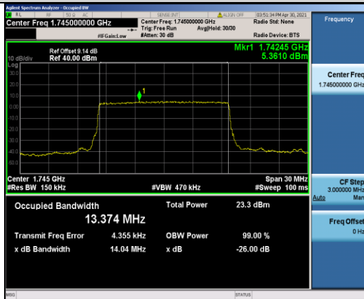
Band66-15MHz-QPSK-132322-75RB#0-13.374
