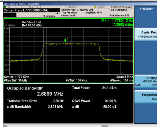
Band66-3MHz-QPSK-132657-15RB#0-2.6869
