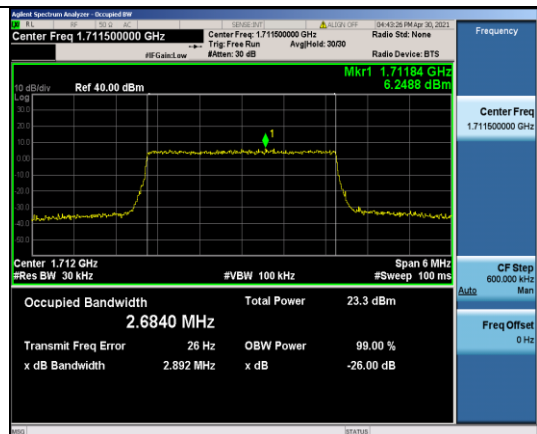
Band66-3MHz-16QAM-131987-15RB#0-2.6840
