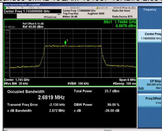
Band66-3MHz-16QAM-132322-15RB#0-2.6819
