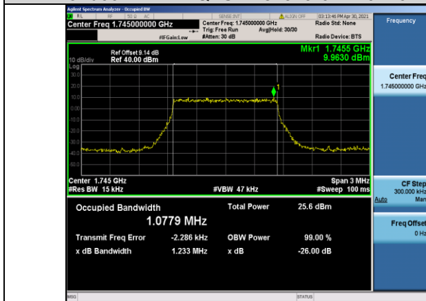
Band66-1.4MHz-QPSK-132322-6RB#0-1.0779
