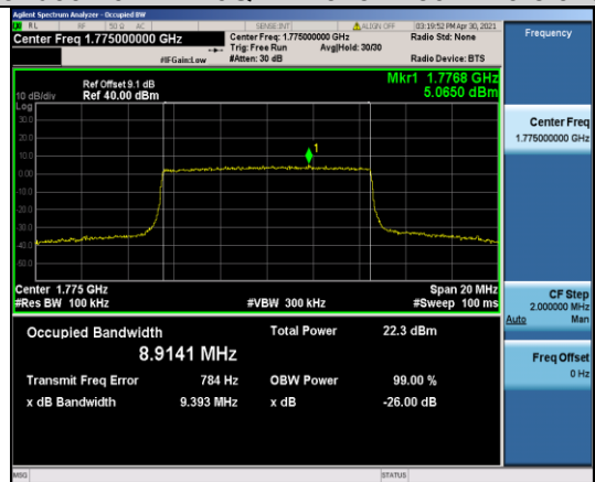
Band66-10MHz-16QAM-132622-50RB#0-8.9141
