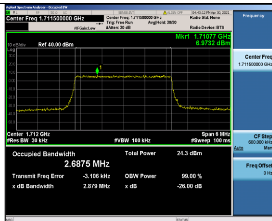
Band66-3MHz-QPSK-131987-15RB#0-2.6875
