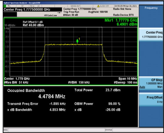
Band66-5MHz-16QAM-132647-25RB#0-4.4784
