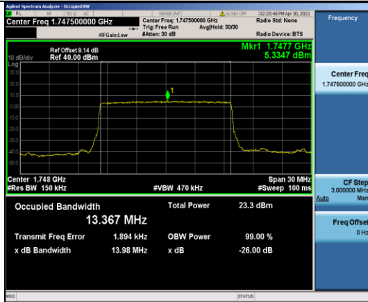
Band4-15MHz-QPSK-20325-75RB#0-13.367
