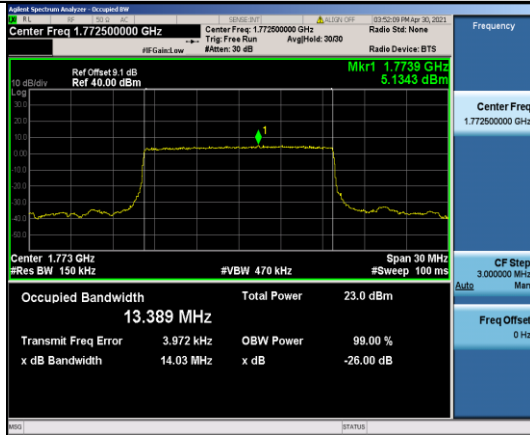
Band66-15MHz-QPSK-132597-75RB#0-13.389
