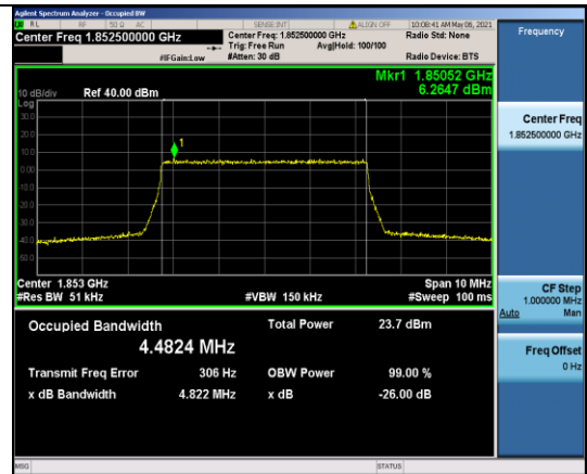
Band2-5MHz-16QAM-18625-25RB#0-4.4824
