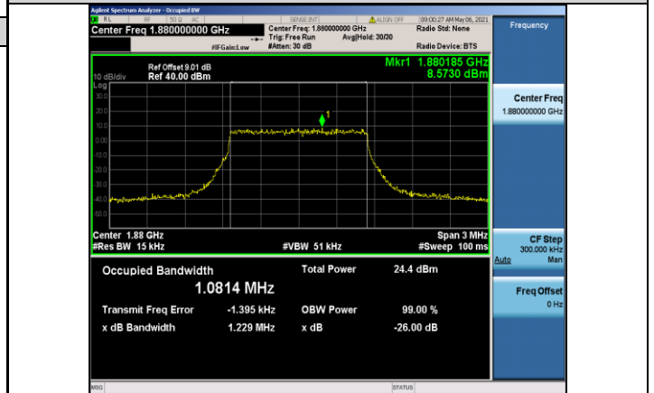
Band2-1.4MHz-16QAM-18900-6RB#0-1.0814
