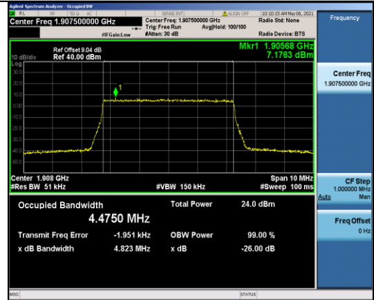
Band2-5MHz-16QAM-19175-25RB#0-4.4750
