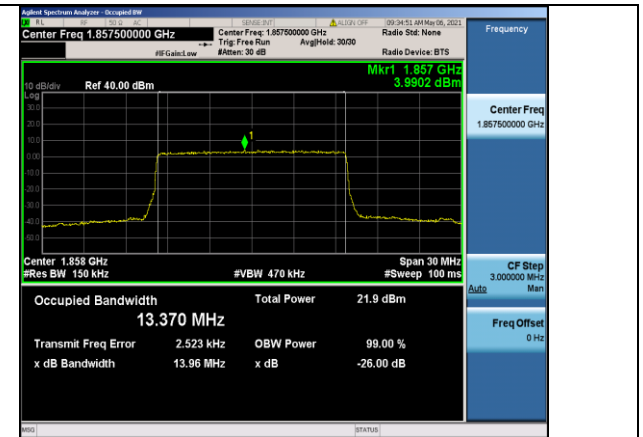
Band2-15MHz-16QAM-18675-75RB#0-13.370
