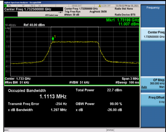
Band4-1.4MHz-16QAM-20175-6RB#0-1.1113
