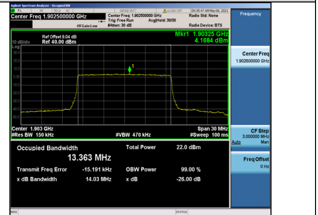
Band2-15MHz-16QAM-19125-75RB#0-13.363
