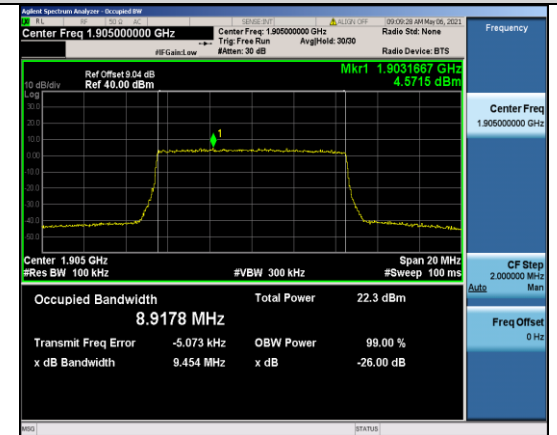
Band2-10MHz-16QAM-19150-50RB#0-8.9178
