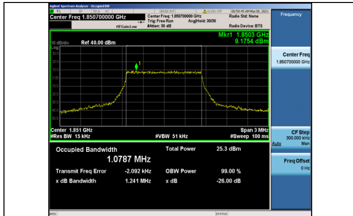
Band2-1.4MHz-QPSK-18607-6RB#0-1.0787
