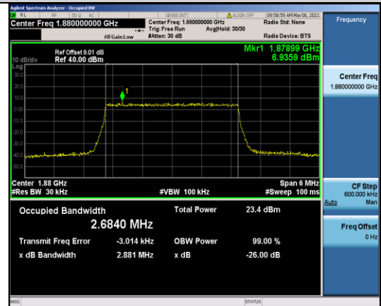
Band2-3MHz-16QAM-18900-15RB#0-2.6840
