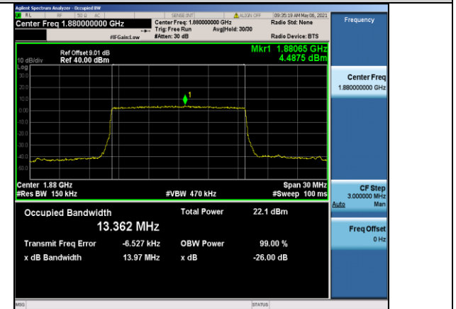
Band2-15MHz-16QAM-18900-75RB#0-13.362
