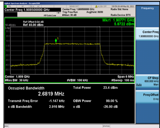
Band2-3MHz-16QAM-19185-15RB#0-2.6819
