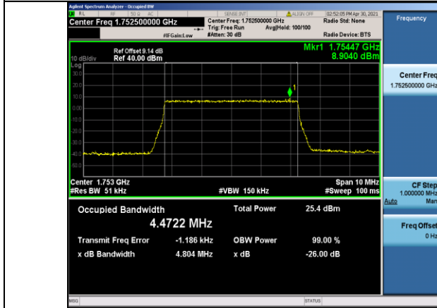
Band4-5MHz-QPSK-20375-25RB#0-4.4722
