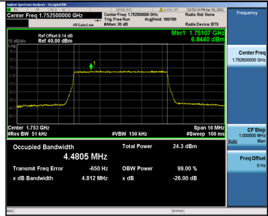
Band4-5MHz-16QAM-20375-25RB#0-4.4805
