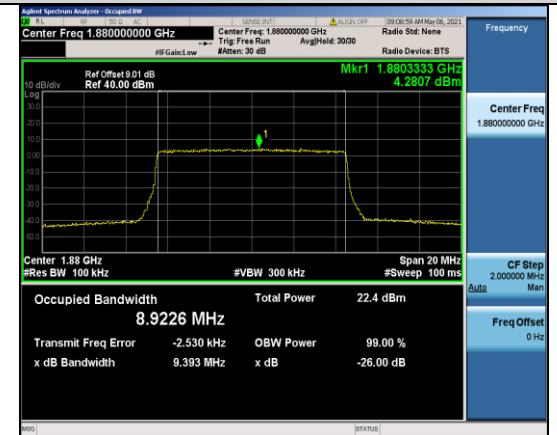
Band2-10MHz-16QAM-18900-50RB#0-8.9226
