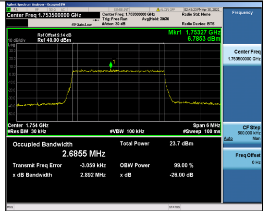
Band4-3MHz-16QAM-20385-15RB#0-2.6855
