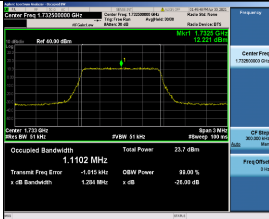
Band4-1.4MHz-QPSK-20175-6RB#0-1.1102
