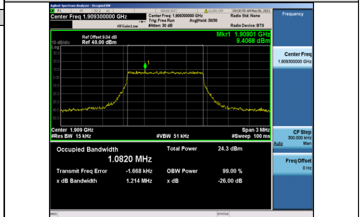
Band2-1.4MHz-16QAM-19193-6RB#0-1.0820
