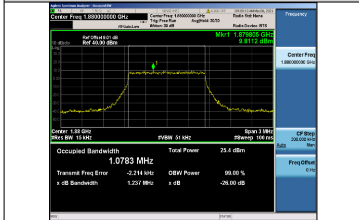
Band2-1.4MHz-QPSK-18900-6RB#0-1.0783
