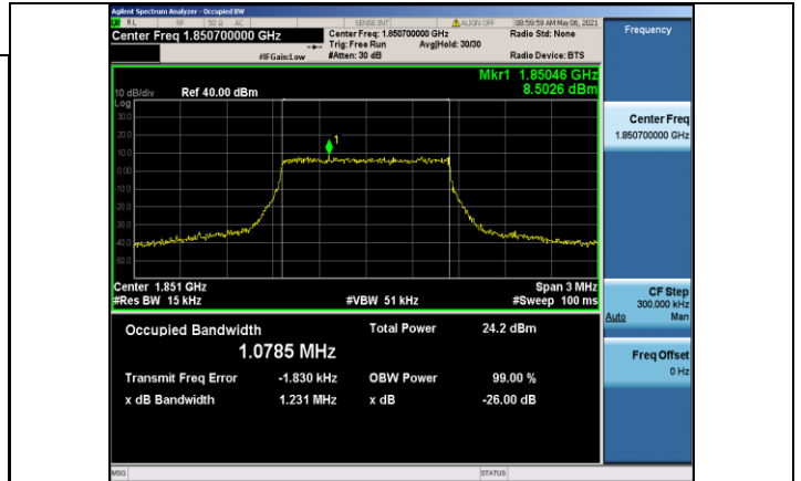
Band2-1.4MHz-16QAM-18607-6RB#0-1.0785
