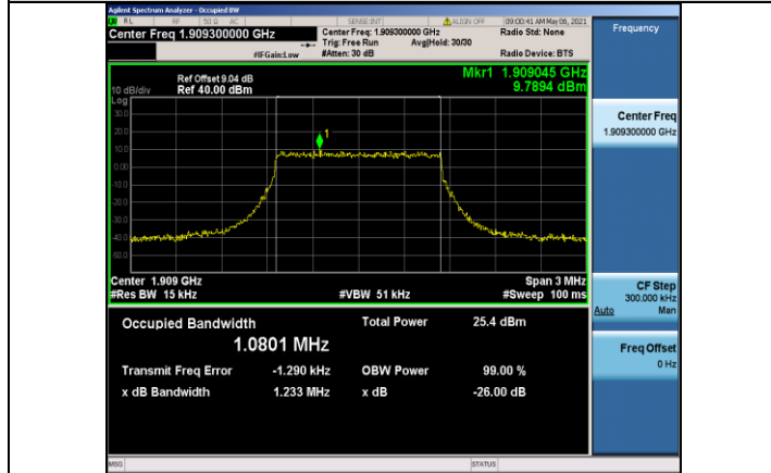
Band2-1.4MHz-QPSK-19193-6RB#0-1.0801
