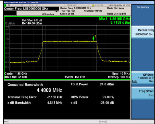
Band2-5MHz-16QAM-18900-25RB#0-4.4809
