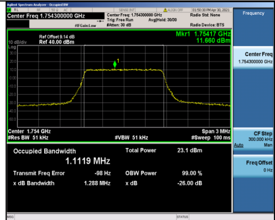
Band4-1.4MHz-16QAM-20393-6RB#0-1.1119
