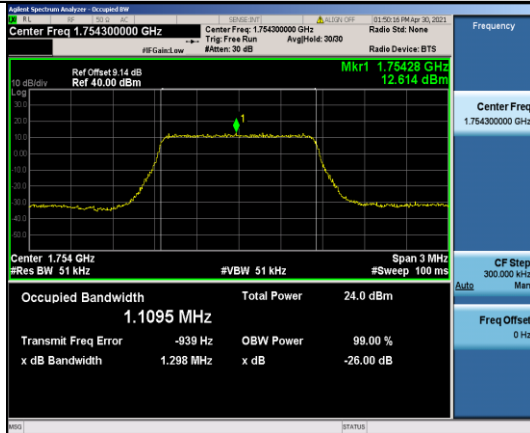
Band4-1.4MHz-QPSK-20393-6RB#0-1.1095
